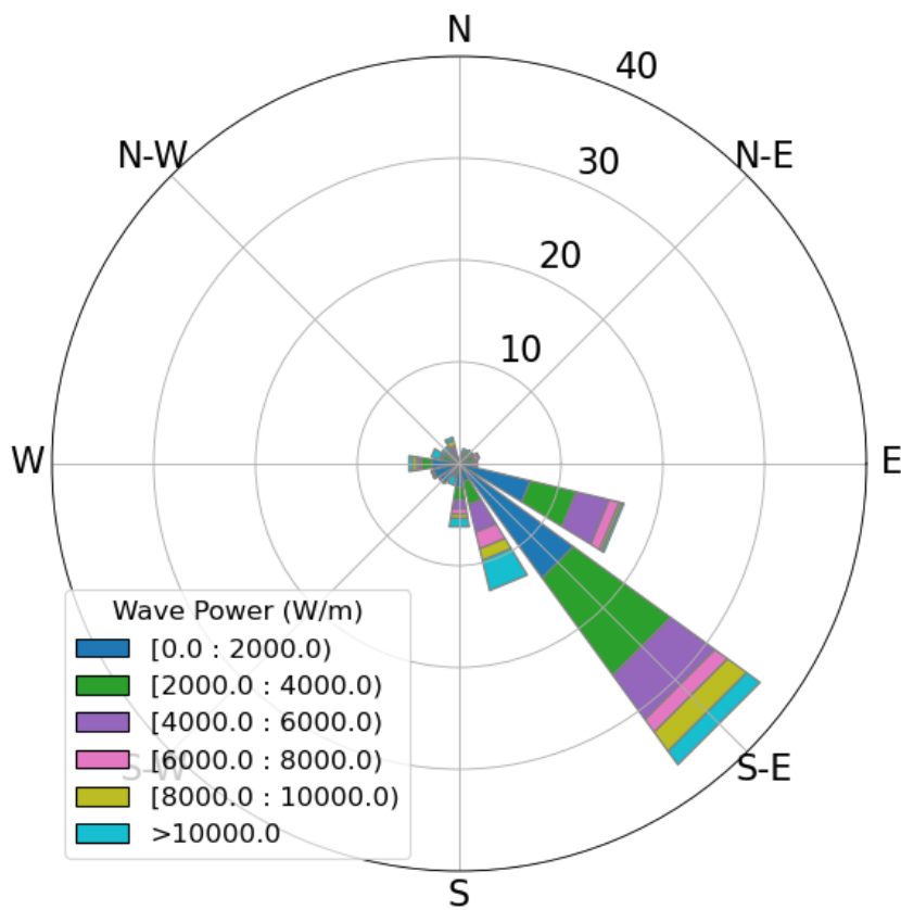
455 Figure 12: Rose diagram of wave power at 28.8°N, 276.4°E in the Gulf of Mexico. The length of each bar and the concentric circles indicate the percentage of datapoints with waves coming from that direction (meteorological convention). The color indicates the wave power.
