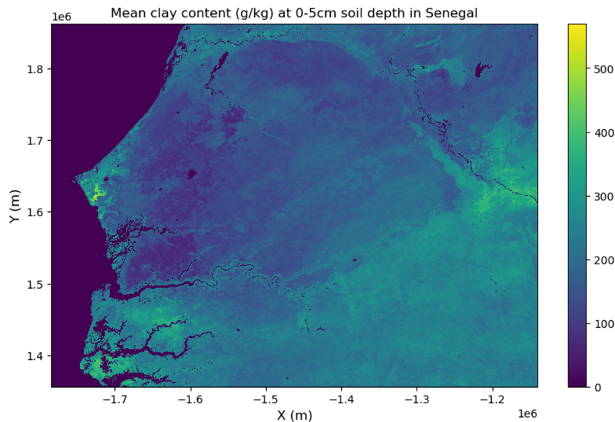
Figure 2: Example scripts that use the API (a) and the pynt component (b) of the SoilGrids Data Component to access and visualize the soil property dataset (c).
