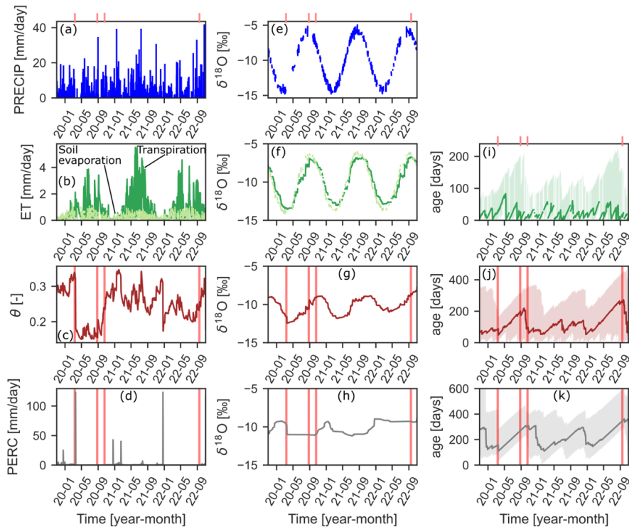
Figure 6 Simulated fluxes and soil water content (a-d), corresponding \delta^{18}\text{O} signal (e-h) and corresponding 10 th , 50 th and 10 th percentile of water ages (i-k) of a single grid cell. Vertical red lines indicate the four different dates from Figure 6. Power law distribution function serves as SAS function (SAS parameters: k_{\text{evap-soil}}=0.2 , k_{\text{transp}}=0.5 , k_{\text{perc-rz}}=1.5 , k_{\text{perc-ss}}=1.5 ; see Figure 2)
