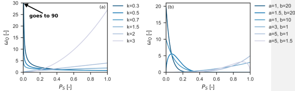
Figure 2 Storage selection with different parameters illustrated for power law distribution function (a; see Eq. (1)) and Kumaraswamy distribution function (b; see Eq. (3))
