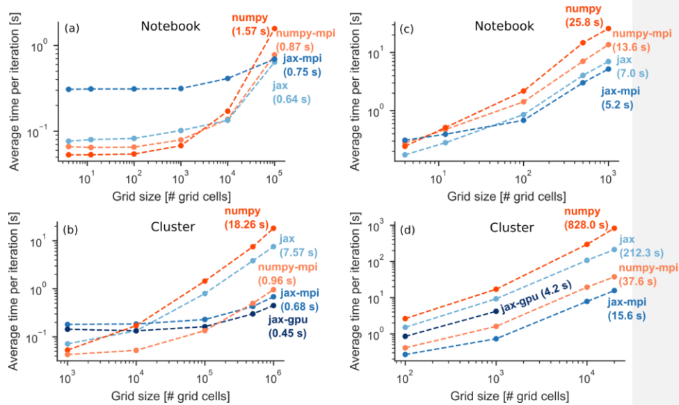
300 Figure 3 Runtime performance of computational back-ends for the RoGeR-SVAT type model (a, b) and for the RoGeR-SVAT- 18 O type transport model (c, d). Note that, the number of grid cells represents the two horizontal spatial dimensions (e.g. longitudes and latitudes). The total number of elements is greater for transport models due to additional age dimensions and can be derived by multiplying the number of grid cells (i.e. two spatial dimensions) with the number of water ages (e.g. 1500). SVAT model used 100 iterations and SVAT- 18 O transport model used 20 iterations.
