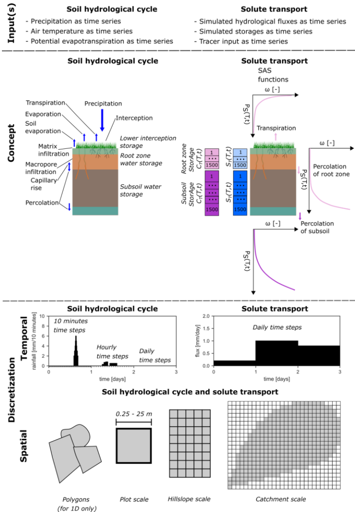
210 Figure 1 Overview of model inputs, conceptual implementation shown for a single grid cell or unit (Water storages are represented in italics ), and temporal discretization of the soil hydrologic cycle and solute transport. Spatial discretization for different scales is the same for the soil hydrologic cycle and solute transport.
