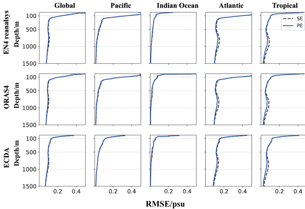
Figure 8. The same with Figure 6 but for salinity RMSE.
