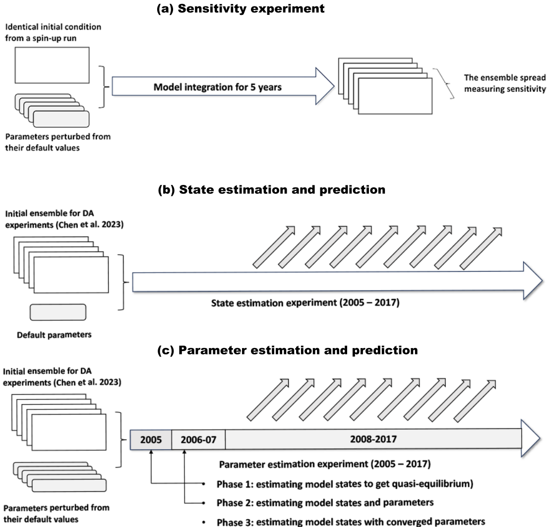
Figure 2. The schematic diagrams of (a) the sensitivity experiment , (b) state estimation and prediction experiment, (c) parameter estimation and prediction experiment.
