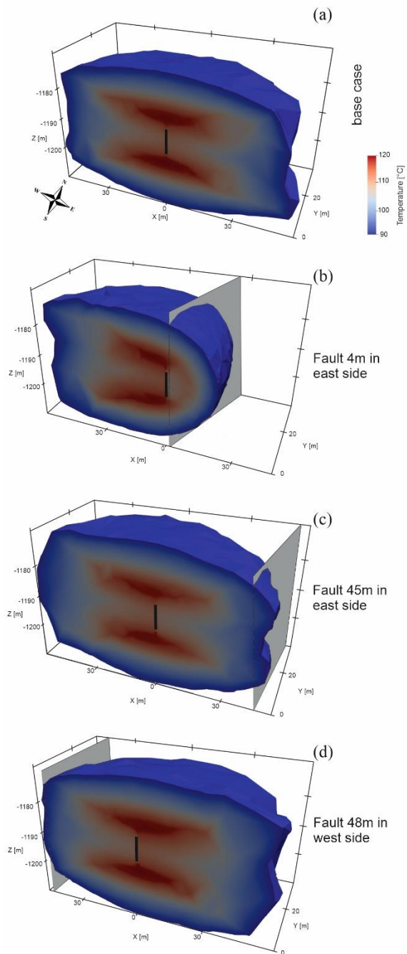
380 Figure 8: Heat accumulation in four different scenarios of the DeepStor model at the end of the last production cycle. The planned well is shown as a solid black line. Subplots from a to d represent different scenarios including base case, arbitrary fault (shown with a grey surface) in 4 and 45 m in the east of the well and 48 m in the west. The temperature scale is also the same and shown only once in subplot a to avoid repetition.
