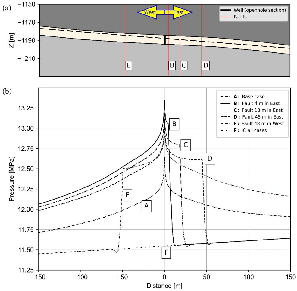
405 Figure 9: Total pressure increase of five simulated cases at the end of the first injection cycle. The cross section in subplot a indicates the position of the traces used for plotting the pressure data of five different scenarios and the initial condition (IC). Negative values for distance represent the western side of the well. To make the curves more readable, scenarios are labelled as A, B, C, D, E, and the initial condition as F.
