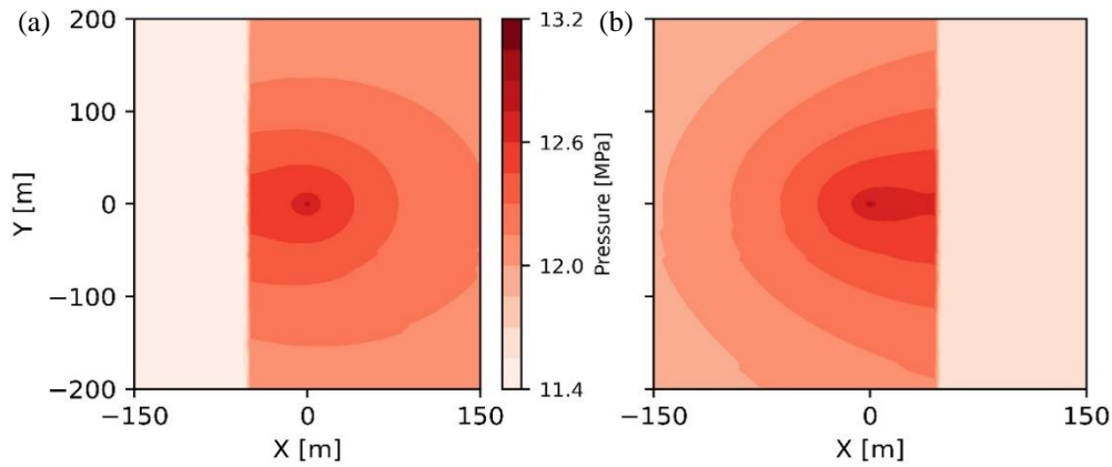
Figure 11: Total pressure changes after the first injection cycle in two scenarios. The well position is in the center of both plots (coordinates=0.0 and 0.0). The fault location is easily distinguishable by the sharp change in the pressure data: 48 m in the west of well (a) and 45 m in the east (b). Negative and positive values for the x and y axis are relative to the position of the well.
