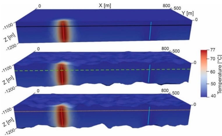
345 Figure 5: Heat distribution after 10 years of storage in the Malm limestone reservoir of the GGB. Red and blue lines represent hot and cold wells, respectively. The upper scenario with a uniform box shaped reservoir is considered as the base case while contacts of the reservoir in the middle and lower scenarios are perturbed. Solid black, dashed green and dotted orange traces are used in Figure 6 for plotting the temperature values.
