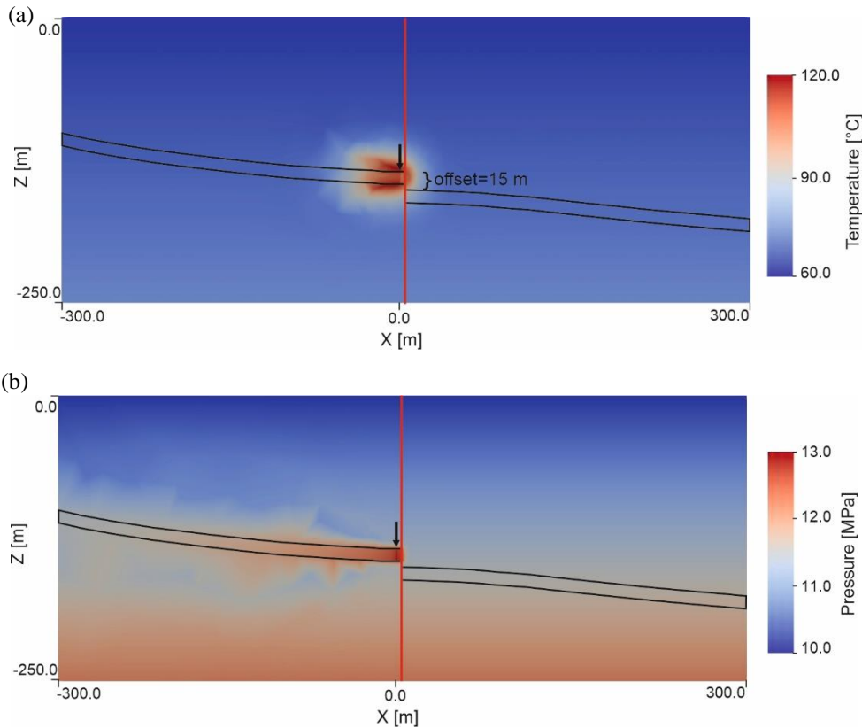
410 Figure 10: a) Temperature changes in a cross section of the DeepStor model at the end of the last production cycle. b) Pressure regime in the model after the first injection cycle (6 months). In both subplots location of the well is highlighted by a black arrow in the middle of the model. The fault is represented as a continuous thick red line which locates 4 m in the east of the well and has a fixed 15 m offset. The thick black line also represents the boundaries of the reservoir layer.
