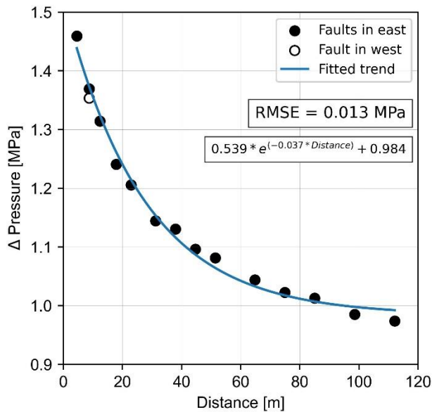
515 Figure 14: Difference between the well pressure on day five of injection and initial condition ( \Delta Pressure) versus the distance of the arbitrary fault to the well. The continuous line represents an exponential function with three degrees of freedom.
