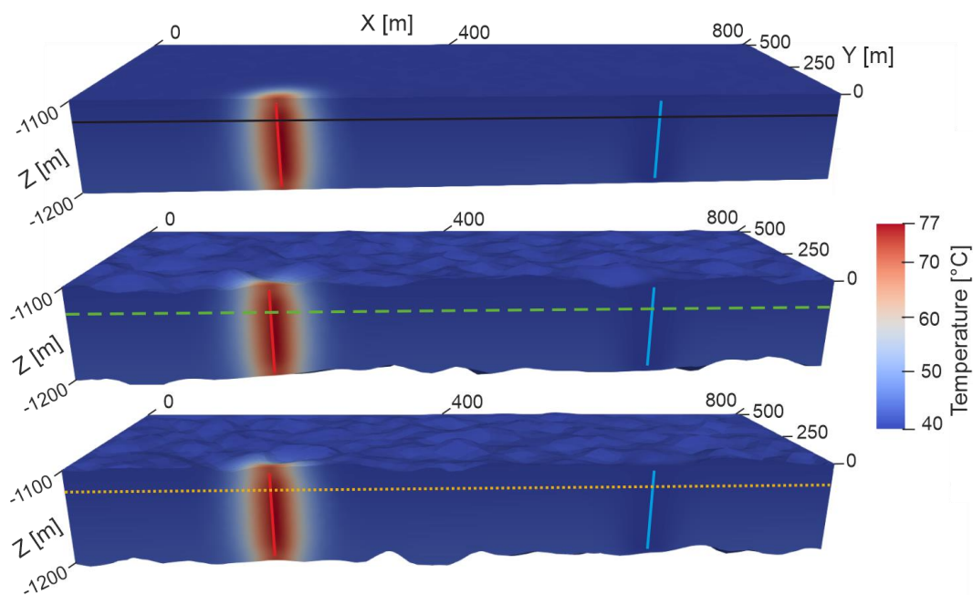
260 Figure 4: Heat distribution after 10 years of storage in the Malm limestone reservoir of the GBB. Red and blue lines represent warm and cold wells, respectively. The upper scenario with a uniform box shaped reservoir is considered as the base case while contacts of the reservoir in the middle and lower scenarios are perturbed and irregular. Solid black, dashed green and dotted orange traces are used in Figure 5 for plotting the temperature values.
