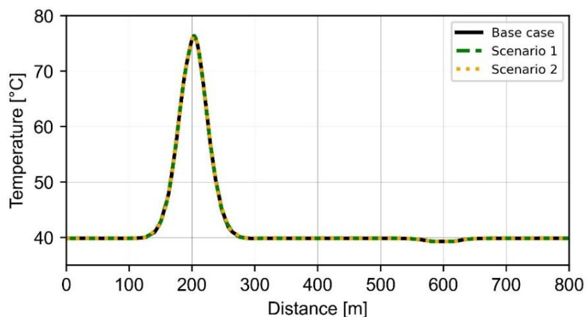
265 Figure 5: Temperature distribution curves of the values coming from the base case and two perturbed scenarios after 10 years of injection and production for the GBB. Warm and cold wells are located at 200 m and 600 m points of the x axis. To find the location of the plotted trace, refer to Figure 4. Similar to the models' extension in x direction x axis i.e. Distance (in m) ranges from 0 m to 800 m.
