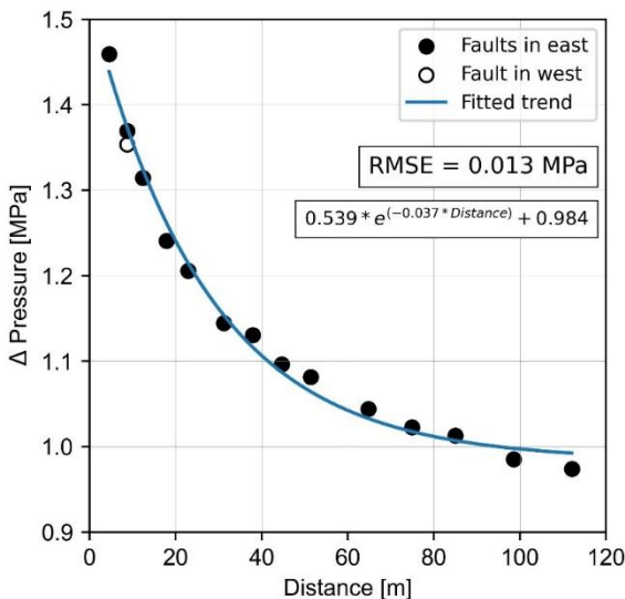
410 Figure 11: Difference between borehole pressure on day five of injection and initial condition ( \Delta Pressure) versus the distance of the arbitrary fault to borehole. The continuous line is representing an exponential function with three degrees of freedom.
