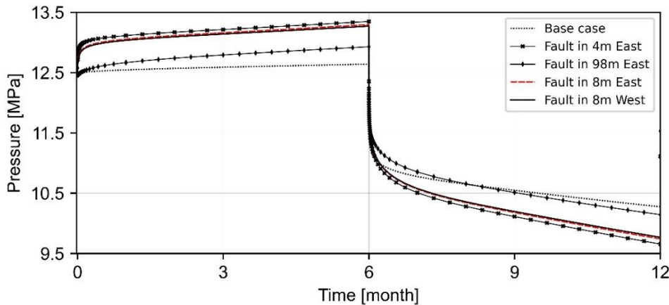
405 Figure 10: Total pressure evolution in the well during the first injection and production phase. Only five cases are plotted to keep the figure readable. Higher pressure accumulation in the east of the well can be observed by the slight difference between dashed red (Fault in 8m East) and black (Fault in 8m West) curves.
