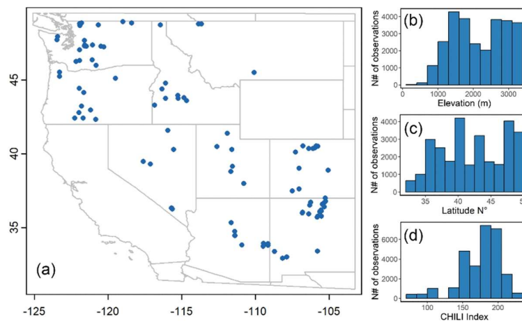
Figure 2. Location of SNOTEL stations used for training the SVR (a), and their density distributions in terms of (b) elevation, (c) latitude, and (d) heat-insolation index. 150
