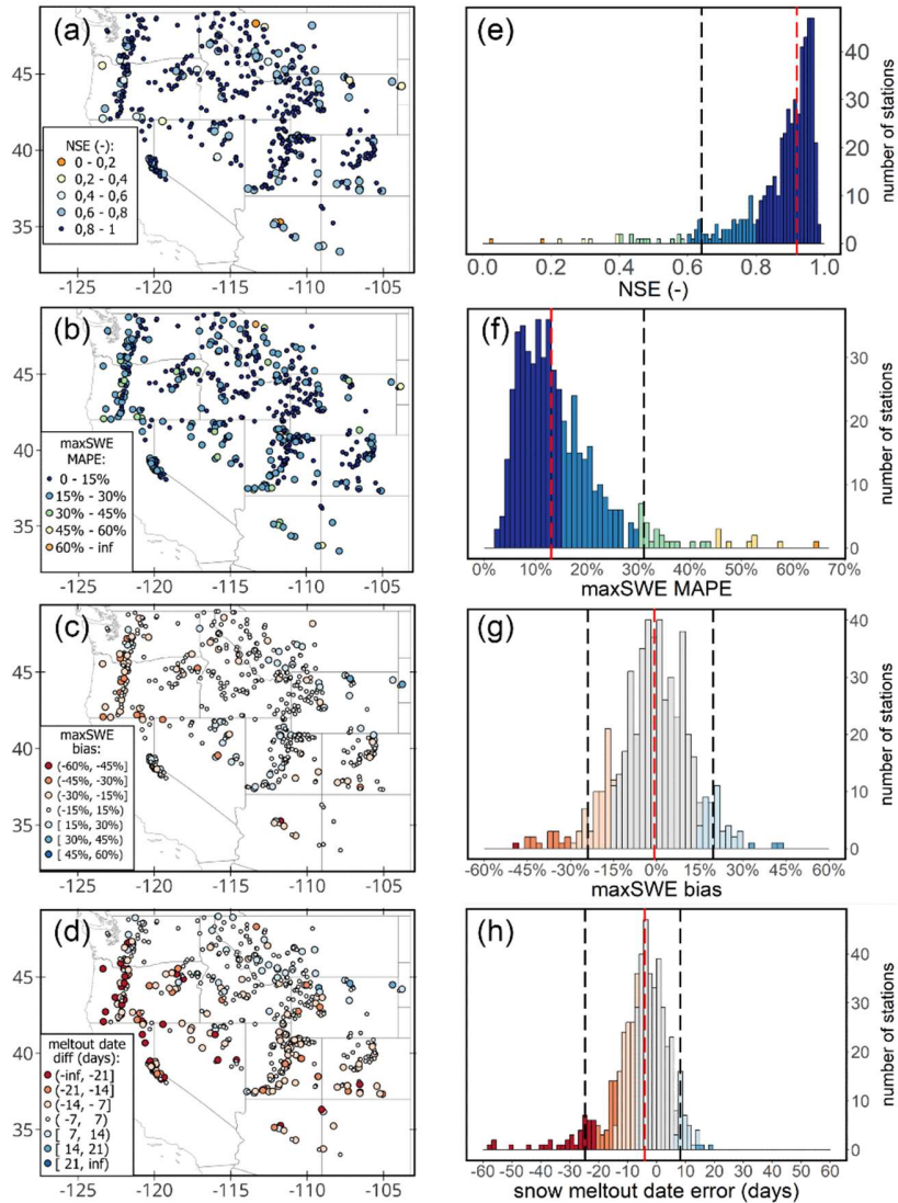
285 Figure 6. GEMS performance metrics for independent SNOTEL stations: spatial distributions of the resultant (a) NSE, (b) 290 maxSWE MAPE, (c) maxSWE bias, (d) snow meltout date error, and corresponding histograms (e-h). Vertical red dashed lines on the histograms denote the median across all stations; the vertical black dashed line correspond to the 5 th percentile (and 95 th percentile in case of two-tailed distributions).
