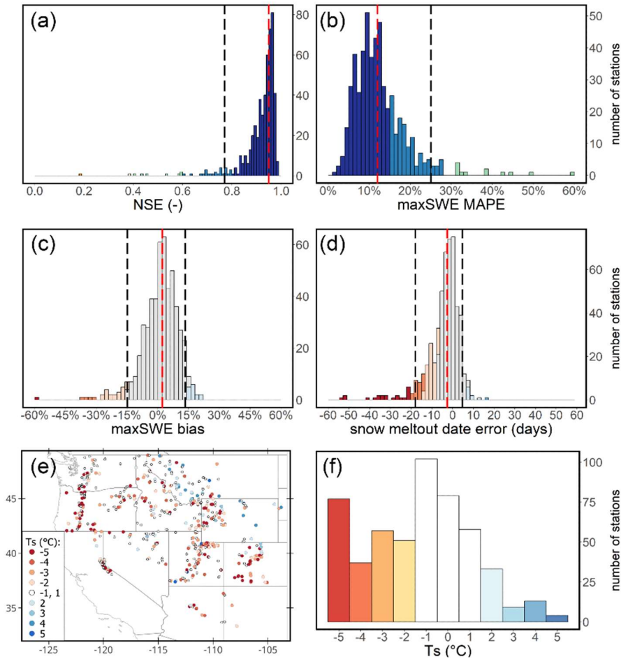
Figure 7. GEMS performance metrics for the independent SNOTEL stations with station-adjusted T_s threshold: (a) NSE, (b) maxSWE MAPE, (c) maxSWE bias, (d) snow meltout date error. The bottom map (e) and histogram (f) show density and spatial distribution of the adjusted T_s values.
