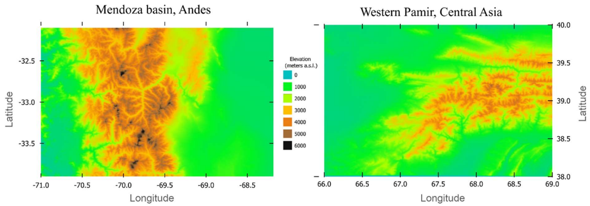
200 Figure 3. Selected regions for distributed snow modelling
