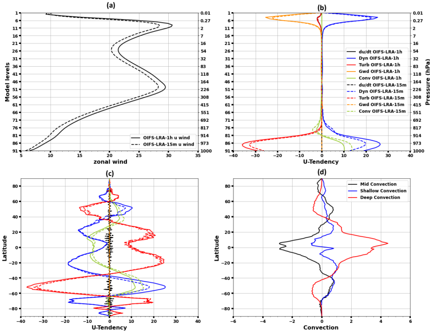
622 Figure 3. (a) Averaged zonal wind ( u ) [ \text{ms}^{-1} ] and zonal wind tendencies [ \text{ms}^{-2}/\text{hour} ] over the Southern Ocean ( 40^{\circ}\text{S} - 60^{\circ}\text{S} , 623 all longitude) as a function of height for OIFS-LRA-1h and OIFS-LRA-15m. Model levels (y-axis left) and pressure levels (y- 624 axis right). (c) Zonal and time average of zonal wind tendencies at the lowest level of the model as a function of latitude. (d) 625 Zonal and time average convection difference [ \text{Kgm}^{-2}/\text{hour} ] between OIFS-LRA-15m and OIFS-LRA-1h configurations. The 626 solid lines in panels (b) and (c) show the wind tendency for OIFS-LRA-1h configuration whereas the dashed lines are for 627 OIFS-LRA-15m configuration. Shown are averages over 1979-2019.
