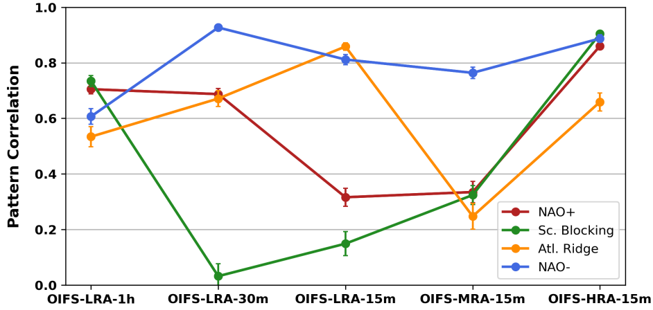
653 Figure 8. Pattern correlation coefficient of the individual weather regime between OIFS model configurations and ERA5 for 654 the period 1979-2019 for the DJF season. The error bars represent a 95% confidence interval.
