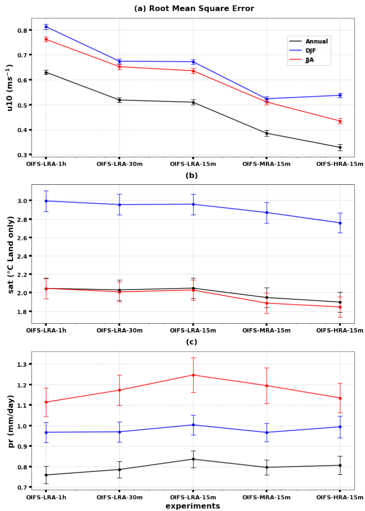
616 617 Figure 2. Root mean squared error of surface zonal wind (a), SAT (b), and precipitation (c) over the period 1979-2019 for all 618 the configurations: annual (black) and seasonal mean (DJF: blue, JJA: red). The error bars represent a 95% confidence interval.
