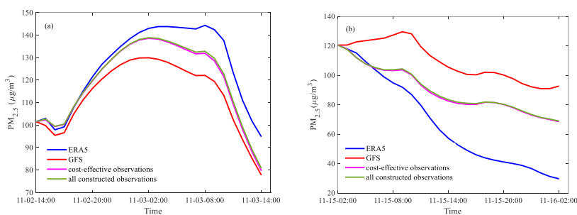
Figure 8 Time series of the PM_{2.5} concentrations averaged over the BTH region of the truth run, the control run, and the assimilation run inherited from the cost-effective observations and all the constructed observations for the AF initialized by 14:00 on 2 November 2018 with lead time of 24 hours (a) and the DF 625 started from 02:00 on 15 November 2018 with lead time of 24 hours (b).
