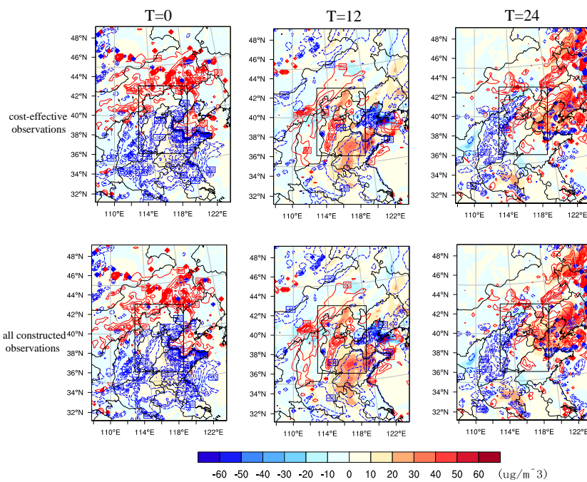
635 Figure 10 The differences of the boundary layer height (contour line, m, blue line means reduction and red line means increase) and the \text{PM}_{2.5} concentrations (shaded, \mu\text{g m}^{-3} ) between the assimilation run inherited from the cost-effective observations and constructed observations and the control run for the AF started from 14:00 on 2 November 2018 and with the lead times of 12h and 24h.
