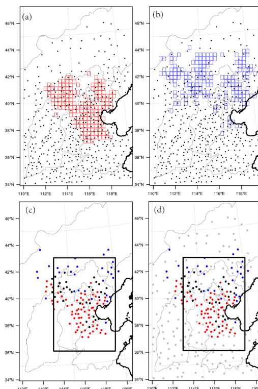
Figure 6 The spatial distributions of the 174 sensitive grid points (red squares) for AFs (a), the 184 sensitive grid points (blue squares) for DFs (b), and all constructed stations [denoted by black dots in (a) and (b)]; and a contrasting between the essential stations for AFs (red dots) and those for DFs (blue dots) (c), where the thick black dots present their overlapped stations. (d) shows the cost-effective stations network including the essential stations (blue, red, and black dots) as in (c) and the additional scattered stations (gray dots). 420
