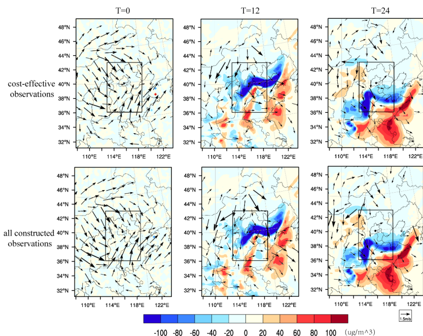
670 Figure 11 The differences of ground wind (vector, \text{m s}^{-1} ) and \text{PM}_{2.5} concentrations (shaded, \mu\text{g m}^{-3} ) between the assimilation run (inherited from the cost-effective observations and all constructed stations observations) and the control run for the DF started from 02:00 on 15 November 2018 and with the lead times of 12h and 24 h.
