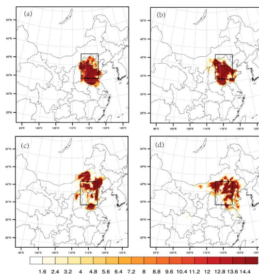
Figure 5 The horizontal distribution of the TME (unit: \text{J kg}^{-1} ) for the AFs started from (a) 02:00 on Nov 2 and (b) 14:00 on Nov 2 in 2018, and for the DFs started from (c) 02:00 on Nov 4 and (d) 14:00 on Nov 4 in 2018. The black rectangle is the verification area, i.e. the BTH region.
