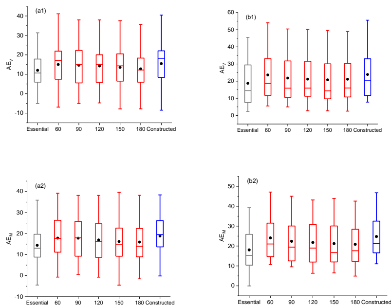
Figure 7 The boxplot of the (1) AE_V and (2) AE_M values when assimilating the essential station observations, the essential observations plus the scattered station observations with the distances 60, 90, 120, 150 and 180km, and all constructed station observations for (a) AFs and (b) DFs.
