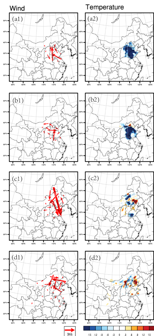
Figure 4 The horizontal distribution of the wind (1) and temperature (2) components of the CNOP-type errors for the AF started from the 02:00 on Nov 2 (a) and from 14:00 on Nov 2 in 2018 (b), and for the DF started from 02:00 on Nov 4 (c) and from 14:00 on Nov 4 in 2018 (d).
