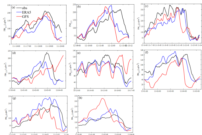
Figure 2 Time series of the PM_{2.5} concentrations averaged over the BTH region of observations (black line) and simulations initialized by ERA5 (blue line) and GFS (red line) meteorological data during the eight heavy hazy events in 2016–2018. These events occurred during (a) 12:00BJT, 15 Nov-02:00 BJT, 20 Nov in 2016; (b) 00:00 BJT, 9 Dec-12:00 BJT, 13 Dec in 2016; (c) 00:00 BJT, 16 Dec-00:00 BJT, 23 Dec in 2016; (d) 00:00 BJT, 30 Nov-00:00 BJT, 4 Dec in 2017; (e) 00:00 BJT, 13 Oct-00:00 BJT, 17 Oct in 2018; (f) 00:00 BJT, 1 Nov-00:00 235 BJT, 5 Nov in 2018; (g) 00:00 BJT, 11 Nov-00:00 BJT, 16 Nov in 2018; (h) 00:00 BJT, 30 Nov-00:00 BJT, 4 Dec in 2018.
