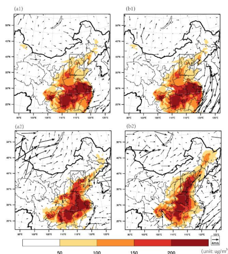
240 Figure 3 The surface wind (vector, \text{m s}^{-1} ) and \text{PM}_{2.5} concentration (shaded; \mu\text{g m}^{-3} ) components of the initial states for the simulation of the event during 30 November and 4 December in 2018 (1) and their evolutions at the lead time 18 hours (2), where the initial time is 00:00 30 November 2018 and (a) is initialized by the ERA5 and (b) is initialized by the GFS.
