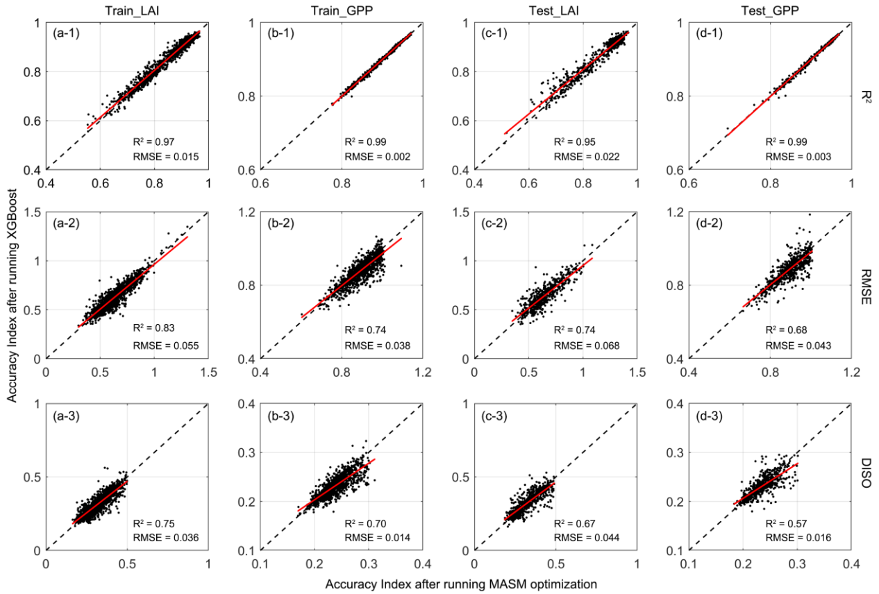
800 Figure 6. Accuracy indexes ( R^2 , RMSE, and DISO) validation between trained and predicted parameters in simulating LAI and GPP. The X-axis represents the accuracy index using MASM posterior parameters; The Y-axis represents the accuracy index using estimated parameters from the trained XGBoost model.
