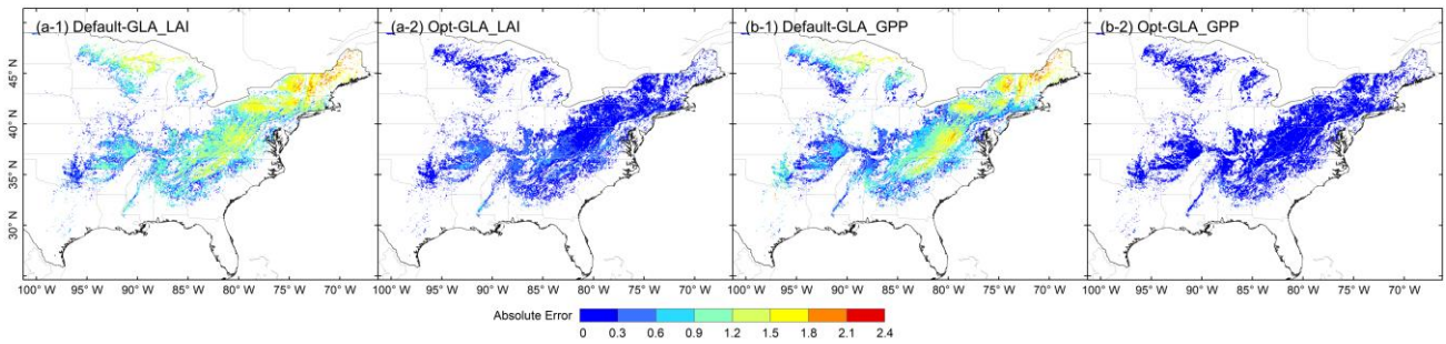
810 Figure 9. Spatial distribution of annual absolute error between model results and GLASS products from 2001 to 2018.: (a-1) and (a-2) are the absolute difference of prior and posterior LAI, respectively; (b-1) and (b-2) are the absolute difference of prior and posterior GPP, respectively.
