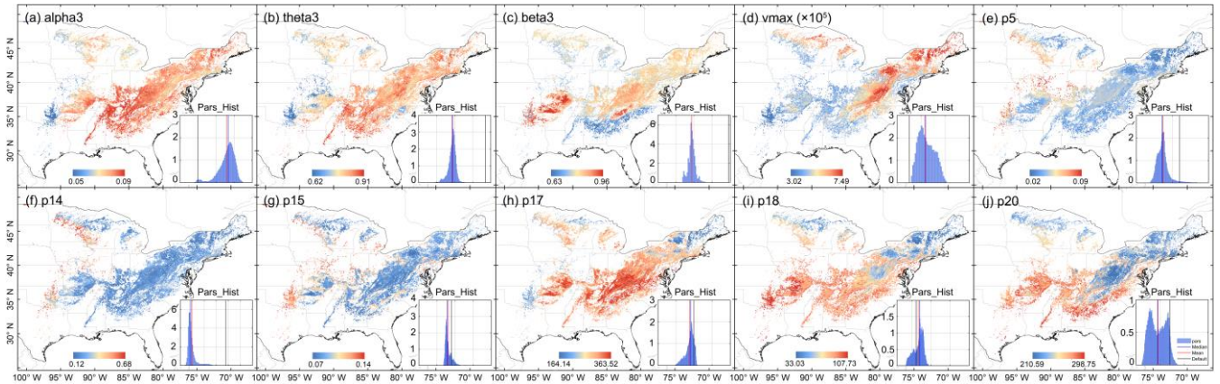
805 Figure 7. Spatial distribution of posterior parameter. The inset in the lower right corner of each plot represents the spatial distribution histogram of each parameter
