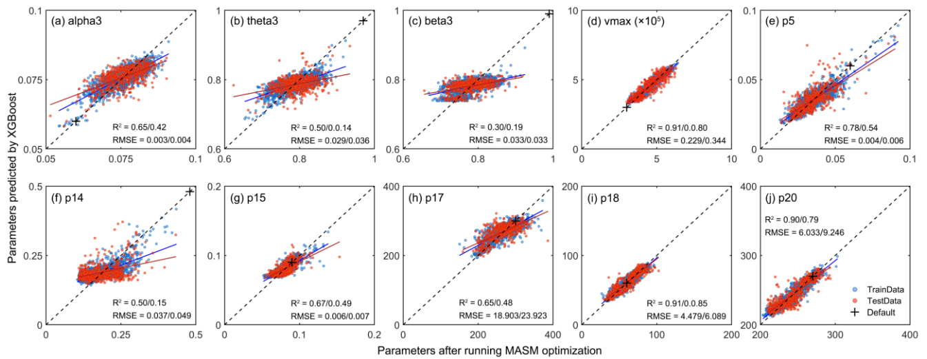
795 Figure 5. Scatter plots of the results of the XGBoost model. The X-axis represents parameters after running MASM optimization, Y-axis means values obtained from XGBoost model. The means before and after the slash represent the accuracy indexes of the training set and testing sets, respectively. The blue dots represent the training set, and red dots represent the testing set. The black cross indicates default values.
