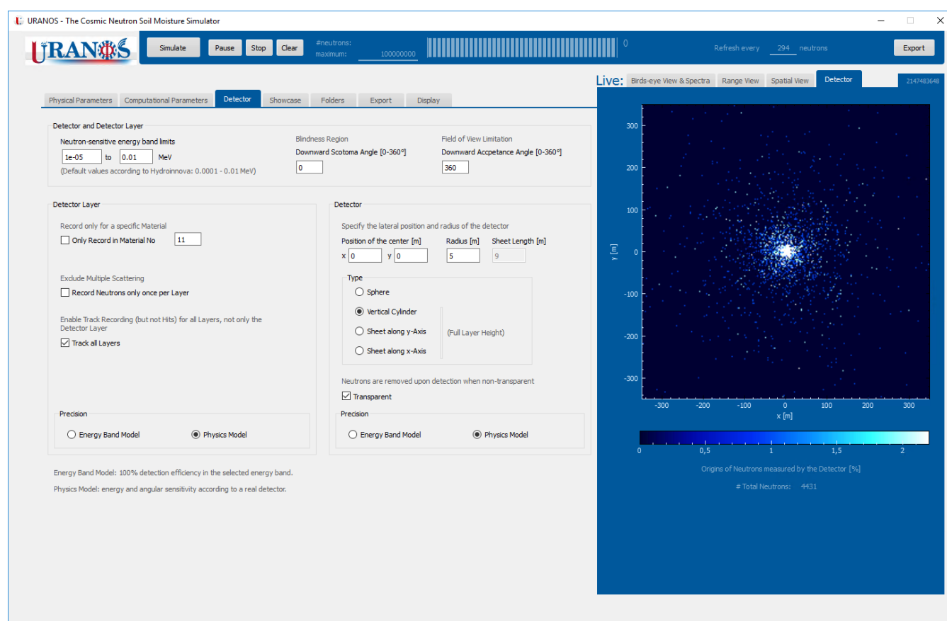
Figure 17. URANOS user interface showing the detector tabs. (left) Settings for changing energy and and angular sensitivity as well as geometric shape and extension. (right) Detector scoring output showing the origins of detected neutrons
