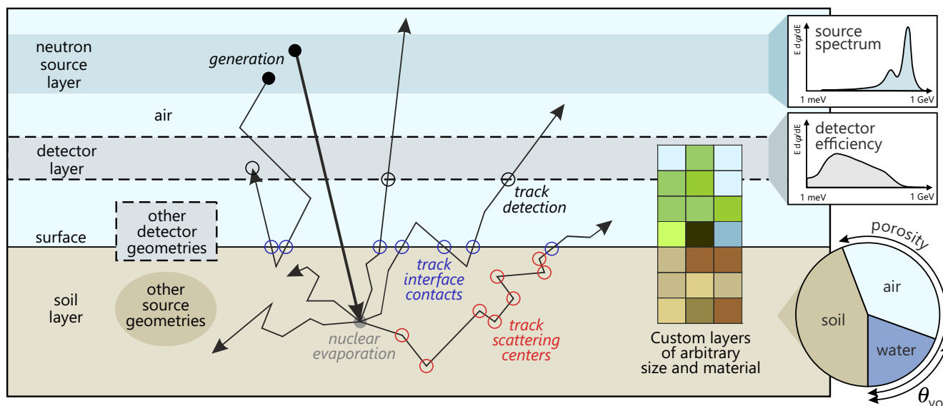
Figure 1. Two-dimensional projection of the 3D model setup and processes. Neutrons are generated in a source layer following a source spectrum that resembles the energy distribution of particles propagated through the air column above. High-energy neutrons create fast neutrons by nuclear evaporation in the soil. They further scatter through the material layers until they eventually reach the detector layer which absorbs the neutrons depending on the chosen detector response function. While the soil is modeled as a combination of silicate, air, and water, various other components of the environment can be modeled with the available material and density options.
