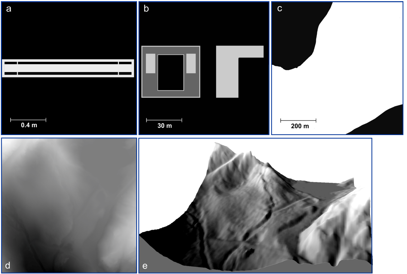
Figure 4. Examples of layers for voxel geometry definitions (all in top view) with grayscale values defining preconfigured materials: a) a 2 nd proportional counter with 1 st of moderator, b) the rooftop of the institute of physics in Heidelberg, c) a part of a lake (Schrön, 2017), d) voxel geometry for a digital environmental model (Kaunertal Glacier at N46° 52.2 E10° 42.6) with 500 × 500 pixels at a lateral resolution of 1 m and 0.5 m in height, e) shaded illustration of the resulting layered voxel structure from d).
