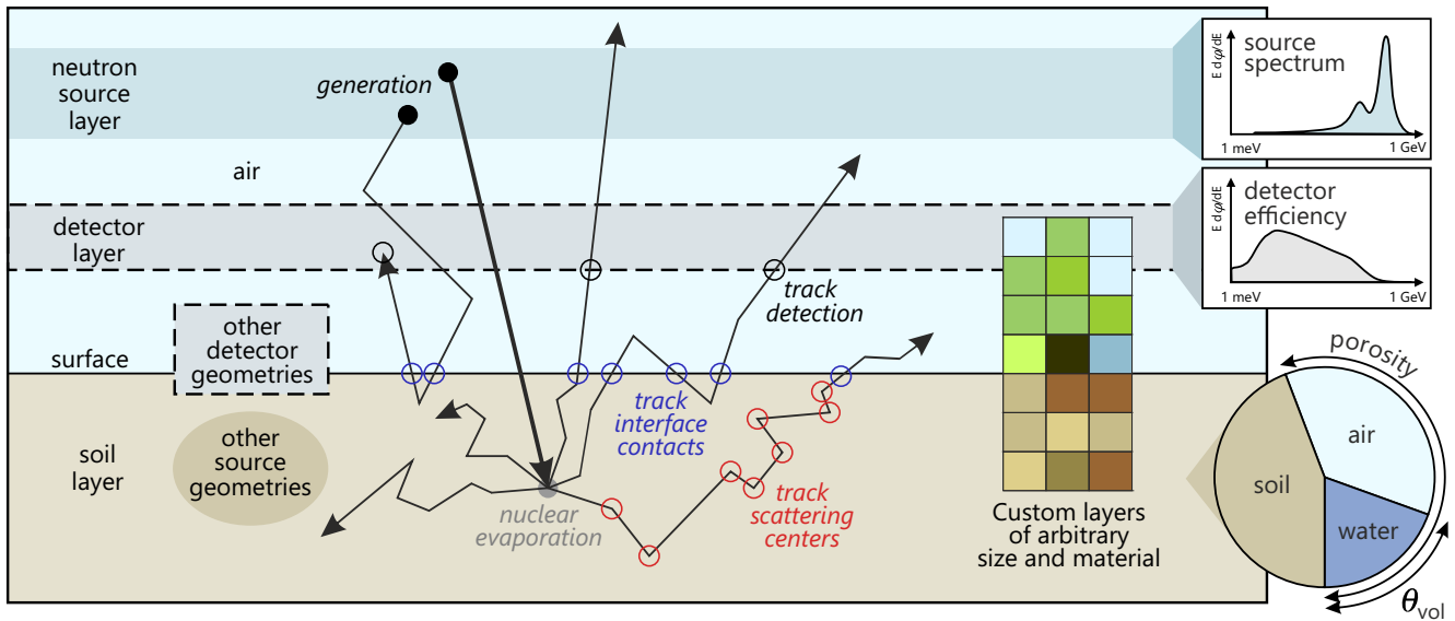
Figure 1. Two-dimensional projection-representation of the 3D model setup ( not to scale ) and processes. Neutrons are generated in a source layer ( black filled circle • ) following a source spectrum that resembles the energy distribution of particles propagated through the air column above. High-energy neutrons create fast neutrons by nuclear evaporation in the soil ( gray filled circle • ). They further scatter within (red empty circle ◦) or through the material layers ( blue empty circle ◦ ) until they eventually reach the detector layer ( gray empty circle ◦ ) which absorbs the neutrons depending on the chosen detector response function. While the soil is modeled as a combination of silicate, air, and water, various other components of the environment can be modeled with the available material and density options.
