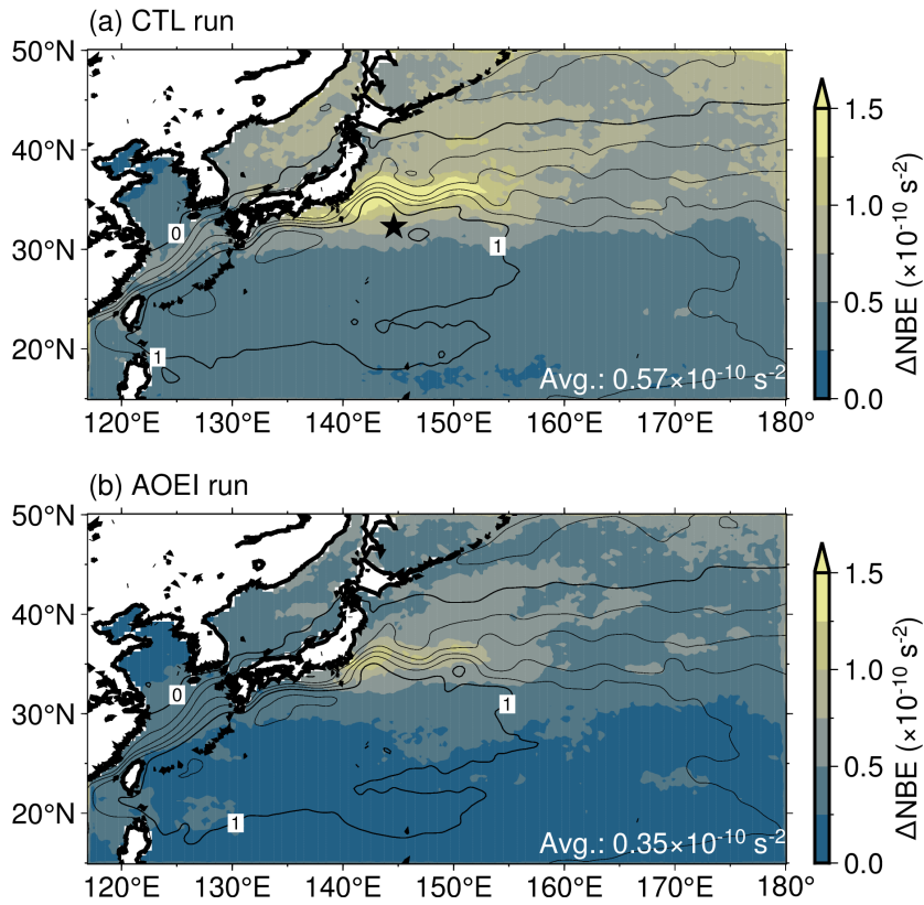
750 Figure 11: \Delta NBE (color) and SSH (contour) averaged over the whole experiment period for the (a) CTL and (b) AOEI runs. Thin (thick) contour intervals are 0.2 (1) m. Spatiotemporally averaged \Delta NBE over the whole period and domain is shown in the lower right corners. The black star in (a) denotes the position of the KEO buoy.
