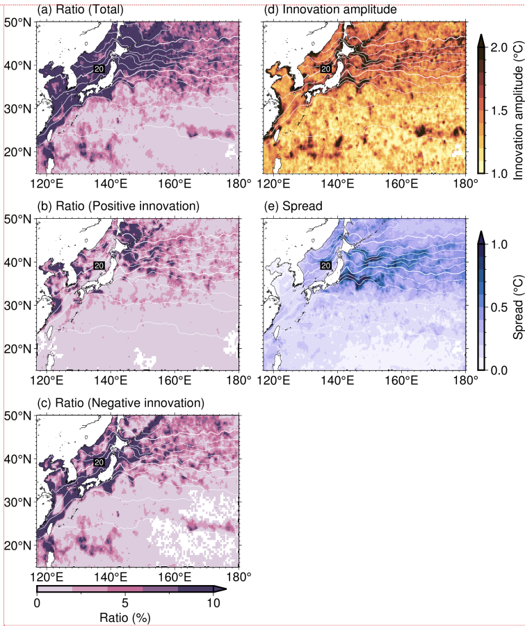
Figure 5: (a) Ratio of the period when the AOEI is applied to the SST compared with the whole experiment period in the AOEI run. (b) and (c) Same as (a) but for when the innovation is positive and negative, respectively. (d) and (e) innovation amplitude and ensemble spread averaged during the period when the AOEI is applied, respectively. White contours indicate SST averaged over the whole period. Thin (thick) contour intervals are 2 (10) °C. White areas indicate no AOEI application.
