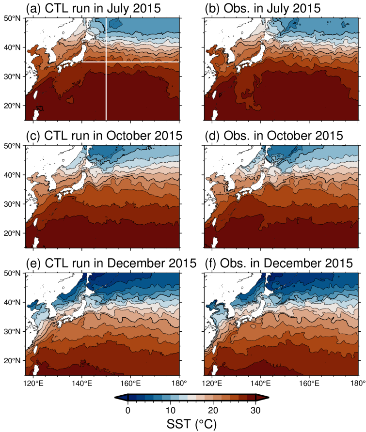
685 Figure 1: Monthly-mean SST s for (a) July, (c) October, and (e) December 2015 in the CTL run. (b), (d), and (f) Same as (a), (c), and (e), but for assimilated satellite SSTs. Thin (thick) black contour intervals are 2 (10) °C. White lines in (a) indicate 150°E (35°N) used for the zonal (meridional) sections in Fig. 3.
