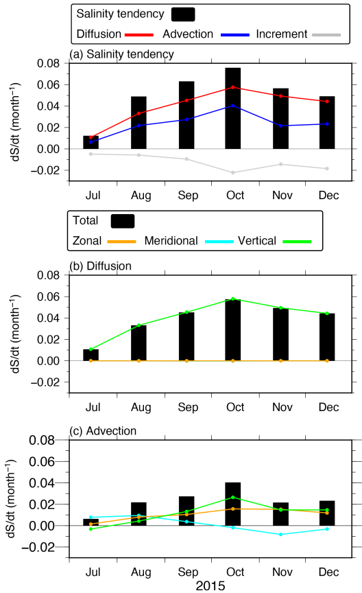
765 Figure A1: (a) Monthly mean for each term in the salinity budget equation [Eq. (5)] averaged over the KE region in the intermediate layer (140°–160°E, 30°–40°N, and 500–1000 m depth) in the CTL run: the salinity tendency term (the LHS term; black bars), salinity diffusion term (the first term on the RHS; red line), salinity advection term (the second term on the RHS, blue line), and salinity analysis increment term (the last term on the RHS; gray line). (b) and (c) Same as (a), but for salinity diffusion and advection terms (black bars), and zonal (orange lines), meridional (cyan lines), and vertical (green lines) components.
