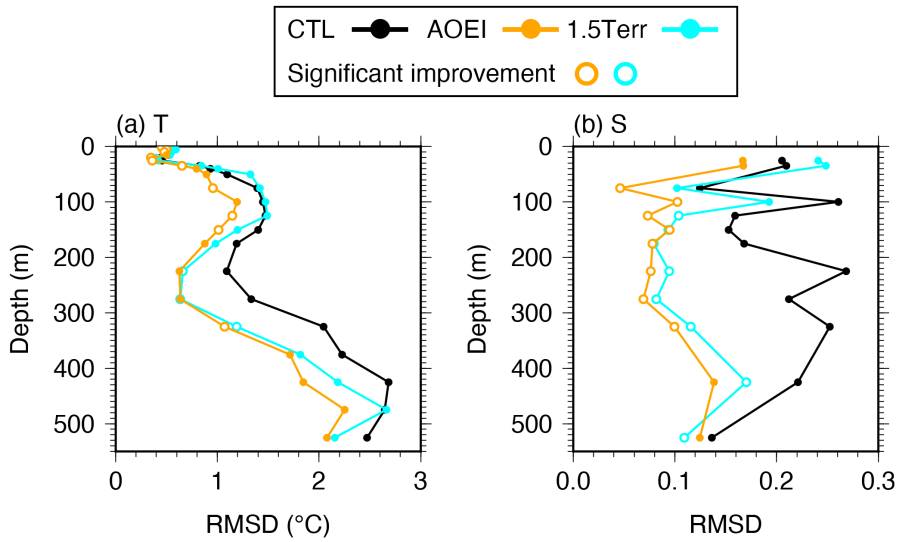
755 Figure 12: (a) Temperature and (b) salinity RMSDs averaged over the whole experiment period at the KEO buoy in the CTL (black), AOEI (orange), and 1.5Terr (cyan) runs. Open circles indicate significant improvement in the AOEI and 1.5Terr runs relative to the CTL run.
