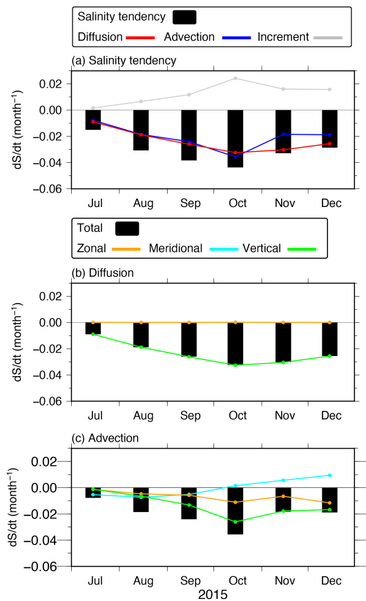
Figure B1: (a) Monthly mean for each term for the difference between the AOEI and CTL runs in the salinity budget equation [Eq. (B1)]: Salinity tendency difference term (the LHS term; black bars), salinity diffusion difference term (the first term on the RHS; red line), salinity advection difference term (the second term on the RHS; blue line), and salinity analysis increment difference term (the last term on the RHS; gray line). (b) and (c) Same as (a) but for the salinity diffusion and advection difference terms (black bars), respectively, and zonal (orange lines), meridional (cyan lines), and vertical (green lines) components.
