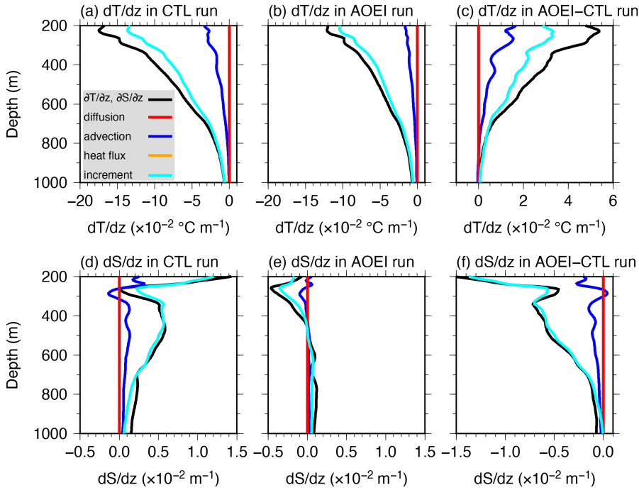
735 Figure 10: (a)–(c) Same as Fig. 9 but for each term of the temperature stratification tendency equation [Eq. (13)]: Temperature gradient tendency term (the LHS term; black), temperature diffusion gradient term (the first term on the RHS; red), temperature advection gradient term (the second term on the RHS; blue), shortwave penetration gradient term (the third term on the RHS; orange), and temperature increment gradient term (the last term on the RHS; cyan). (d)–(f) Same as (a)–(c) but for the salinity stratification tendency equation [Eq. (14)]. In (a)–(c), we note 740 that the shortwave penetration gradient term is almost zero and overlaps with the temperature diffusion gradient term.
