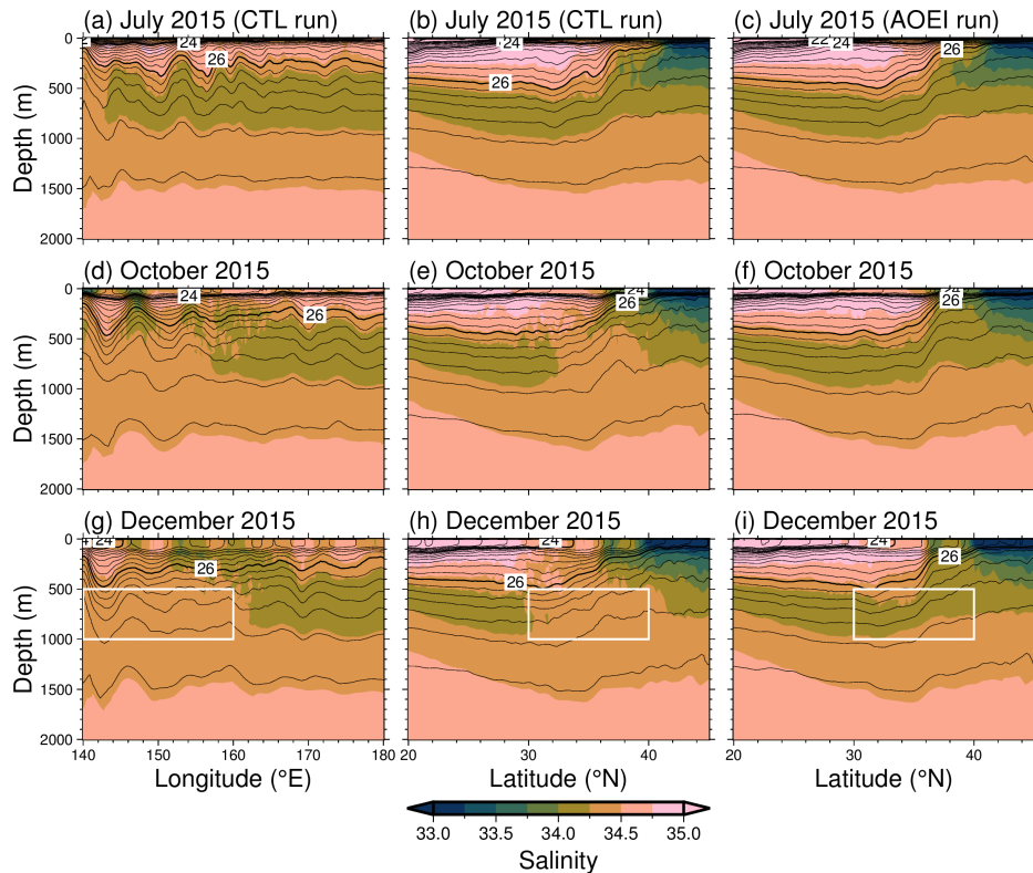
695 Figure 3: The zonal section of monthly-mean salinity (color) and potential density (contour) along 35°N in (a) July, (d) October, and (g) December 2015 in the CTL run. (b), (e), and (h) Same as (a), (d), and (g), but for the meridional section along 150°E. (c), (f), (i) Same as (b), (e), (h) but for AOEI run. Thin (thick) contour intervals are 0.25 (2) kg m -3 . The white box in (g) [(h) and (i)] encloses a longitude (latitude)-depth section of 140°–160°E (30°–40°N) and 500–1000 m depth.
