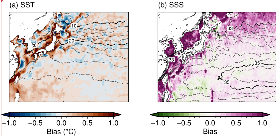
Figure 7: (a) SST and (b) SSS forecast biases (color) and averages (contour) over the whole experiment period in the AOEI run . Thin (thick) contour intervals are 2 (10) °C in (a) and 0.25 (2) in (b).
