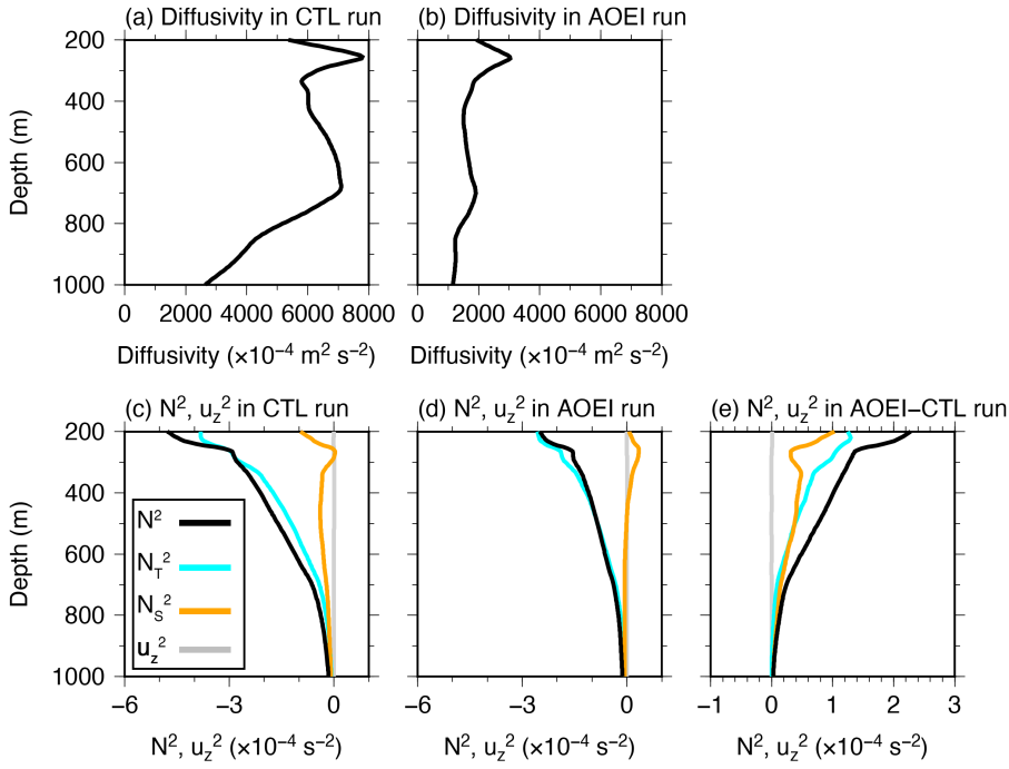
730 Figure 9: Total vertical diffusivity tendency during the positive vertical diffusivity tendency period averaged over the KE region ( 140^{\circ} – 160^{\circ} E, 30^{\circ} – 40^{\circ} N) in the (a) CTL and (b) AOEI runs. (c) and (d) Same as (a) but for the squared buoyancy frequency (black) and shear (gray) tendency. (e) Same as (c) and (d), but for the AOEI minus CTL run. In (c)–(e), cyan (orange) lines indicate contributions from \partial N_T^2 / \partial t ( \partial N_S^2 / \partial t ).
