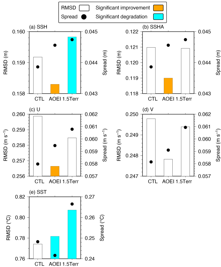
Figure 13: RMSDs for (a) SSH and (b) SSHA relative to the AVISO, surface (c) zonal and (d) meridional velocity relative to the drifter buoys, and (e) SSTs relative to the Himawari-8 averaged over the whole domain and period. Black dots indicate the ensemble spread in the observation space. We note that the ranges of the vertical axis are different between the RMSDs and ensemble spreads.
