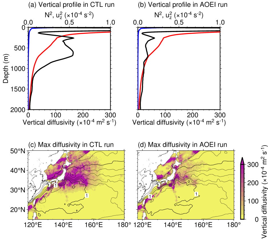
725 Figure 8: Vertical diffusivity (black), and squared buoyancy frequency (red) and shear (blue) averaged over the KE region (140°–160°E, 30°–40°N) for the whole experiment period in the (a) CTL and (b) AOEI runs. Maxima of the averaged vertical diffusivity for the whole experiment period within 300–1000 m depth in the (c) CTL and (d) AOEI runs. Black contours show SSH averaged over the whole period. Thin (thick) contour intervals are 0.2 (1) m.
