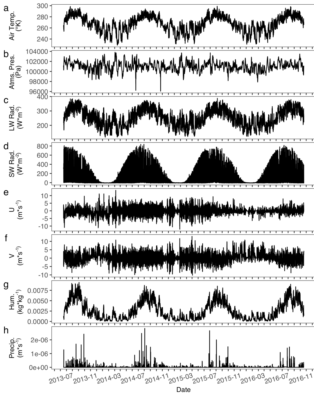
Figure A3. Toolik hourly meteorological data used in simulations. Air temperature ^{\circ}\text{K} (a), atmospheric pressure Pa (b), longwave radiation \text{W}\cdot\text{m}^{-2} (c), shortwave radiation \text{W}\cdot\text{m}^{-2} (d), 2 component wind speed \text{m}\cdot\text{s}^{-1} (e & f), humidity \text{kg}\cdot\text{kg}^{-1} (g), and precipitation \text{m}\cdot\text{s}^{-1} (h).
