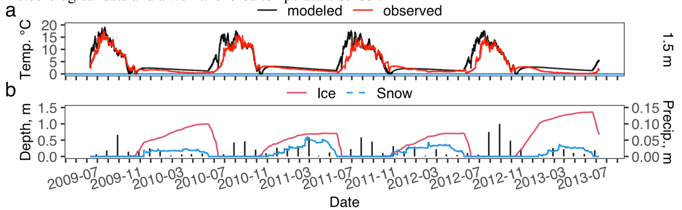
270 Figure 2. Fox Den Lake modeled and observed water temperature at 1.5 m (a) and modeled lake ice depth, modeled lake snow depth and 275 measured monthly precipitation (vertical black bars) (b).
