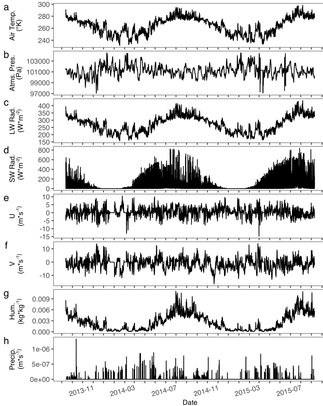
Figure A1. Atkasuk hourly meteorological data used in simulations. Air temperature ^{\circ}\text{K} (a), atmospheric pressure Pa (b), longwave radiation \text{W}\cdot\text{m}^{-2} (c), shortwave radiation \text{W}\cdot\text{m}^{-2} (d), 2 component wind speed \text{m}\cdot\text{s}^{-1} (e & f), humidity \text{kg}\cdot\text{kg}^{-1} (g), and precipitation \text{m}\cdot\text{s}^{-1} (h).
