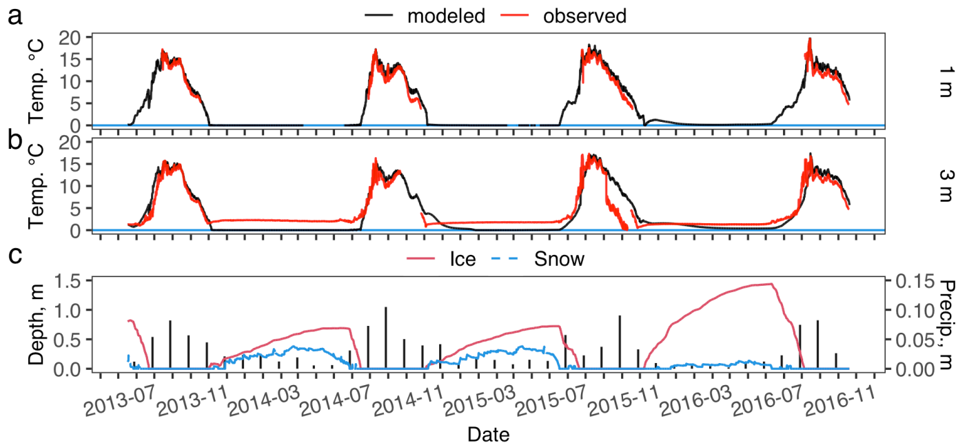
280 Figure 3. Toolik Lake modeled and observed lake water temperature at 1 m (a) and 3 m (b) and modeled lake ice depth, lake snow depth 285 and measured monthly precipitation (vertical black bars) (c). Missing observed data in (a) and (b) is due to seasonal placement and removal of the temperature sensors, see Methods for details. The y-axis of panel (a) is limited to water temperatures > 0^{\circ}\text{C} as the LAKE model water temperature is limited to > 0^{\circ}\text{C} .
