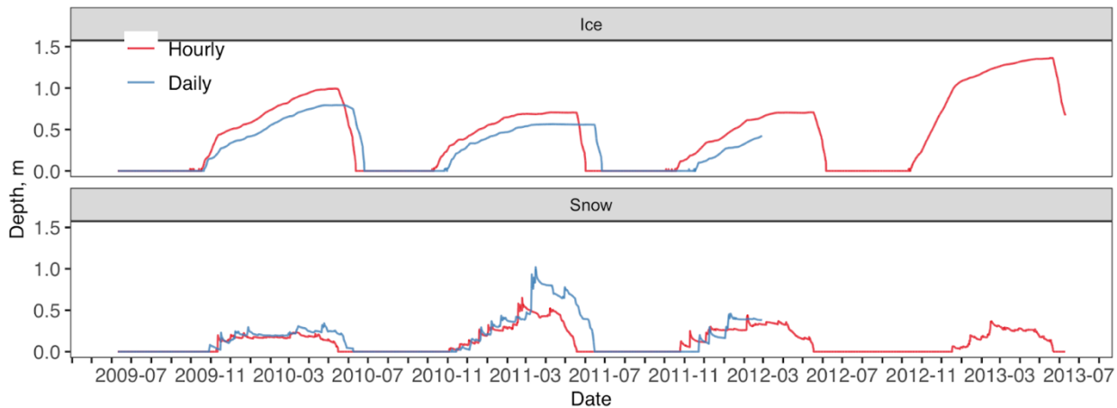
555 Figure F5. Fox Den ice and snow depth across different temporal resolution simulations. No observed data available, hourly temporal resolution in red and daily temporal resolution in blue.
