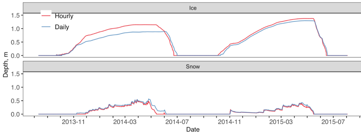
550 Figure F4. Atqasuk ice and snow depth across different temporal resolution simulations. No observed data available, hourly temporal resolution in red and daily temporal resolution in blue.
