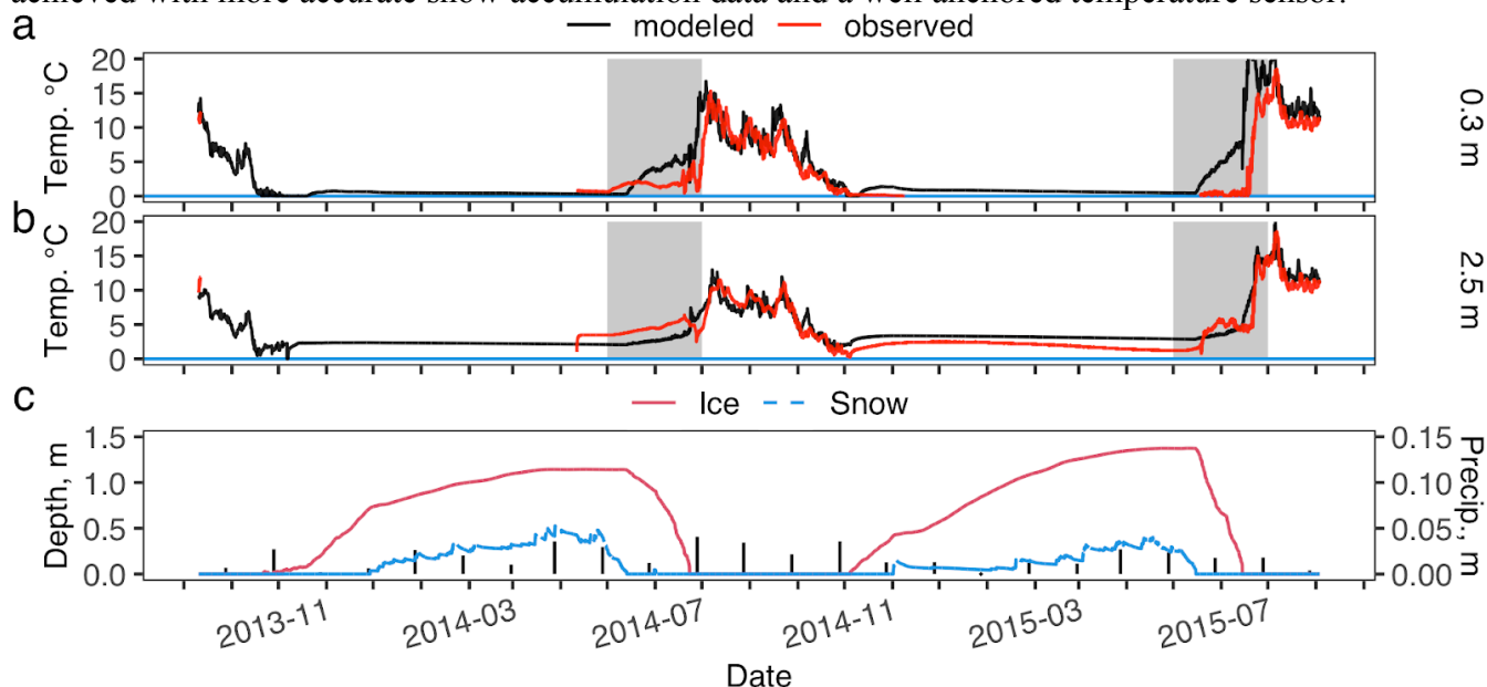
255 Figure 1. Atqasuk modeled and observed lake water temperature at 0.3 m (a) and 2.5 m (b) and modeled lake ice depth, lake snow depth and measured monthly precipitation (vertical black bars) (c). Gray shading indicates periods of uncertainty in temperature sensor depth when ice-raffing may have moved the sensor to shallower water. The y-axis of panel (a) is limited to water temperatures > 0^{\circ}\text{C} as the LAKE model water temperature is limited to > 0^{\circ}\text{C} .
