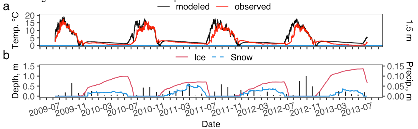
270 Figure 2. Fox Den Lake modeled and observed water temperature at 1.5 m (a) and modeled lake ice depth, modeled lake snow depth and measured monthly precipitation (vertical black bars) (b).
