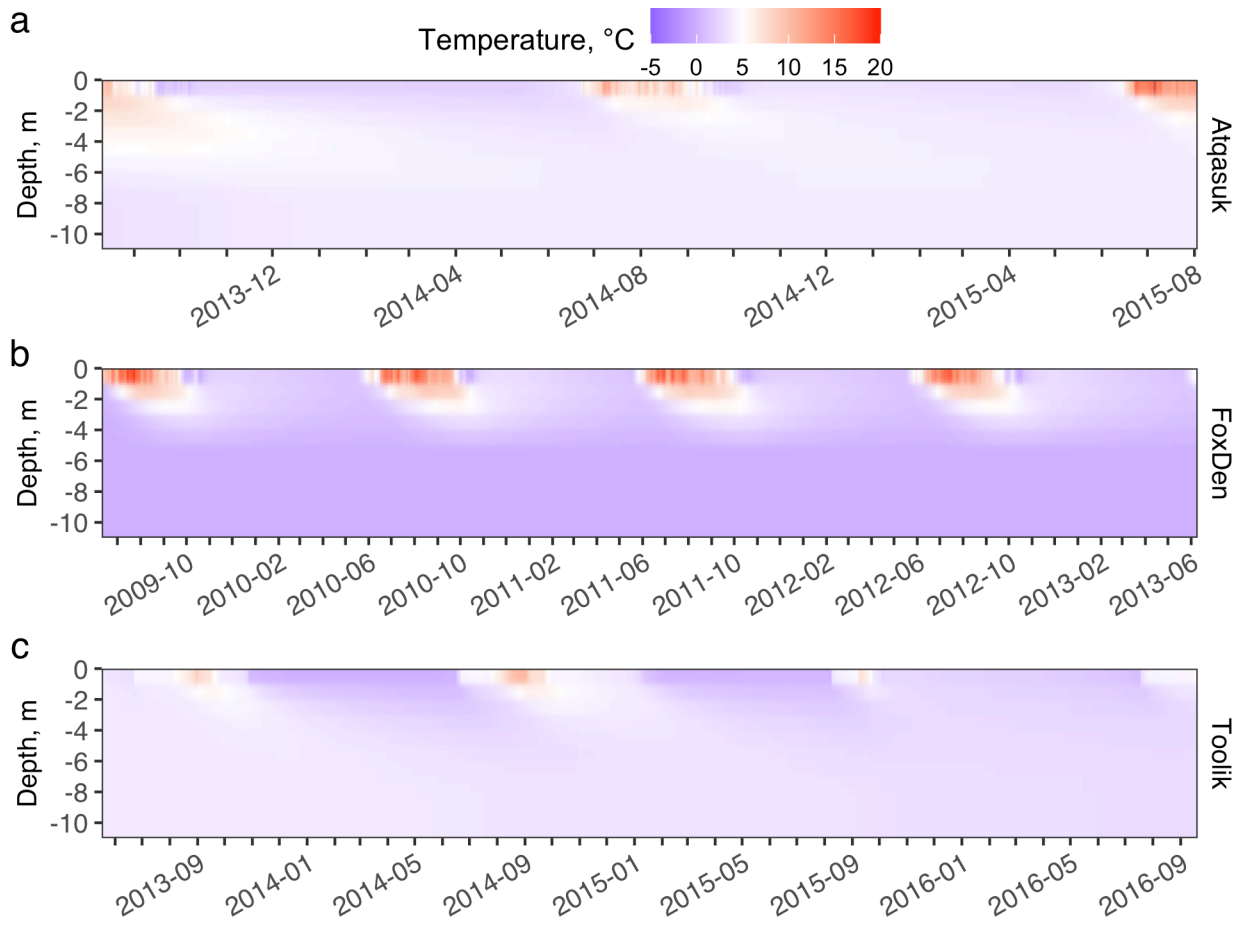
Figure C2. Baseline lake sediment temperature over the simulation period for Atqasuk (a), Fox Den (b), and Toolik Lake (c) from 0 m to 10 m depth.
