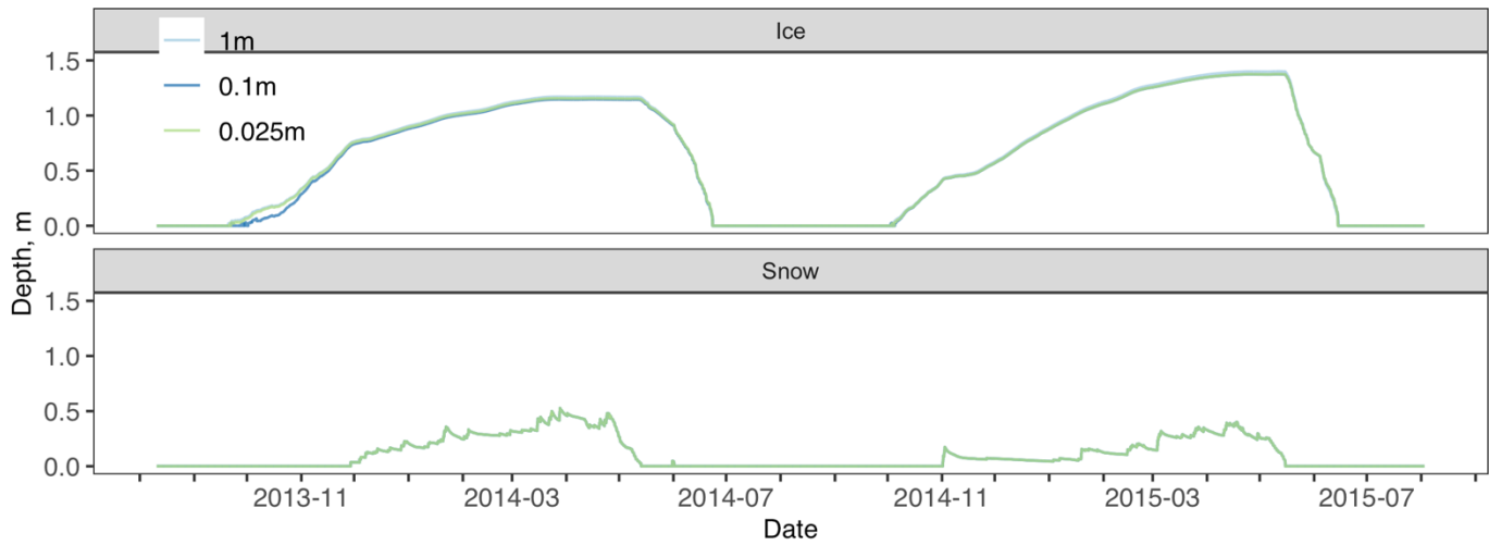
490 Figure D3. Atqasuk ice and snow depth across different water vertical resolution simulations. No observed data available, 1m vertical resolution in light blue, 0.1m vertical resolution in blue, 0.025m vertical resolution in green. Note data overlaps for most of the time series.
