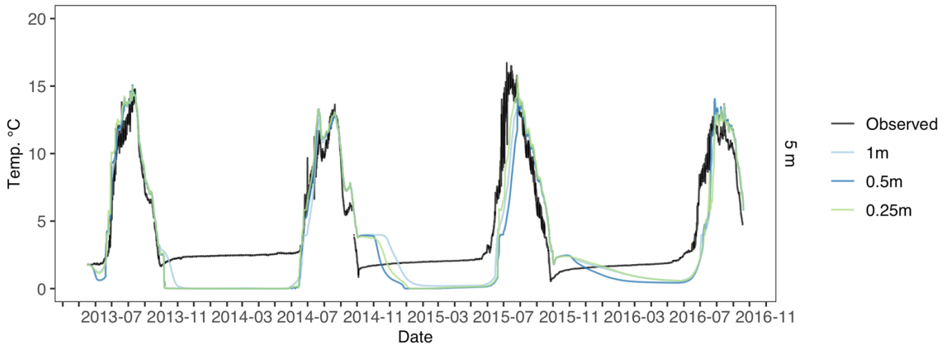
Figure D6. Toolik 5m water temperature across different water vertical resolution simulations. Observed water temperature in black, 1m vertical resolution in light blue, 0.5m vertical resolution in blue, 0.25m vertical resolution in green.
