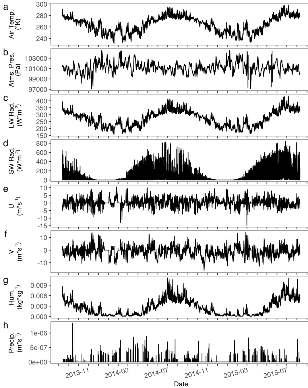
445 Figure A1. Atqasuk hourly meteorological data used in simulations. Air temperature ^{\circ}\text{K} (a), atmospheric pressure Pa (b), longwave radiation \text{W m}^{-2} (c), shortwave radiation \text{W m}^{-2} (d), 2 component wind speed \text{m s}^{-1} (e & f), humidity \text{kg kg}^{-1} (g), and precipitation \text{m s}^{-1} (h).
