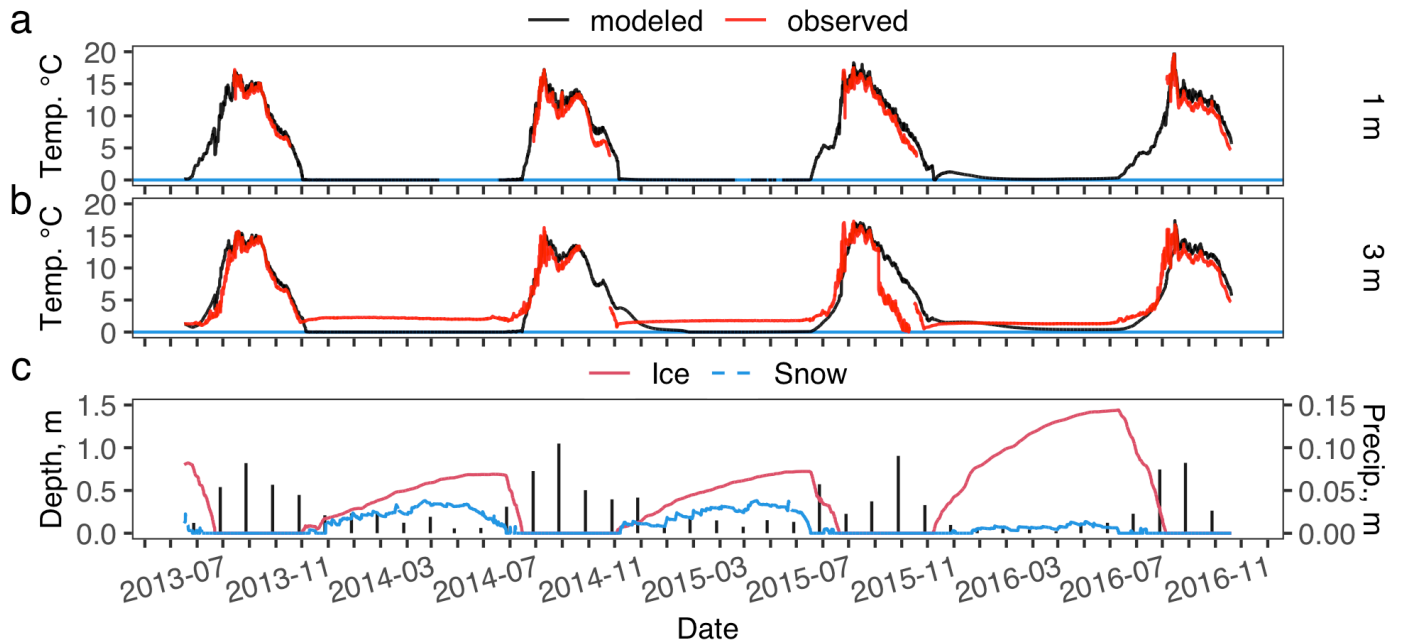
280 Figure 3. Toolik Lake modeled and observed lake water temperature at 1 m (a) and 3 m (b) and modeled lake ice depth, lake snow depth and measured monthly precipitation (vertical black bars) (c). Missing observed data in (a) and (b) is due to seasonal placement and removal of the temperature sensors, see Methods for details. The y-axis of panel (a) is limited to water temperatures > 0^{\circ}\text{C} as the LAKE model water temperature is limited to > 0^{\circ}\text{C} .
