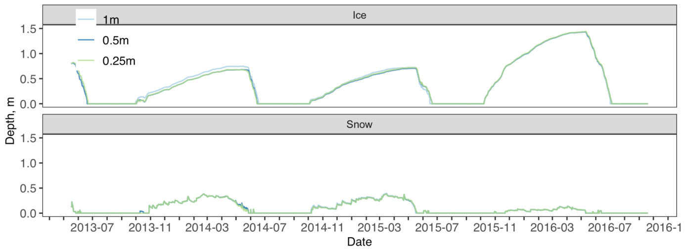
515 Figure D9. Toolik ice and snow depth across different water vertical resolution simulations. No observed data available, 1m vertical resolution in light blue, 0.5m vertical resolution in blue, 0.25m vertical resolution in green.
