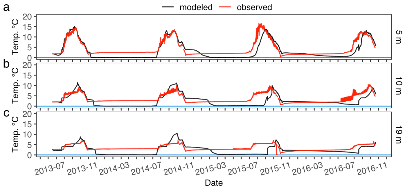
290 Figure 4. Toolik Lake modeled and observed lake water temperature at 5 m (a), 10 m (b) and 19 m (c).
