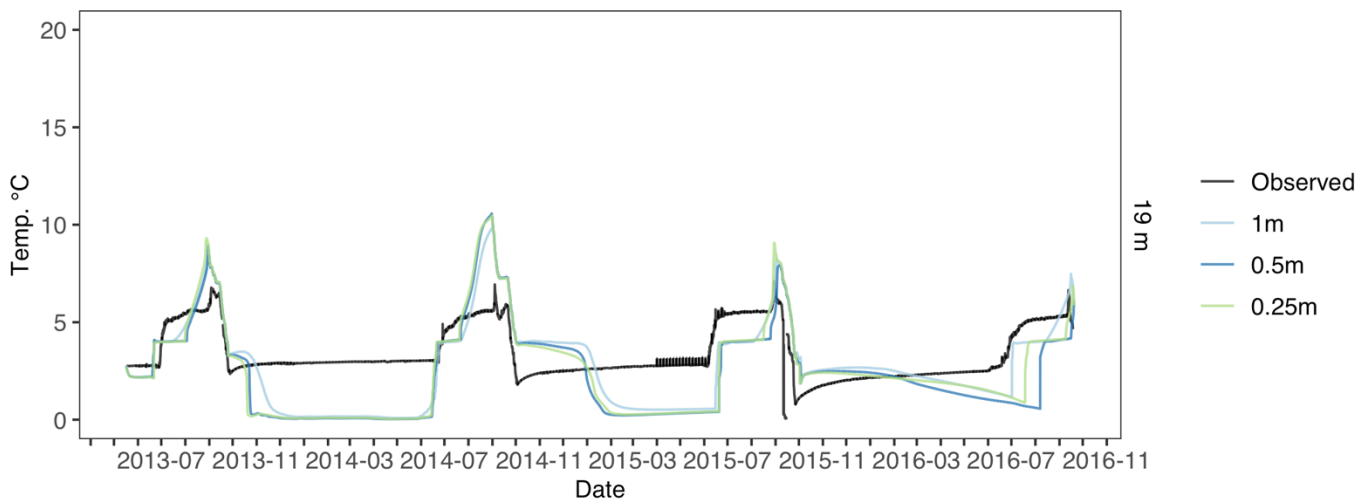
Figure D8. Toolik 19m water temperature across different water vertical resolution simulations. Observed water temperature in black, 1m vertical resolution in light blue, 0.5m vertical resolution in blue, 0.25m vertical resolution in green.
