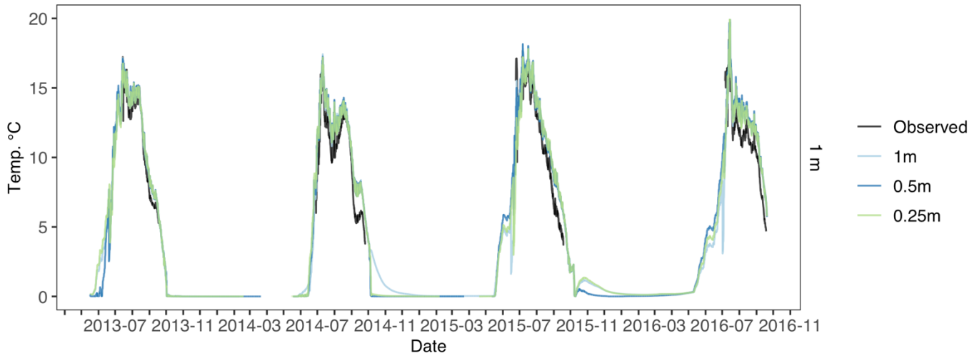
500 Figure D4. Toolik 1m water temperature across different water vertical resolution simulations. Observed water temperature in black, 1m vertical resolution in light blue, 0.5m vertical resolution in blue, 0.25m vertical resolution in green.
