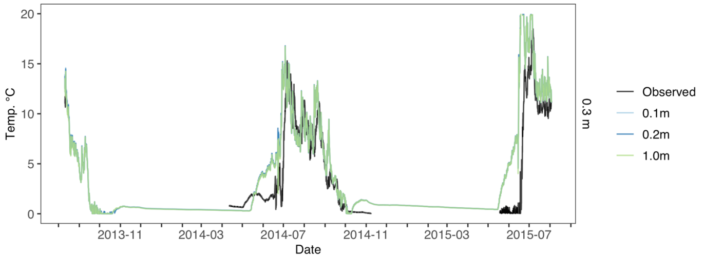
525 Figure E1. Atqasuk 0.3m water temperature across different soil vertical resolution simulations. Observed water temperature in black, 0.1m vertical resolution in light blue, 0.2m vertical resolution in blue, 1.0m vertical resolution in green.
