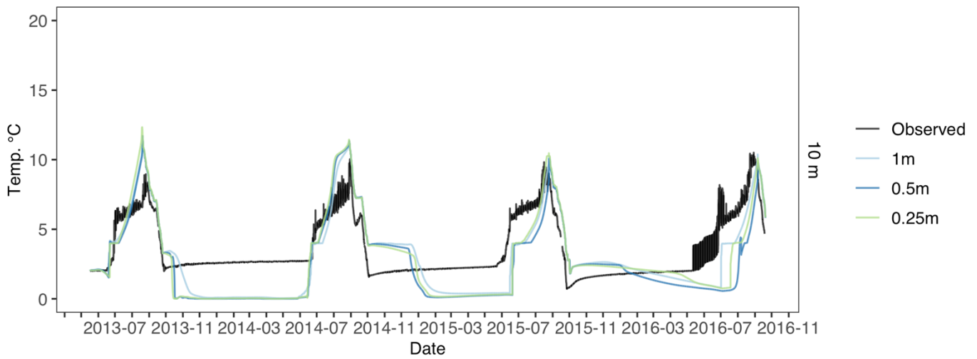
Figure D7. Toolik 10m water temperature across different water vertical resolution simulations. Observed water temperature in black, 1m vertical resolution in light blue, 0.5m vertical resolution in blue, 0.25m vertical resolution in green.
