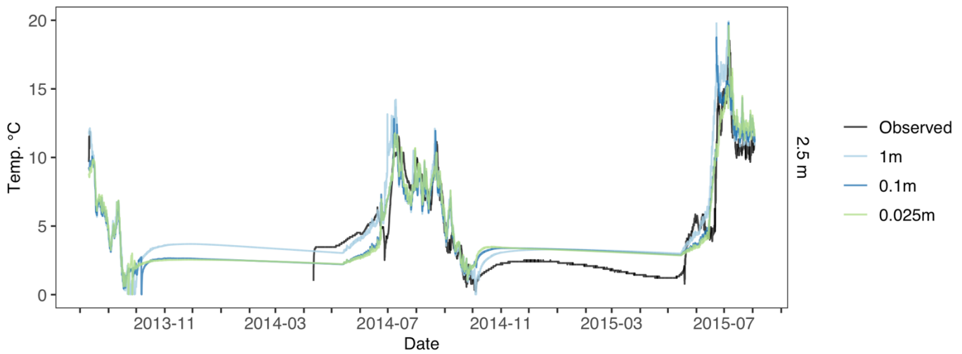
485 Figure D2. Atqasuk 2.5m water temperature across different water vertical resolution simulations. Observed water temperature in black, 1m vertical resolution in light blue, 0.1m vertical resolution in blue, 0.025m vertical resolution in green. Note 0.1m and 0.025m overlap for most of the time series.
