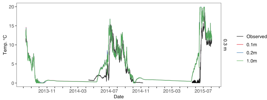
580 Figure E1. Atqasuk 0.3m water temperature across different soil vertical resolution simulations. Observed water temperature in black, 0.1m vertical resolution in red, 0.2m vertical resolution in blue, 1.0m vertical resolution in green.
