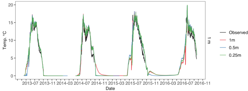
545 Figure D4. Toolik 1m water temperature across different water vertical resolution simulations. Observed water temperature in black, 1m vertical resolution in red, 0.5m vertical resolution in blue, 0.25m vertical resolution in green.
