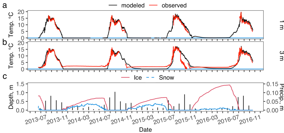
295 Figure 3. Toolik Lake modeled and observed lake water temperature at 1 m (a) and 3 m (b) and modeled lake ice depth, lake snow depth and measured monthly precipitation (vertical black bars) (c). Missing observed data in (a) and (b) is due to seasonal placement and removal of the temperature sensors, see Methods for details. The y-axis of panel (a) is limited to water temperatures > 0 °C as the LAKE model water temperature is limited to > 0 °C.
