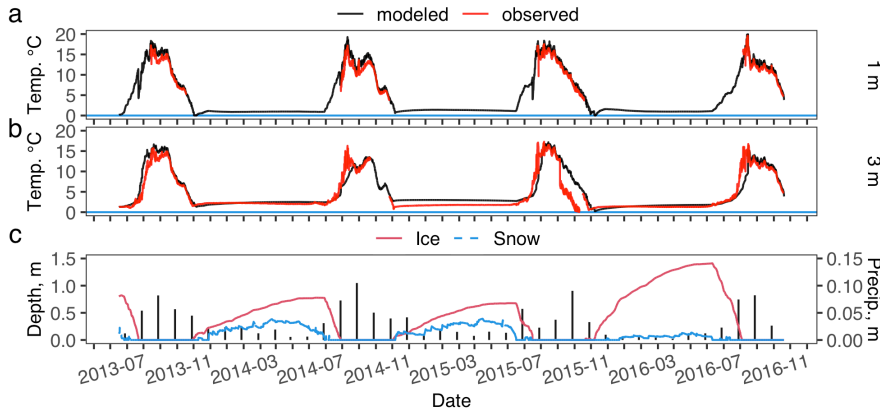
495 Figure B1. Modeled and observed lake water temperature at 1 m (a) and 3 m (b) and modeled lake ice depth, lake snow depth and measured monthly precipitation (vertical black bars) (c) for Toolik Lake with no inflow. Missing observed data in (a) and (b) is due to seasonal placement and removal of the temperature sensors, see Methods for details.
