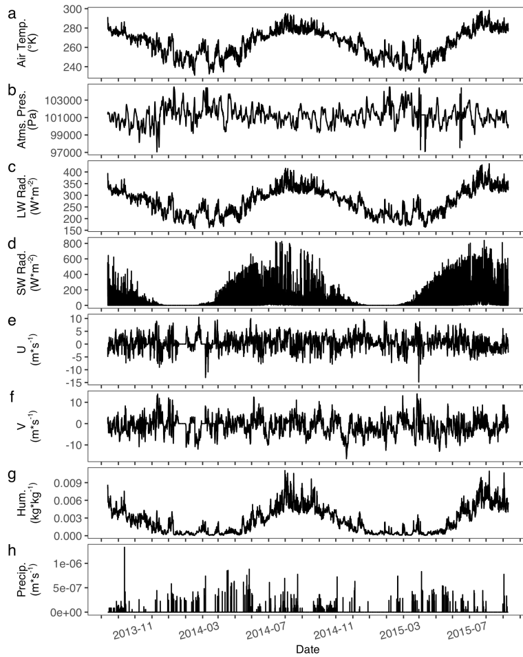
480 Figure A1. Atqasuk hourly meteorological data used in simulations. Air temperature °K (a), atmospheric pressure Pa (b), longwave radiation W m^{-2} (c), shortwave radiation W m^{-2} (d), 2 component wind speed m s^{-1} (e & f), humidity kg kg^{-1} (g), and precipitation m s^{-1} (h).
