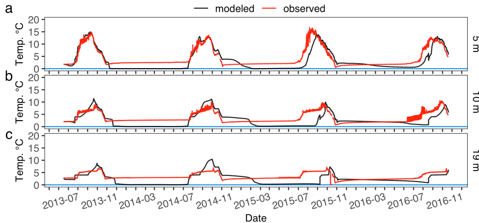
305 Figure 4. Toolik Lake modeled and observed lake water temperature at 5 m (a), 10 m (b) and 19 m (c).
