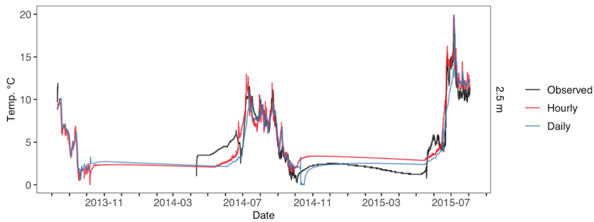
Figure F2. Atqasuk 2.5m water temperature across different temporal resolution simulations. Observed water temperature in black, hourly temporal resolution in red and daily temporal resolution in blue.
