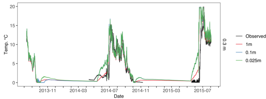
¶25 Figure D1. Atqasuk 0.3m water temperature across different water vertical resolution simulations. Observed water temperature in black, 1m vertical resolution in red, 0.1m vertical resolution in blue, 0.025m vertical resolution in green. Note 0.1m and 0.025m overlap for most of the time series.
