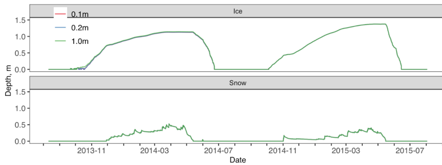
Figure E3. Atqasuk ice and snow depth across different soil vertical resolution simulations. No observed data available, 0.1m vertical resolution in red, 0.2m vertical resolution in blue, 1.0m vertical resolution in green.
