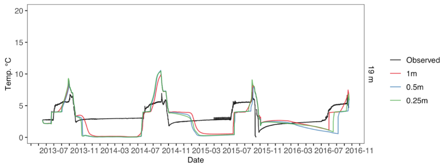
565 Figure D8. Toolik 19m water temperature across different water vertical resolution simulations. Observed water temperature in black, 1m vertical resolution in red, 0.5m vertical resolution in blue, 0.25m vertical resolution in green.
