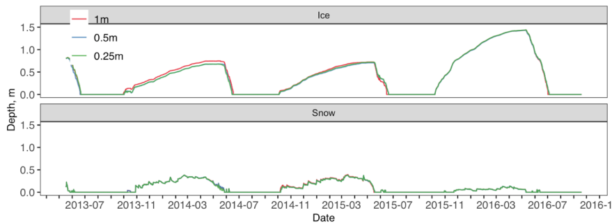
570 Figure D9. Toolik ice and snow depth across different water vertical resolution simulations. No observed data available, 1m vertical resolution in red, 0.5m vertical resolution in blue, 0.25m vertical resolution in green.
