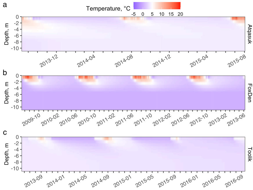
515 Figure C2. Baseline lake sediment temperature over the simulation period for Atqasuk (a), Fox Den (b), and Toolik Lake (c) from 0 m to 10 m depth.
