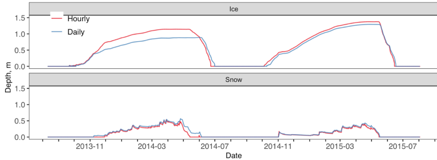
Figure F4. Atqasuk ice and snow depth across different temporal resolution simulations. No observed data available, hourly temporal resolution in red and daily temporal resolution in blue.
