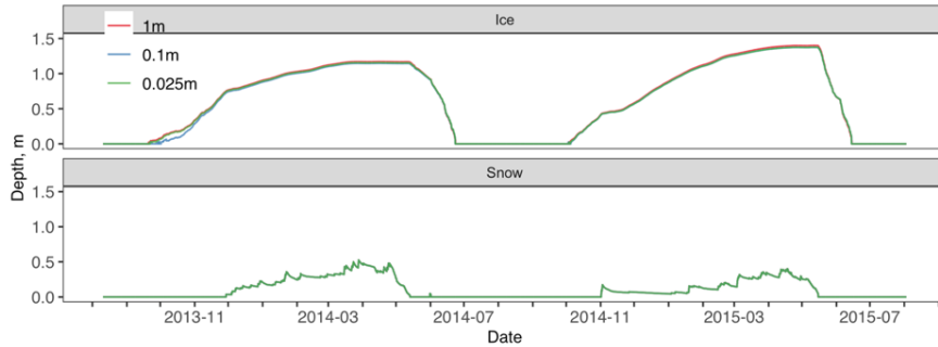
535 Figure D3. Atqasuk ice and snow depth across different water vertical resolution simulations. No observed data available, 1m vertical resolution in red, 0.1m vertical resolution in blue, 0.025m vertical resolution in green. Note data overlaps for most of the time series.
