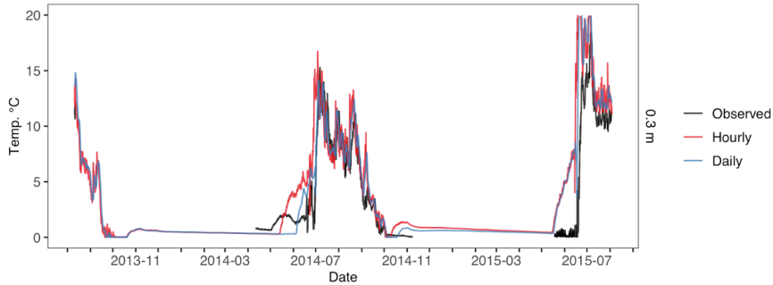
600 Figure F1. Atqasuk 0.3m water temperature across different temporal resolution simulations. Observed water temperature in black, hourly temporal resolution in red and daily temporal resolution in blue.
