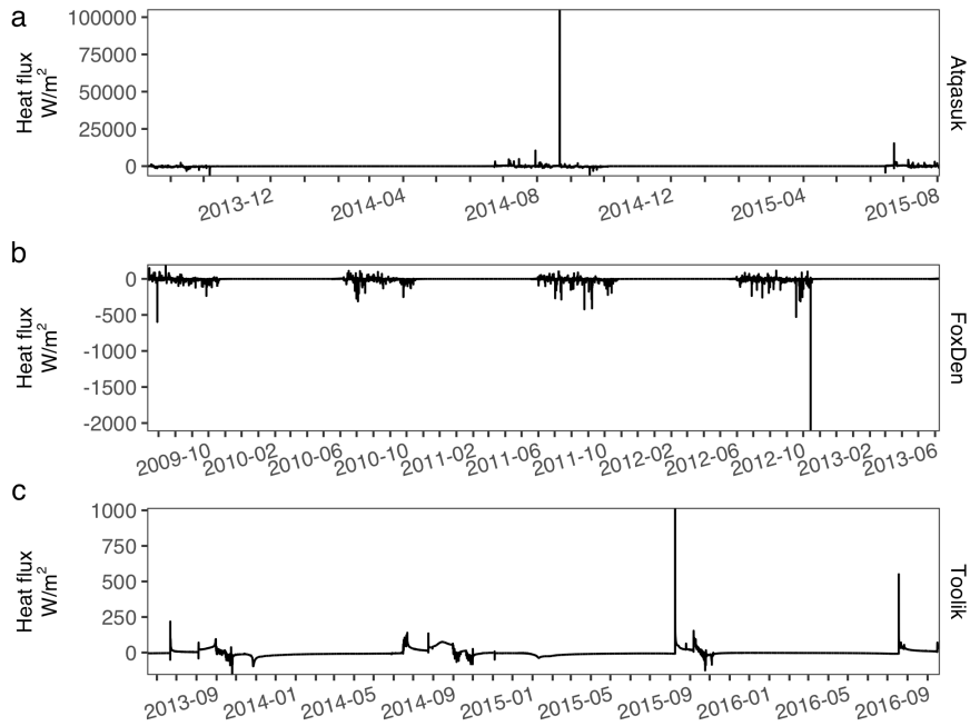
¶20 Figure C3. Downward heat flux at the bottom of the water column over the baseline simulation period for Atqasuk (a), Fox Den (b), and Toolik Lake (c).
