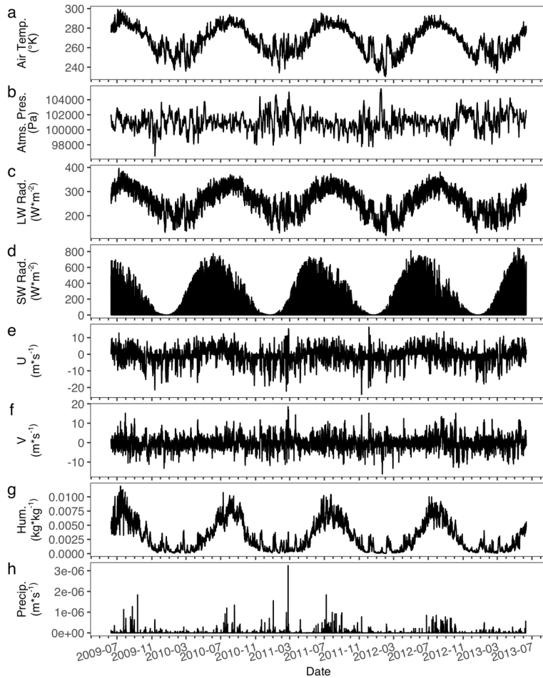
485 Figure A2. Fox Den hourly meteorological data used in simulations. Air temperature °K (a), atmospheric pressure Pa (b), longwave radiation W m^2 (c), shortwave radiation W m^2 (d), 2 component wind speed m s^{-1} (e & f), humidity kg kg^{-1} (g), and precipitation m s^{-1} (h).
