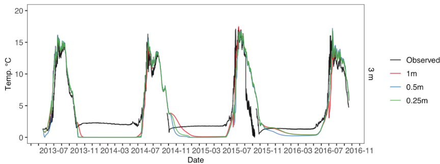
550 Figure D5. Toolik 3m water temperature across different water vertical resolution simulations. Observed water temperature in black, 1m vertical resolution in red, 0.5m vertical resolution in blue, 0.25m vertical resolution in green.
