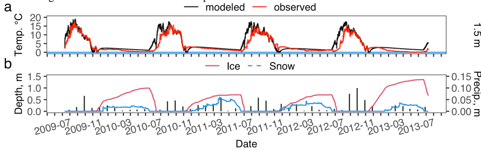
285 Figure 2. Fox Den Lake modeled and observed water temperature at 1.5 m (a) and modeled lake ice depth, modeled lake snow depth and measured monthly precipitation (vertical black bars) (b).
