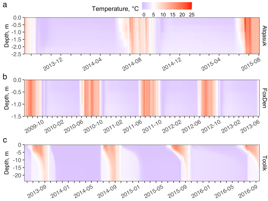
510 Figure C1. Baseline lake water temperature over the simulation period for Atqasuk (a), Fox Den (b), and Toolik Lake (c).
