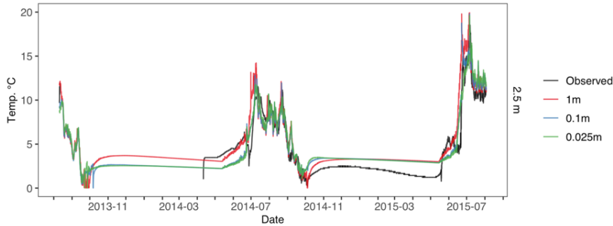
530 Figure D2. Atqasuk 2.5m water temperature across different water vertical resolution simulations. Observed water temperature in black, 1m vertical resolution in red, 0.1m vertical resolution in blue, 0.025m vertical resolution in green. Note 0.1m and 0.025m overlap for most of the time series.
