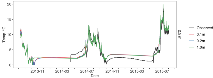
Figure E2. Atqasuk 2.5m water temperature across different soil vertical resolution simulations. Observed water temperature in black, 0.1m vertical resolution in red, 0.2m vertical resolution in blue, 1.0m vertical resolution in green.
