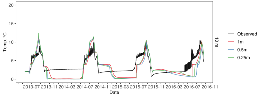
560 Figure D7. Toolik 10m water temperature across different water vertical resolution simulations. Observed water temperature in black, 1m vertical resolution in red, 0.5m vertical resolution in blue, 0.25m vertical resolution in green.
