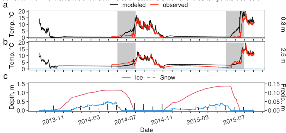
270 Figure 1. Atqasuk modeled and observed lake water temperature at 0.3 m (a) and 2.5 m (b) and modeled lake ice depth, lake snow depth and measured monthly precipitation (vertical black bars) (c). Gray shading indicates periods of uncertainty in temperature sensor depth when ice-rafting may have moved the sensor to shallower water. The y-axis of panel (a) is limited to water temperatures > 0 °C as the LAKE model water temperature is limited to > 0 °C.
