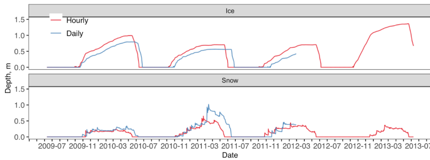
Figure F5. Fox Den ice and snow depth across different temporal resolution simulations. No observed data available, hourly temporal resolution in red and daily temporal resolution in blue.
