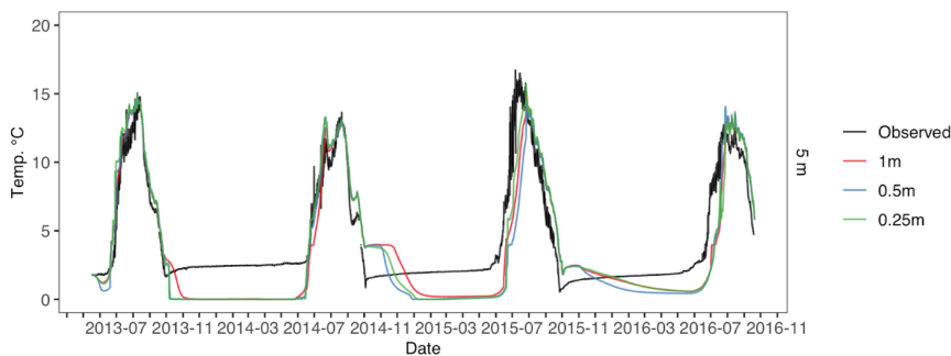
Figure D6. Toolik 5m water temperature across different water vertical resolution simulations. Observed water temperature in black, 1m vertical resolution in red, 0.5m vertical resolution in blue, 0.25m vertical resolution in green.
