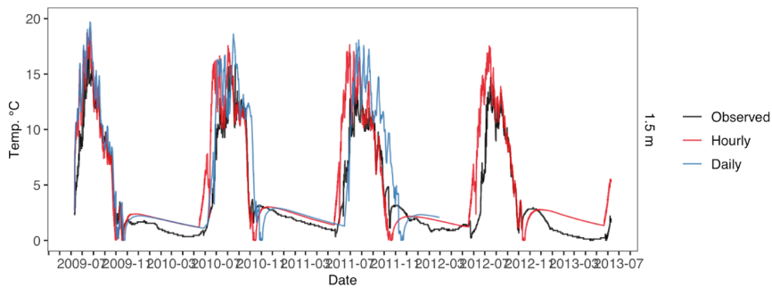
605 Figure F3. Fox Den 1.5m water temperature across different temporal resolution simulations. Observed water temperature in black, hourly temporal resolution in red and daily temporal resolution in blue.
