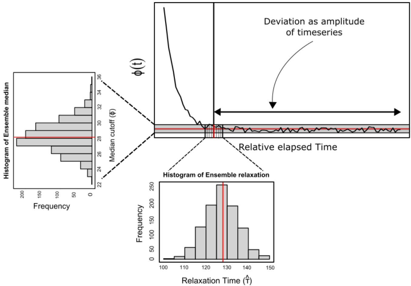
Figure 3: The bootstrapping technique used to calculate the uncertainty in the relaxation timescale. The resampled median about a reference 405 provides a replicate over which the standard error estimate is defined. The solid red represents the expected value of the quantity estimated while the vertical red line is the deviation from this expected value.
