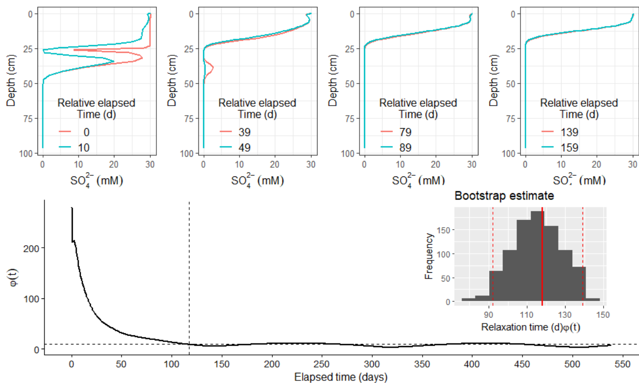
Figure 5: Scenario 1 (EMI): Model evolution for sulfate following deposition. Relative deviation of successive profile with time shown below. Dashed vertical line signify cutoff point by the median (Dashed horizontal line). Inset: Histogram of bootstrap estimate of sulfate relaxation timescale for EMI with 95 % confidence interval.
