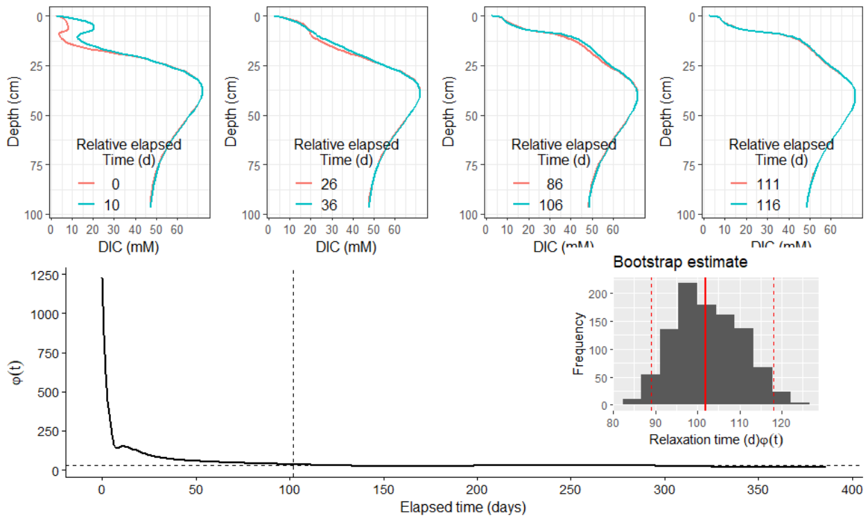
Figure 8: Scenario 2 (EM2): Model evolution for DIC following deposition. Relative deviation of successive profile with time shown below. Dashed vertical line signify cutoff point by the median (Dashed horizontal line). Inset: Histogram of bootstrap estimate of DIC relaxation timescale for EM2 with 95 % confidence interval.
