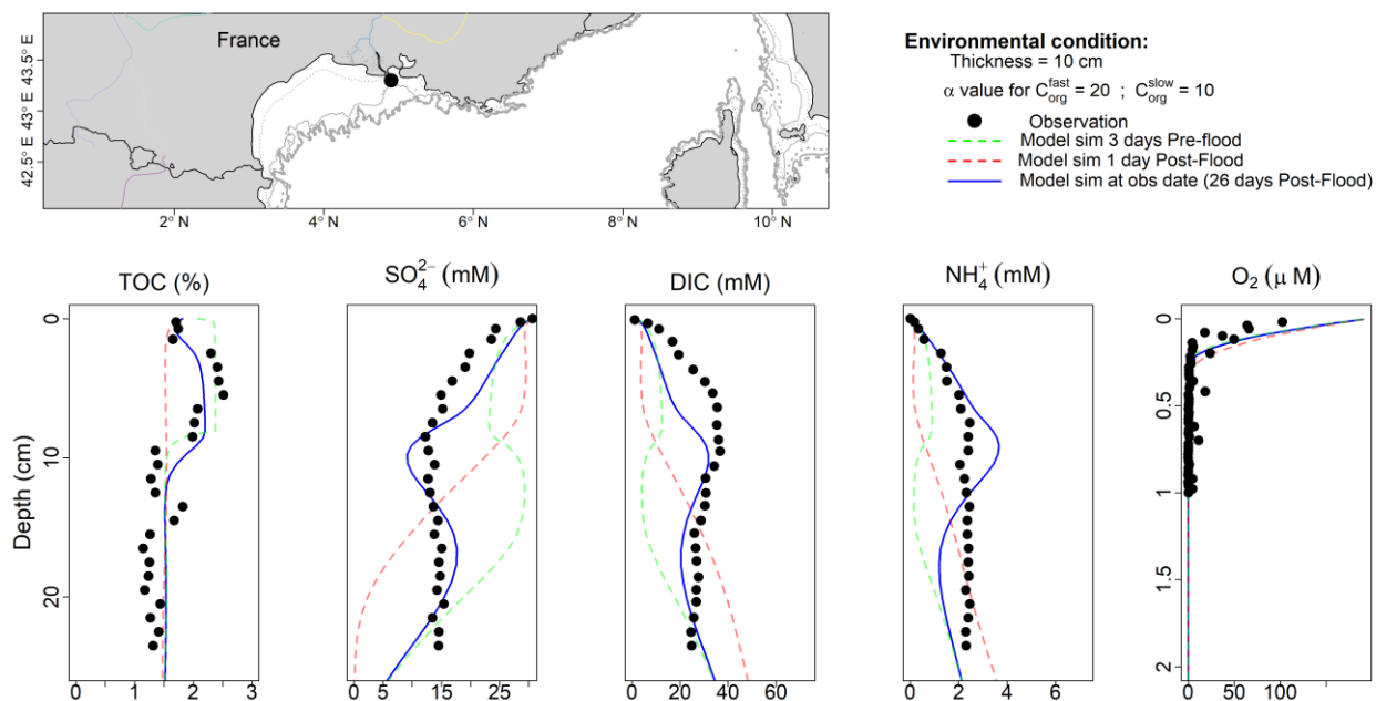
Figure 4: Model and observation depth profile of TOC (%), SO_4^{2-} , DIC, NH_4^+ and O_2 for November/December Event in Station A (Rhône Prodelta). The green and red dashed lines depict the vertical depth profile of the model before (3 days) and after (1 day) the flood deposit. The blue solid line represents the model result on the day the observations were collected (26 days after the flood, as indicated by the black circle).
