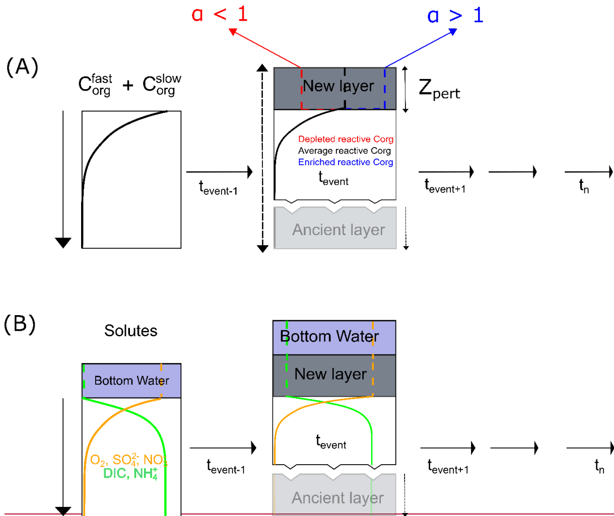
345 Figure 2: Schematic of model implementation for the deposition event scenario. Profile from previous time step (left) and after addition of new layer over a predefined depth layer (right). For the solid (A), the new layer can be enriched (blue) or depleted (red) relative to the old (average) (black). The dissolved substance (B) are set equal to the bottom water concentration during the deposition. Thereafter, the profile is integrated forward with time. The whole sequence of step occurs dynamically with time capitalizing on the integrator ability to simulate dynamic event process. \alpha is the carbon enrichment factor applied over depth Z_{pert} (see text for detail).
