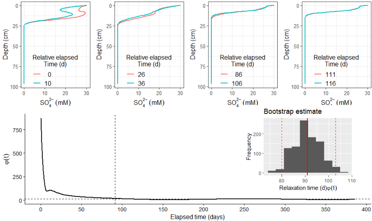
Figure 7: Scenario 2 (EM2): Model evolution for sulfate following deposition. Relative deviation of successive profile with time shown below. Dashed vertical line signifies cutoff point by the median (Dashed horizontal line). Inset: Histogram of bootstrap estimate of sulfate relaxation timescale for EM2 with 95 % confidence interval.
