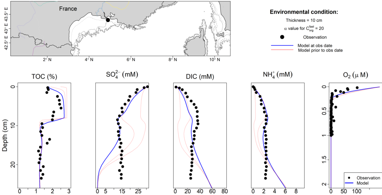
Figure 4: Model and observation depth profile of TOC (%), \text{SO}_4^{2-} , DIC, \text{NH}_4^+ and \text{O}_2 for November/December Event in Station A (Rhône Prodelta). Model results are at 26 days after flood event in blue line. Data collected in December 8, 2008 showed in black circle. The red lines represent the evolution of the model from the deposition (day 0 and 10).
