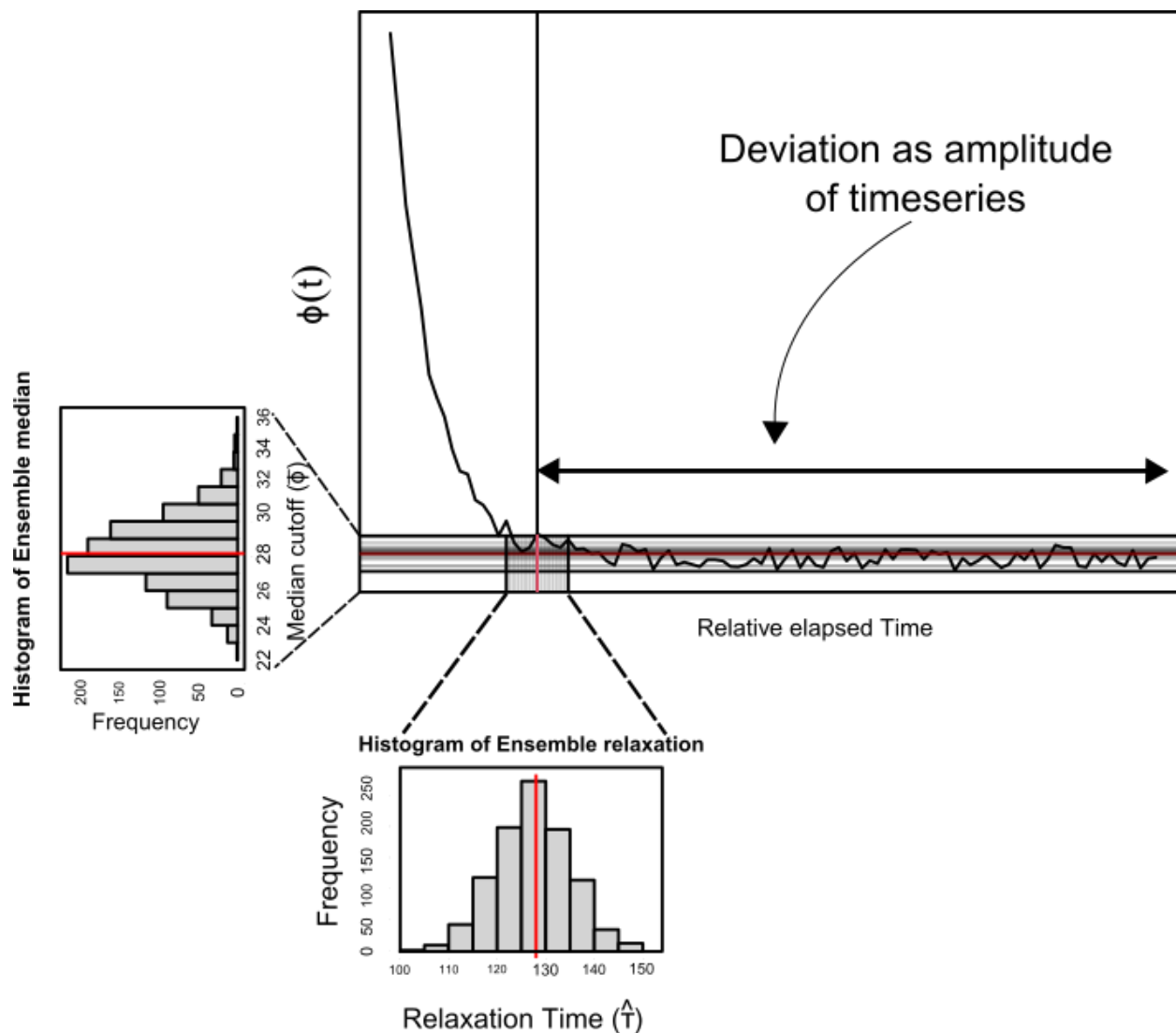
480 Figure 3: The bootstrapping technique used to calculate the uncertainty in the relaxation timescale. The resampled median about a reference provides a replicate over which the standard error estimate is defined. The solid red represents the expected value of the quantity estimated while the vertical red line is the deviation from this expected value.
