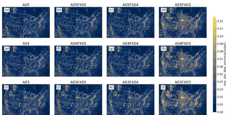
Figure 89: Maximum absolute bias (versus the orig simulation) for NH 3 calculated from hourly output for all simulations and cases.
