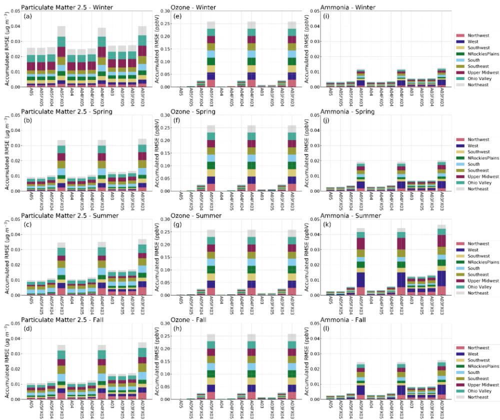
Figure 56: Stacked bar plots of changes to RMSE (y-axis) stratified by region (color), simulation and case (x-axis), and season (subplot) for hourly PM 2.5 , O 3 , and NH 3 calculated from grid-grid pairs with respect to the orig simulation.
