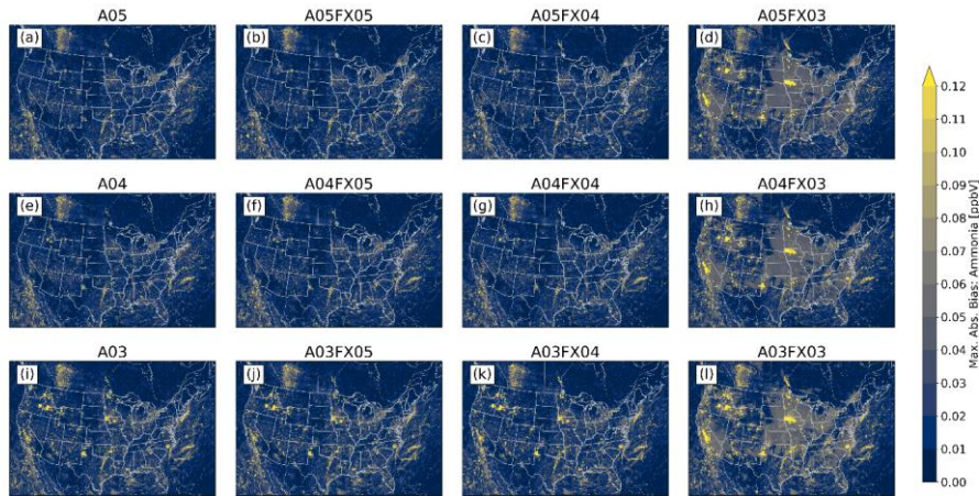
Figure 8: Maximum absolute bias (versus the orig simulation) for \text{NH}_3 calculated from hourly output for all simulations and cases.
