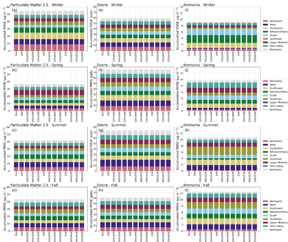
Figure 4: Stacked bar plots of RMSE (y-axis) stratified by region (color), simulation and case (x-axis), and season (subplot) for daily PM 2.5 , MDA8 O 3 , and daily NH 4 two-week averaged NH 3 calculated from in situ observation.
