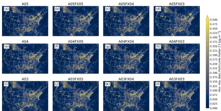
285 Figure 6: Maximum absolute bias (versus the orig simulation) for PM_{2.5} calculated from hourly output for all simulations and cases.
