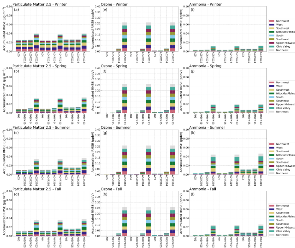
Figure 5: Stacked bar plots of RMSE (y-axis) stratified by region (color), simulation and case (x-axis), and season (subplot) for hourly PM 2.5 , O 3 , and NH 3 calculated from grid-grid pairs with respect to the orig simulation.
