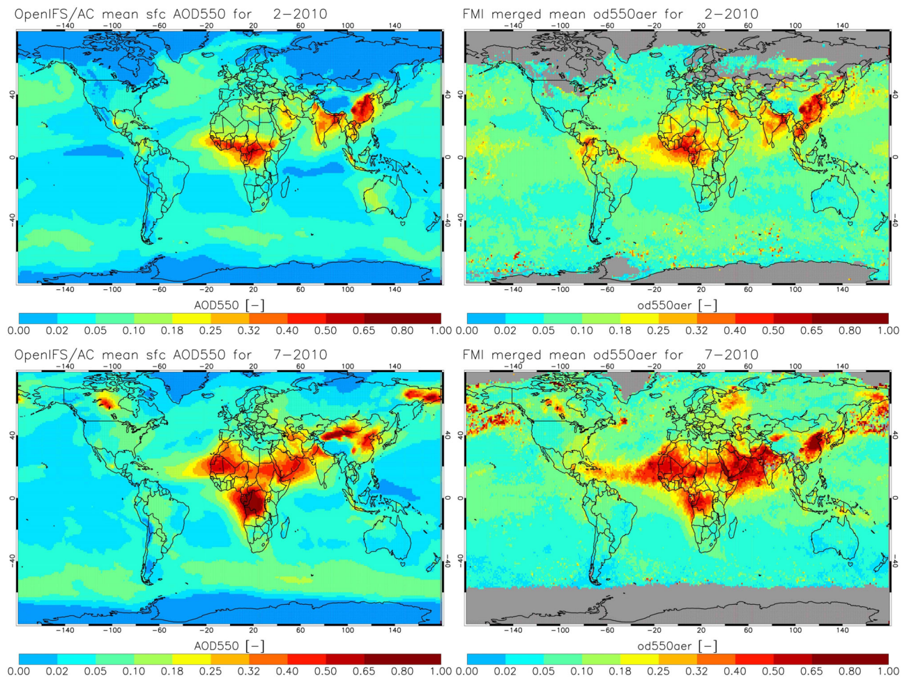
Figure 8. Intercomparison of total AOD at 550 nm for February and July 2010, for OpenIFS/AC-CB05-AER and the FMI merged AOD product.
