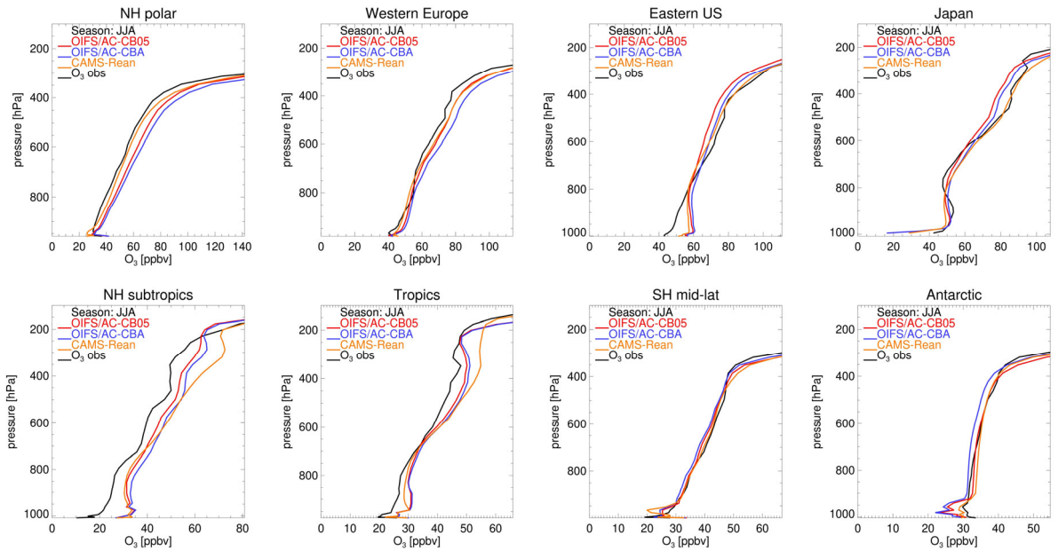
Figure 2. Evaluation of OpenIFS/AC tropospheric O 3 profiles against sondes during June-July-August 2010. For reference also data from the CAMS reanalysis is provided (orange).
