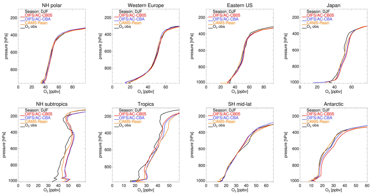
Figure 1. Evaluation of OpenIFS/AC tropospheric O 3 profiles against sondes during December-January-February 2010. For reference also data from the CAMS reanalysis is provided (orange).
