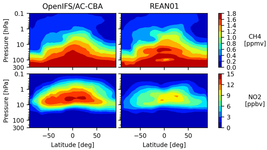
Figure 4. Latitude-pressure distributions of zonally averaged CH 4 (top) and NO 2 (bottom) on 1 October 2010 by OpenIFS/AC-CBA (left) and a BASCOE reanalysis of MIPAS observations (right).
