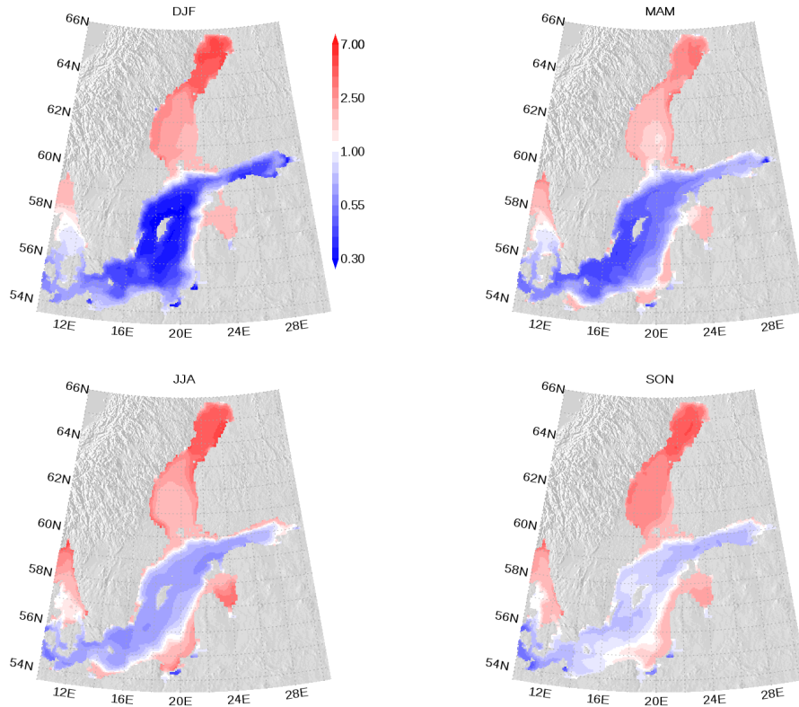
Figure 9. Seasonal mean elemental nitrogen to phosphorus ratio climatology in surface organic matter. The ratio is normalized and a ratio of one refers to the classical Redfield ratio. The map was created using the software package GrADS 2.1.1.b0 ( http://cola.gmu.edu/grads/ , last access: 14 December 2021), using published topography data (Seifert et al., 2008).
