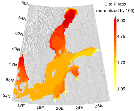
Figure 8. Annual mean elemental carbon to phosphorus ratio in surface organic matter. The ratio is normalized and a ratio of one refers to the classical Redfield ratio. The map was created using the software package GrADS 2.1.1.b0 ( http://cola.gmu.edu/grads/ , last access: 14 December 2021), using published topography data (Seifert et al., 2008).
