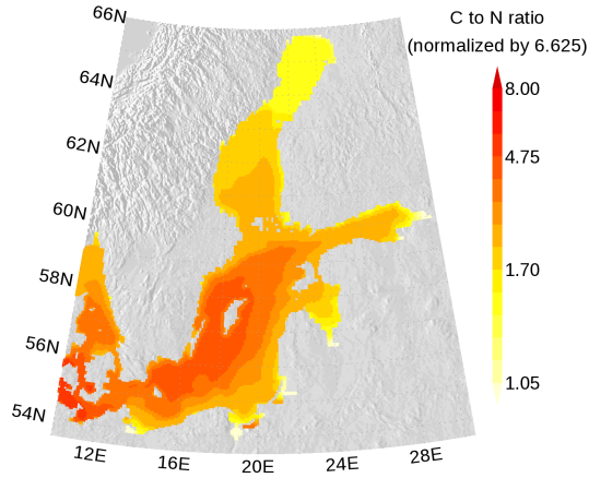
Figure 7. Annual mean elemental carbon to nitrogen ratio in surface organic matter. The ratio is normalized and a ratio of one refers to the classical Redfield ratio. The map was created using the software package GrADS 2.1.1.b0 ( http://cola.gmu.edu/grads/ , last access: 14 December 2021), using published topography data (Seifert et al., 2008).
