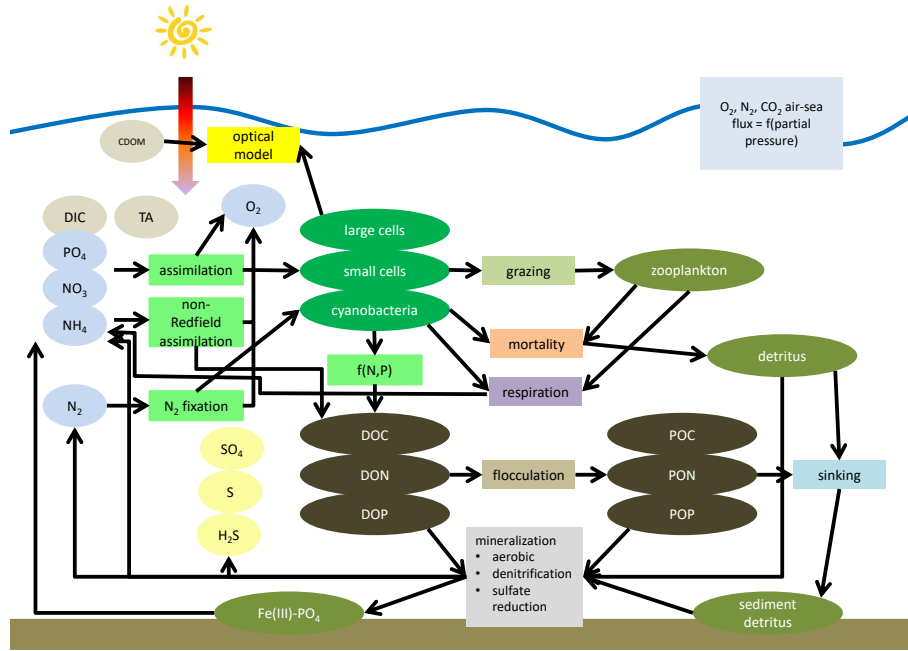
Figure 5. Simplified schematic of the ERGOM model. State variables are shown as ellipses and processes as rectangles. State variables are explained in Tab. 1. Arrows show fluxes of elements mediated by processes. Not all arrows are shown for simplicity of the schematic. E.g., oxygen demanding processes do not show arrows from the oxygen state variable.
