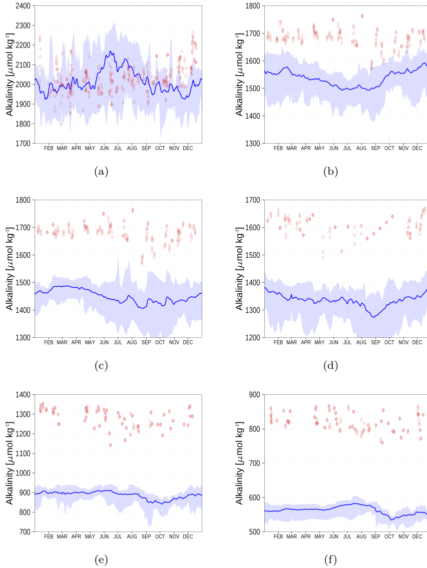
Figure 15. Surface alkalinity climatology (2013-2018) from Observations (red) and from model simulatuion (blue). Shaded areas show the range between 10th and 90th percentile. The subfigures represent stations AH (a), BY1 (b), BY15 (c), BY31 (d), C3 (e), and F9 (f) (Fig. 6). Observed alkalinity data are available from SHARK database (see code and data availability ).
