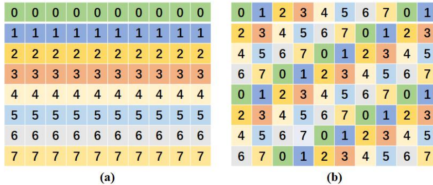
Figure 10. An example of two kinds of parallel decompositions. (a) Regular 2-D decomposition, with each process associated with one subdomain. (b) Round-robin-based decomposition associates each process with multiple subdomains.
