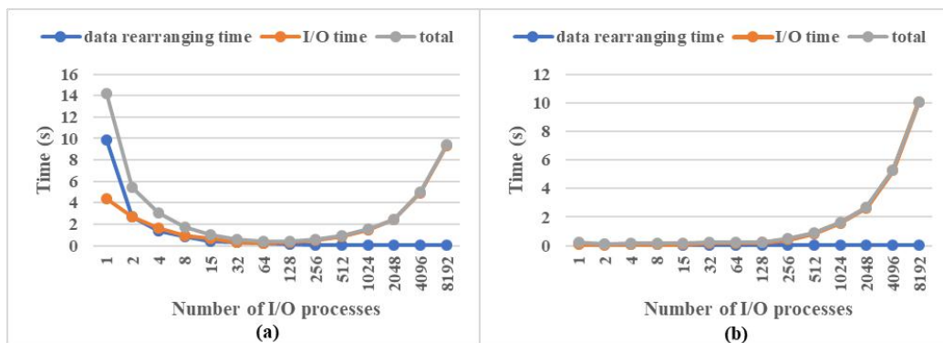
Figure 28. As Fig. 26, but for inputting a field.
