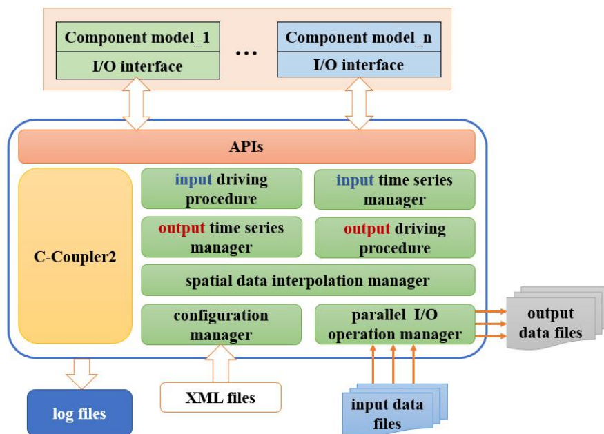
Figure 1. Architecture of CIOFC1.0.
