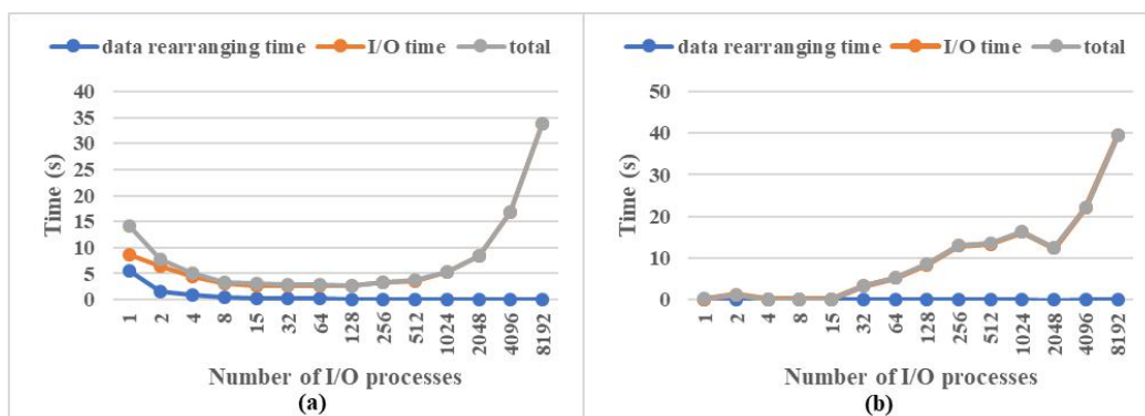
Figure 26. Time required for data rearranging, I/O, and the total time for outputting (a) a 3-D field and (b) a 2-D field at fine resolution. 10,048 processes were used to run the test model.
