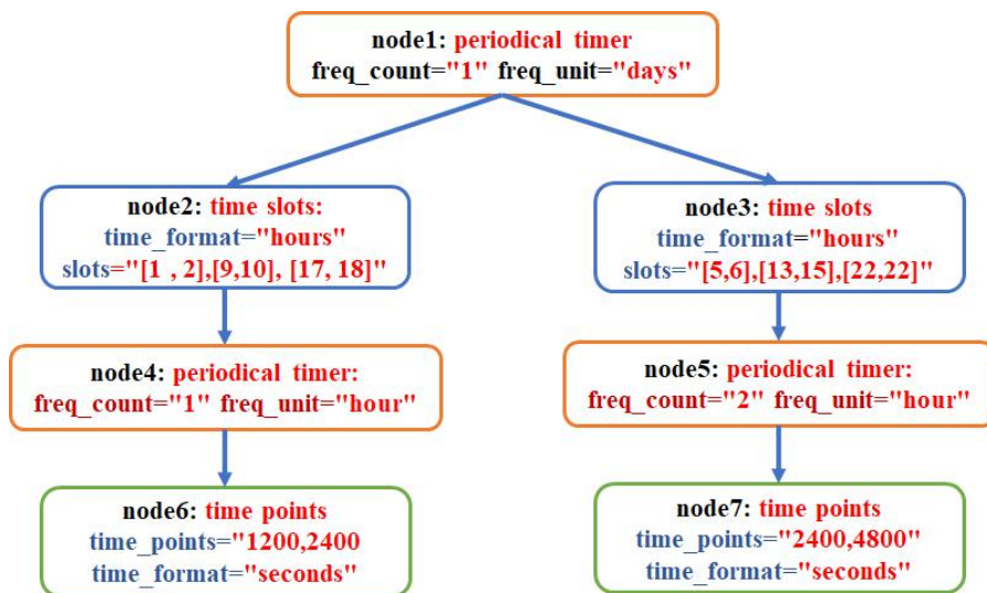
Figure 17. A visualization of the timer tree corresponding to the configuration in Fig. 12.
