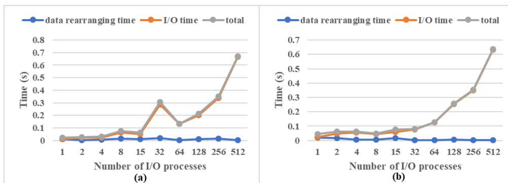
Figure 29. As Fig. 27, but for inputting a field.
