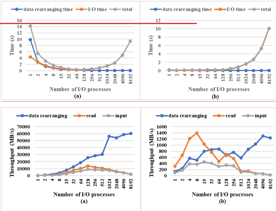
Figure 27. As Fig. 25, but for inputting a field.
