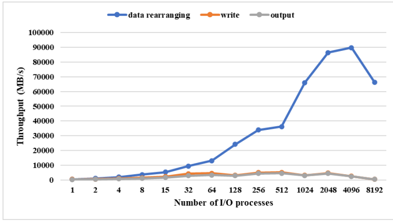
Figure 29. As The average throughput for outputting 100 3-D fields at fine resolution. 10,048 processes were used to run the test model. Fig-27, but for inputting a field.
