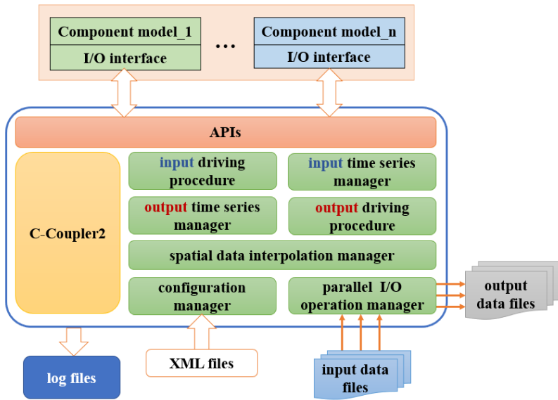
Figure 1. Architecture of CIOFCL0.
