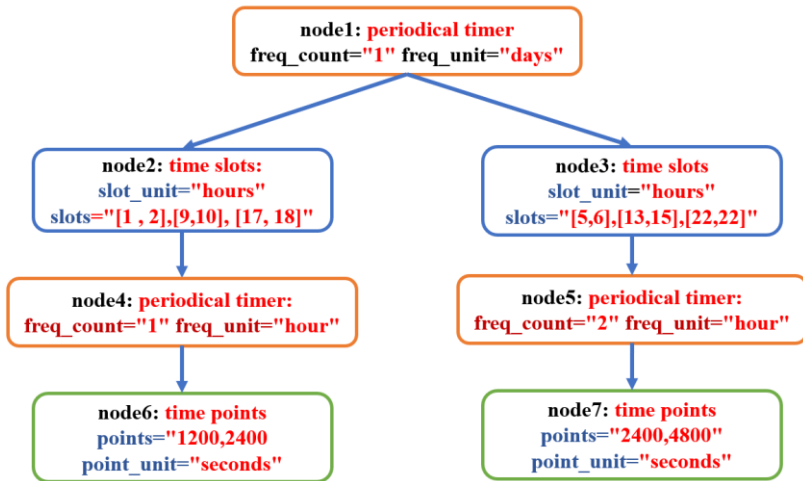
Figure 16. A visualization of the timer tree corresponding to the configuration in Fig. 1211.
