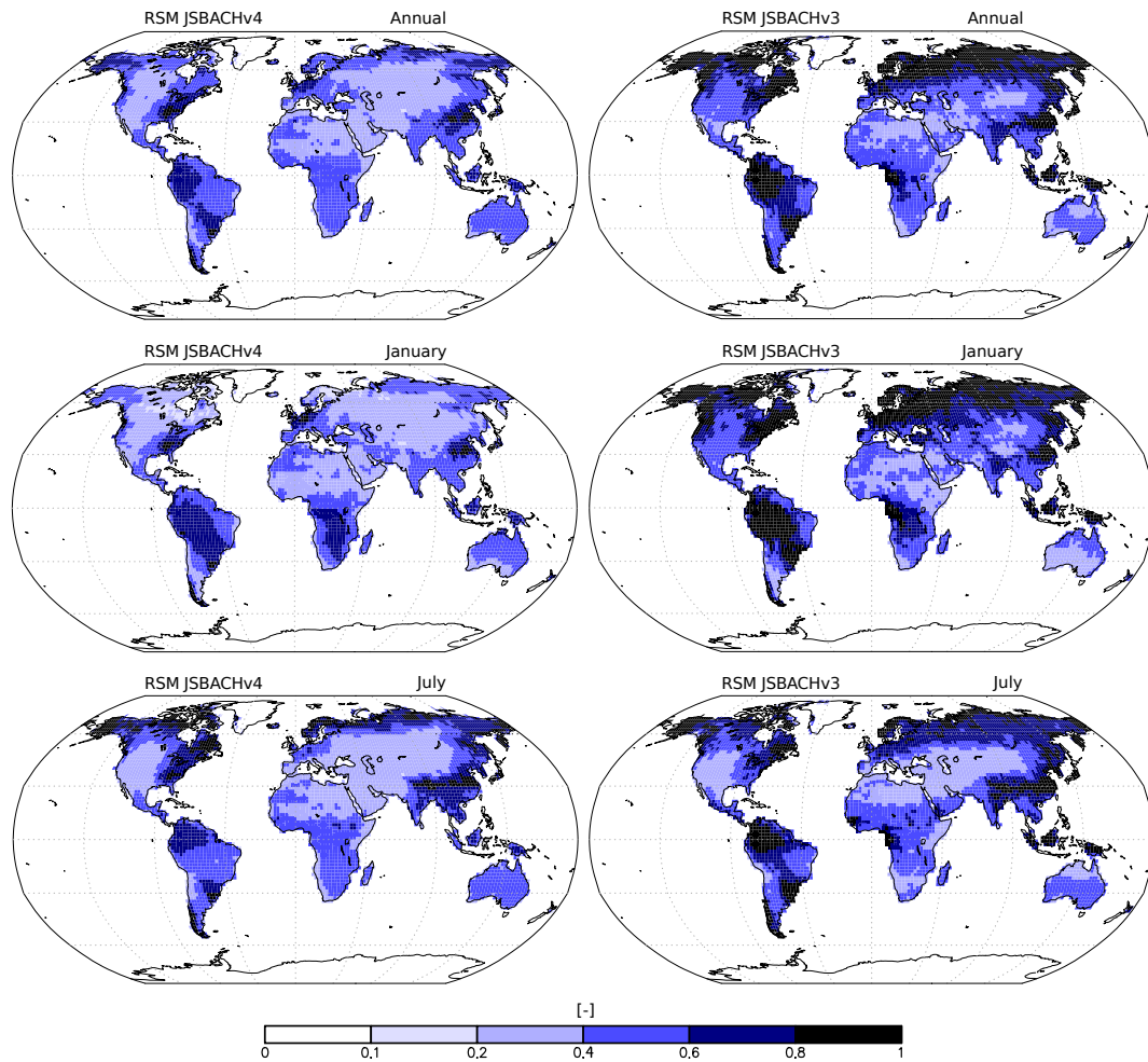
Figure 11. Relative Soil Moisture (RSM) in JSBACHv4 (left) and JSBACHv3 (right). Shown are the annual, January and July means over the years 2001 to 2014. RSM is calculated as the ratio between amount of soil water above wilting point and the amount of water between field capacity and wilting point. RSM thus characterizes the soil conditions concerning water stress of plants (the plant usable field capacity).
