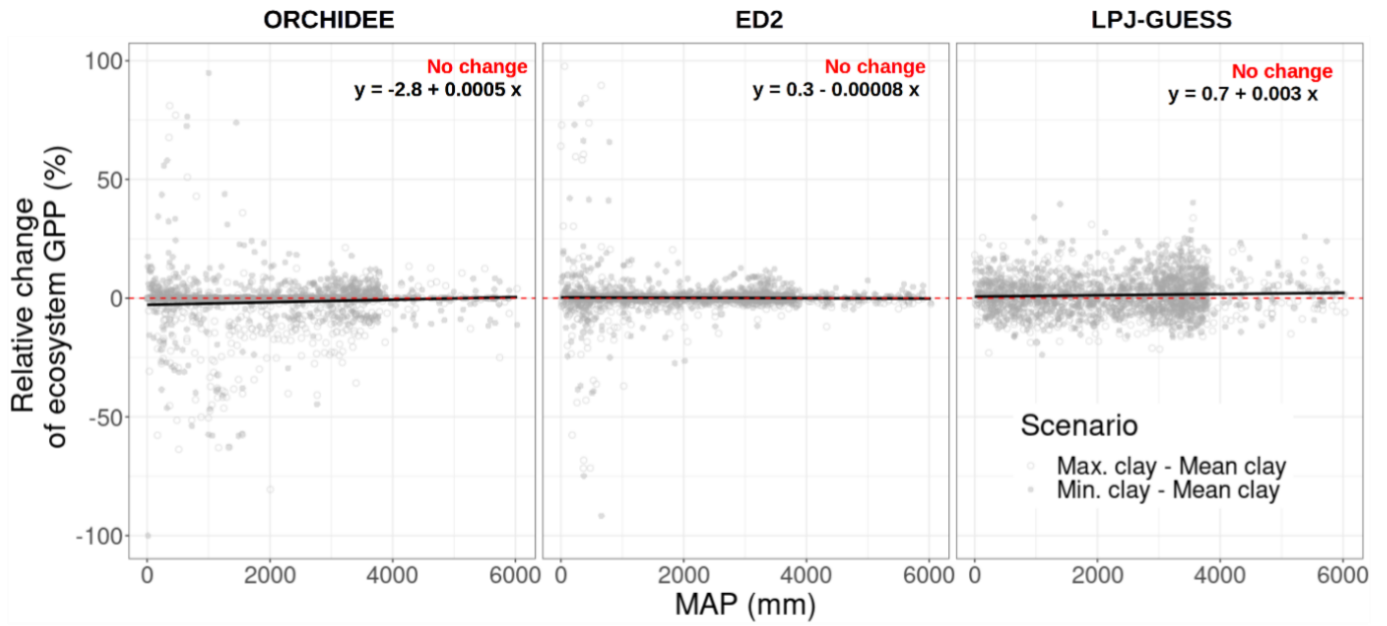
495 Figure 6: Relative change of the annual ecosystem GPP at the end of the historical simulation with the mean annual precipitation (MAP) for both scenarios (shapes) and all three TBMs considered in this study, across the entire simulated region (each point is a gridcell). The MAP is the annual average over the last ten years (2006-2016) of the CRU-NCEP dataset forcing. R^2 of all linear models were lower than 0.01.
