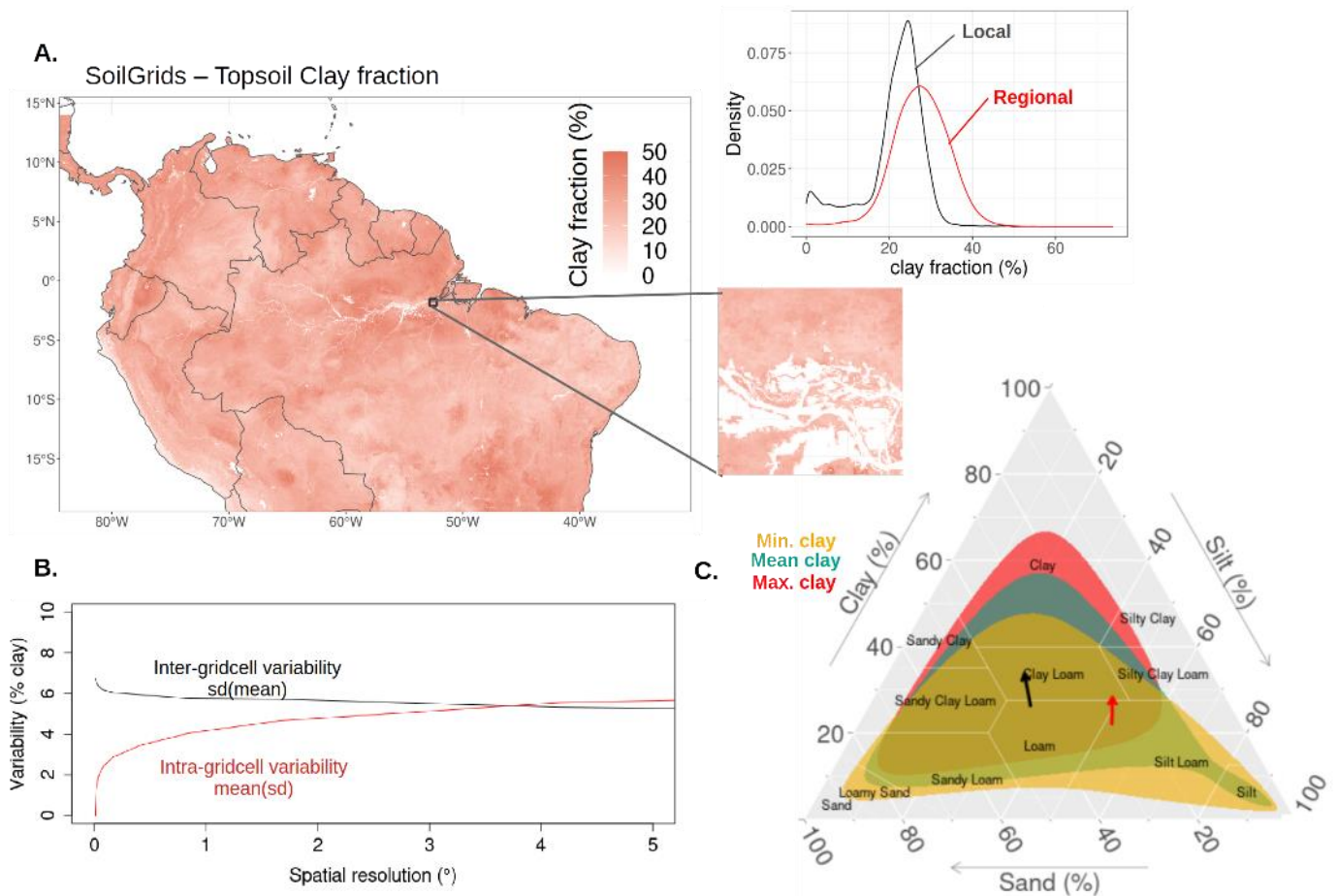
465 Figure 1: Topsoil (0-5cm) clay fraction spatial distribution as defined by the latest version of SoilGrids with a magnified example of a 1x1° gridcell (A). The Min., Mean, and Max. clay scenarios are those soil types that are characterised respectively by the minimum, average, and maximum clay fraction content in each gridcell, excluding those without soil textural information (for instance the rivers as illustrated in the magnified map). In panel A, the density plot reveals the clay fraction distribution at the regional and local (magnified gridcell) levels. Subplot B shows both the intra-gridcell (i.e. mean of the standard deviation (sd) of the clay content) and the inter-gridcell (the standard deviation (sd) of the mean clay content) variability as a function of the spatial resolution. Subplot C is the resulting soil texture distribution for each scenario. The arrows in subplot C show the average change of soil texture moving from the Min. clay to Mean clay scenario (black) and observed (red) changes in soil texture after deforestation (Eleftheriadis et al., 2018). 470
