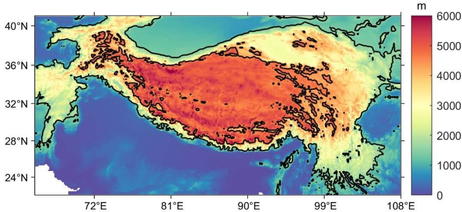
Figure 1: Spatial distribution of elevation and the contour lines of 1.5 and 4.5 km over the Tibetan Plateau.
