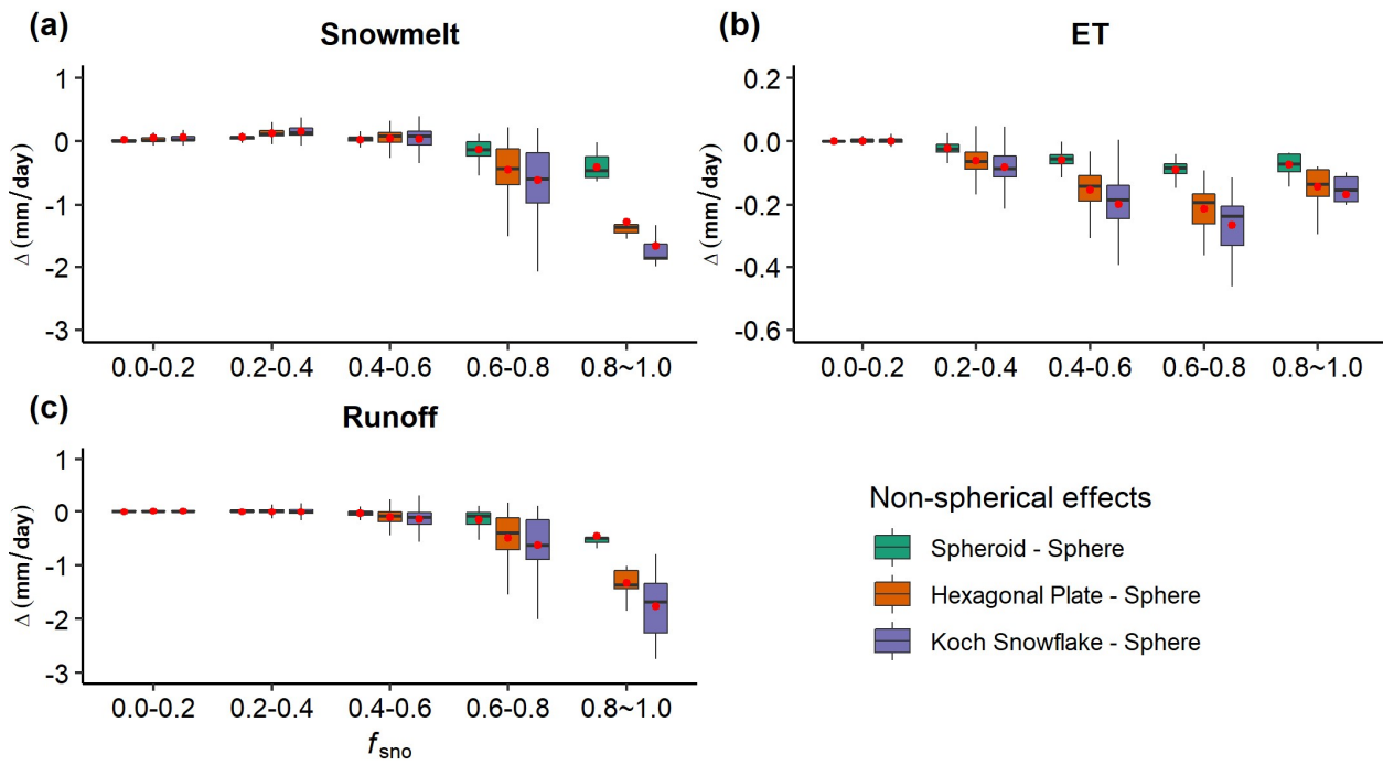
435 Figure 11: Same as Figure 10, except for hydrological terms: (a) snowmelt, (b) ET, and (c) runoff.
