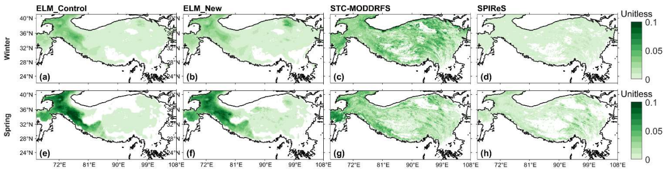
Figure 5: Spatial distributions of SAR estimated from: (a,e) ELM_Control, (b,f) ELM_New, (c,g) STC-MODSCAG/STC-MODDRFS and (d,h) SPIReS for winter (a-d) and spring (e-h). The areas with f_{sno} smaller than 0.01 are masked..
