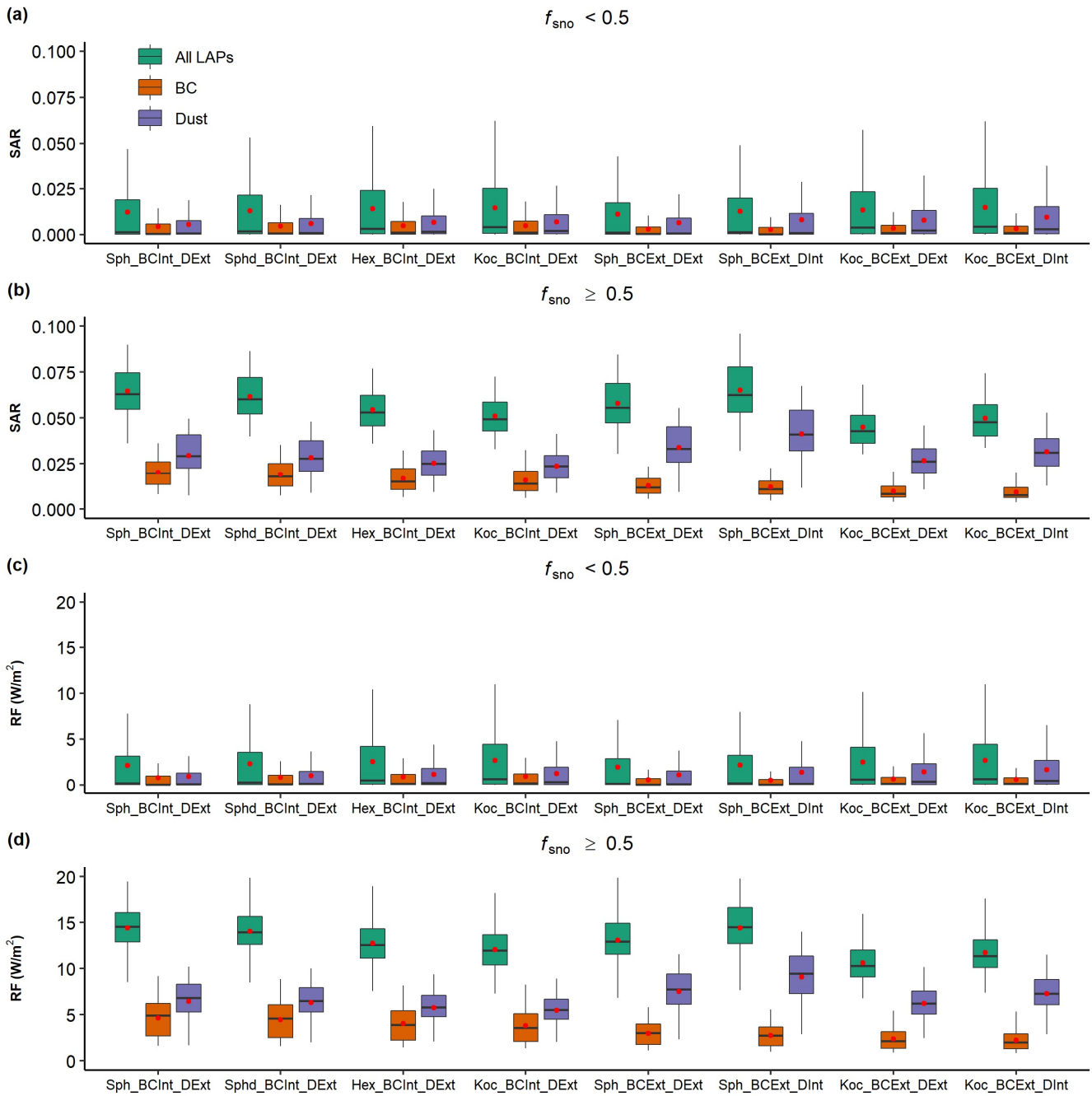
400 Figure 9: Boxplots of SAR (a-b) and RF (c-d) from all LAPs, BC, and dust for different f_{sno} values: (a,c) < 0.5 and (b,d) \geq 0.5 in spring under different cases listed in Table 1. For the case ID labelled in x-axis, the ‘_PP’ suffix is omitted to keep them simplified. Red circles represent the mean values. The corresponding results for winter are shown in Figure S7.
