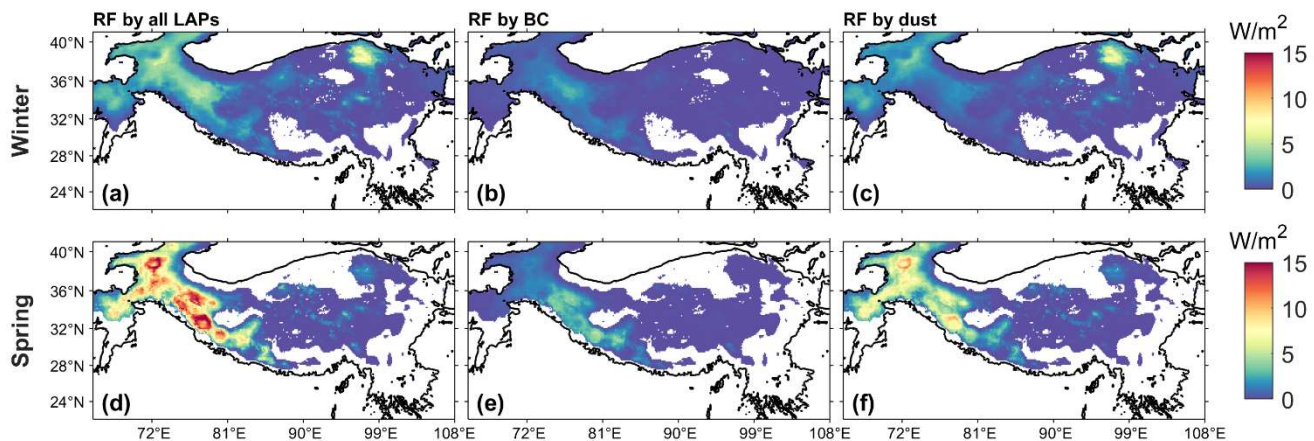
350 Figure 6. Spatial distributions of RF values from (a,d) all LAPs (BC+dust), (b,e) BC and (c,f) dust for (a-c) winter and (d-f) spring in ELM_New. The areas with f_{sno} smaller than 0.01 are masked.
