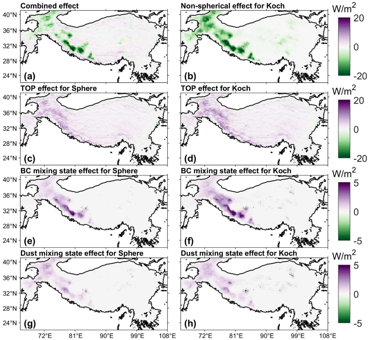
455 Figure 12: Spatial distributions of the change of net solar radiation ( R_{net}^S ) contributed by individual influencing factors and their combined effects in spring, which are derived based on Table 2. The corresponding results in winter are shown in Figure S14.
