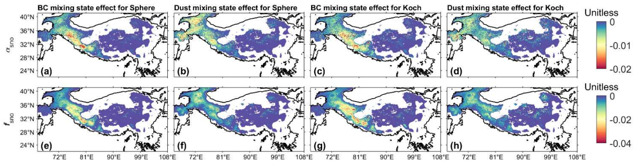
395 Figure 8: The differences in \alpha_{sno} (a-d) and f_{sno} (e-h) between different mixing states (internal - external) of snow-LAP: (a,e) BC (sphere), (b,f) dust (sphere), (c,g) BC (Koch snowflake) and (d,h) dust (Koch snowflake) for spring. Here the differences between internal and external mixing are negative. The specific calculation methods are listed in Table 2. The corresponding results for winter are shown in Figure S6. The areas with f_{sno} smaller than 0.01 are masked.
