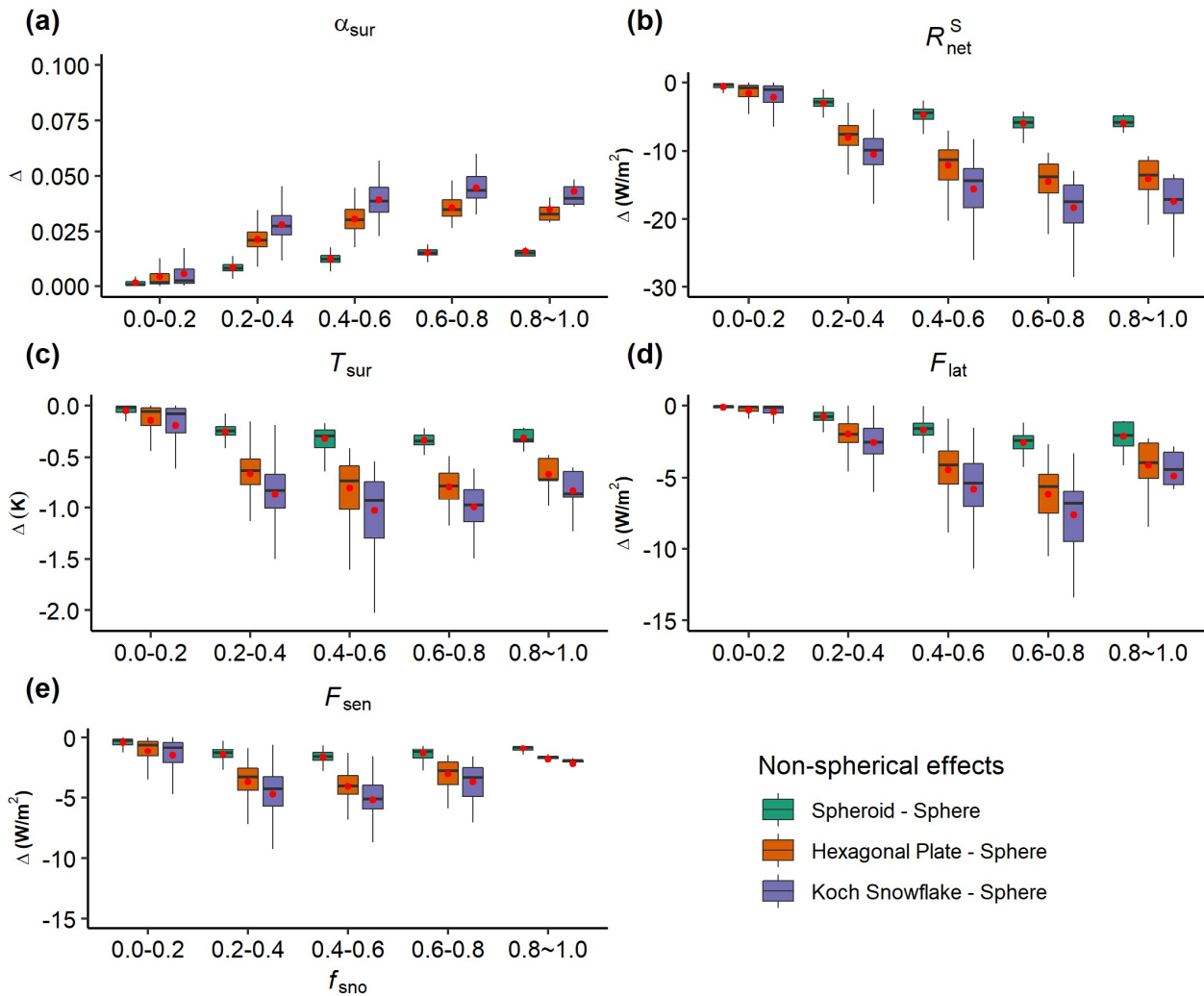
420 Figure 10: The boxplots of the differences ( \Delta ) in surface energy budget terms: (a) surface albedo ( \alpha_{sur} ), (b) net solar radiation ( R_{net}^S ), (c) surface temperature ( T_{sur} ), (d) latent heat flux ( F_{lat} ) and (e) sensible heat flux ( F_{sen} ), between different snow grain shapes: spheroid – sphere, hexagonal plate – sphere and Koch snowflake – sphere under different snow cover fractions ( f_{sno} ) for spring. See Table 2 for the specific calculation methods.
