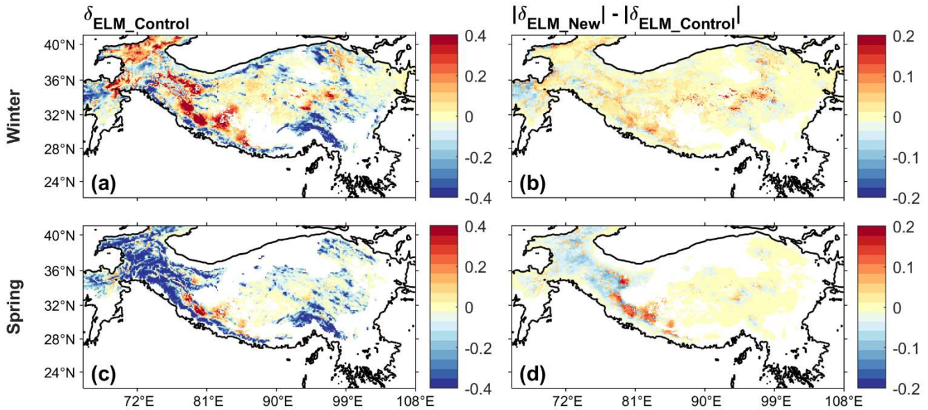
310 Figure 2: (a,c) The f_{sno} bias ( \delta_{ELM\_Control} ) of ELM_Control compared to the mean value of STC-MODSCAG and SPIReS, and (b,d) the difference ( |\delta_{ELM\_New}| - |\delta_{ELM\_Control}| ) between the absolute values of the biases of ELM_New ( \delta_{ELM\_New} ) and ELM_Control ( \delta_{ELM\_Control} ) for winter (a-b) and spring (c-d). The negative values (blue color) in (b,d) show that ELM_New has the smaller bias than ELM_Control. The areas with f_{sno} smaller than 0.01 are masked.
