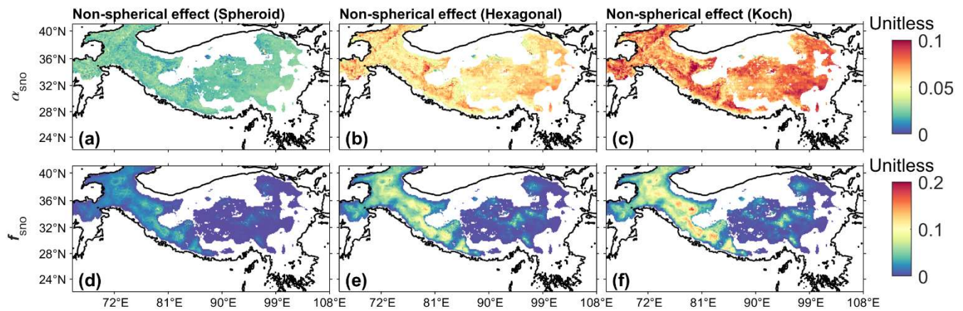
Figure 7: The differences in \alpha_{\text{sno}} (a-c) and f_{\text{sno}} (d-f) between different snow grain shapes: (a,d) spheroid - sphere, (b,e) hexagonal plate - sphere and (c,f) Koch snowflake - sphere, for spring. Here the differences between non-spherical and spherical grain shapes are positive. The specific calculation methods are listed in Table 2. The areas with f_{\text{sno}} smaller than 0.01 are masked.
