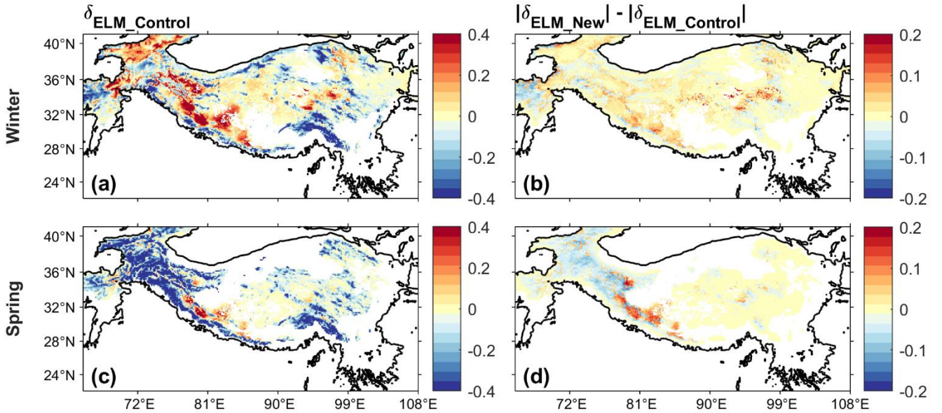
310 Figure 2: (a,c) The f_{\text{sno}} bias ( \delta_{\text{ELM\_Control}} ) of ELM_Control compared to the mean value of STC-MODSCAG and SPIReS, and (b,d) the difference ( |\delta_{\text{ELM\_New}}| - |\delta_{\text{ELM\_Control}}| ) between the absolute values of the biases of ELM_New ( \delta_{\text{ELM\_New}} ) and ELM_Control ( \delta_{\text{ELM\_Control}} ) for winter (a-b) and spring (c-d). The negative values (blue color) in (b,d) show that ELM_New has the smaller bias than ELM_Control. The areas with f_{\text{sno}} smaller than 0.01 are masked.
