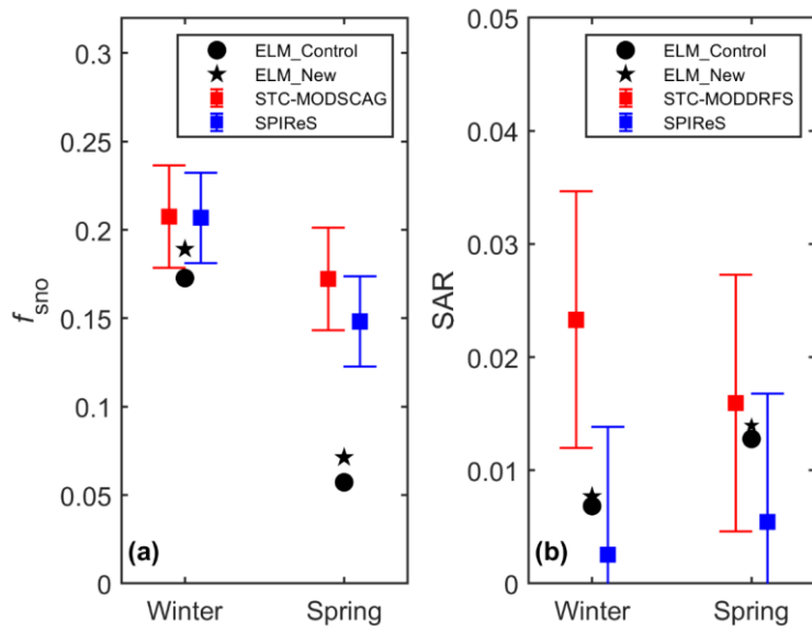
[340] Figure 4: The area-weighted average of (a) f_{sno} and (b) SAR induced by LAPs for winter and spring from ELM, STC-MODSCAG/STC-MODDRFS, and SPIReS. The bar width represents the uncertainty bounds of STC-MODSCAG and SPIReS from Bair et al., (2021a).
