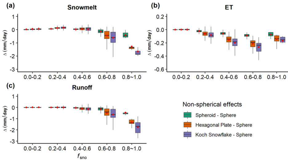
Figure 12: Same as Figure 11, except for hydrological terms: (a) snowmelt, (b) ET, and (c) runoff.
