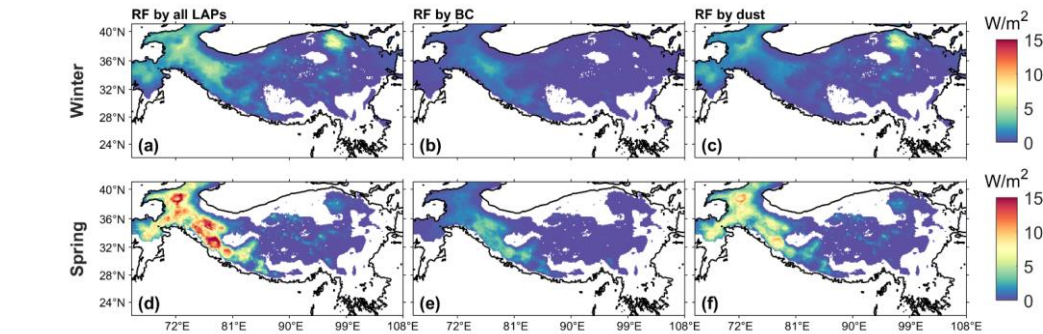
375 Figure 7. Spatial distributions of RF values from (a,d) all LAPs (BC+dust), (b,e) BC and (c,f) dust for (a-c) winter and (d-f) spring in ELM_New. The areas with f_{sno} smaller than 0.01 are masked.
