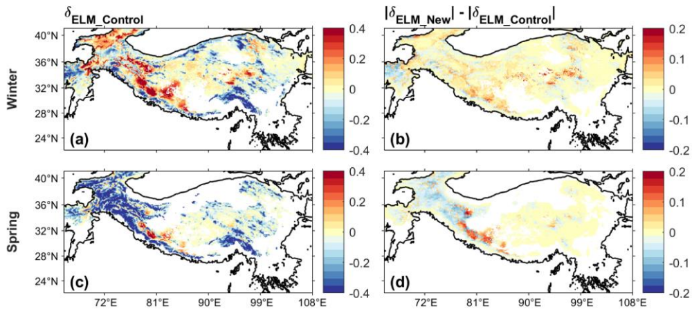
Figure 3: (a,c) The f_{sno} bias ( \delta_{ELM\_Control} ) of ELM_Control compared to the mean value of STC-MODSCAG and SPIReS, and (b,d) the difference ( |\delta_{ELM\_New}| - |\delta_{ELM\_Control}| ) between the absolute values of the biases of ELM_New ( \delta_{ELM\_New} ) and ELM_Control ( \delta_{ELM\_Control} ) for winter (a-b) and spring (c-d). The negative values (blue color) in (b,d) show that ELM_New has the smaller bias than ELM_Control. The areas with f_{sno} smaller than 0.01 are masked.
