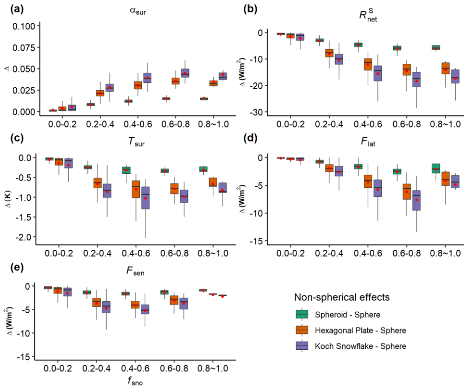
475 Figure 11: The boxplots of the differences ( \Delta ) in surface energy budget terms: (a) surface albedo ( \alpha_{sur} ), (b) net solar radiation ( R_{net}^S ), (c) surface temperature ( T_{sur} ), (d) latent heat flux ( F_{lat} ) and (e) sensible heat flux ( F_{sen} ), between different snow grain shapes: spheroid – sphere, hexagonal plate – sphere and Koch snowflake – sphere under different snow cover fractions ( f_{sno} ) for spring. See Table 2 for the specific calculation methods.
