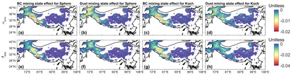
Figure 9: The differences in \alpha_{\text{sno}} (a-d) and f_{\text{sno}} (e-h) between different mixing states (internal - external) of snow-LAP: (a,e) BC (sphere), (b,f) dust (sphere), (c,g) BC (Koch snowflake) and (d,h) dust (Koch snowflake) for spring. Here the differences between internal and external mixing are negative. The specific calculation methods are listed in Table 2. The corresponding results for winter are shown in Figure S5. The areas with f_{\text{sno}} smaller than 0.01 are masked.
