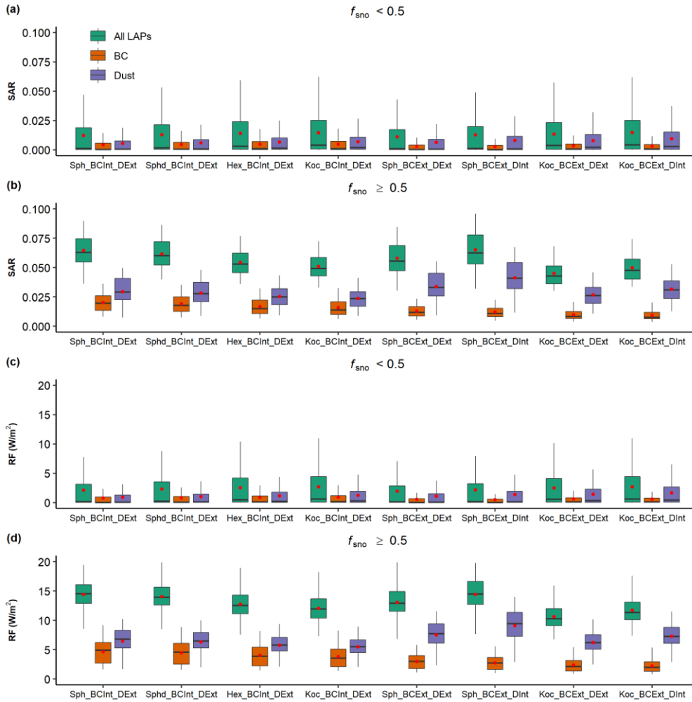
440 Figure 10: Boxplots of SAR (a-b) and RF (c-d) from all LAPs, BC, and dust for different f_{sno} values: (a,c) <0.5 and (b,d) \geq 0.5 in spring under different cases listed in Table 1. For the case ID labelled in x-axis, the ‘_PP’ suffix is omitted to keep them simplified. Red circles represent the mean values. The corresponding results for winter are shown in Figure S6.
