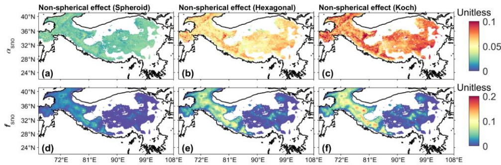
Figure 8: The differences in \alpha_{\text{sno}} (a-c) and f_{\text{sno}} (d-f) between different snow grain shapes: (a,d) spheroid - sphere, (b,e) hexagonal plate - sphere and (c,f) Koch snowflake - sphere, for spring. Here the differences between non-spherical and spherical grain shapes are positive. The specific calculation methods are listed in Table 2. The areas with f_{\text{sno}} smaller than 0.01 are masked.
