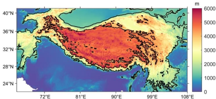
Figure 2: Spatial distribution of elevation and the contour lines of 1.5 and 4.5 km over the Tibetan Plateau.
