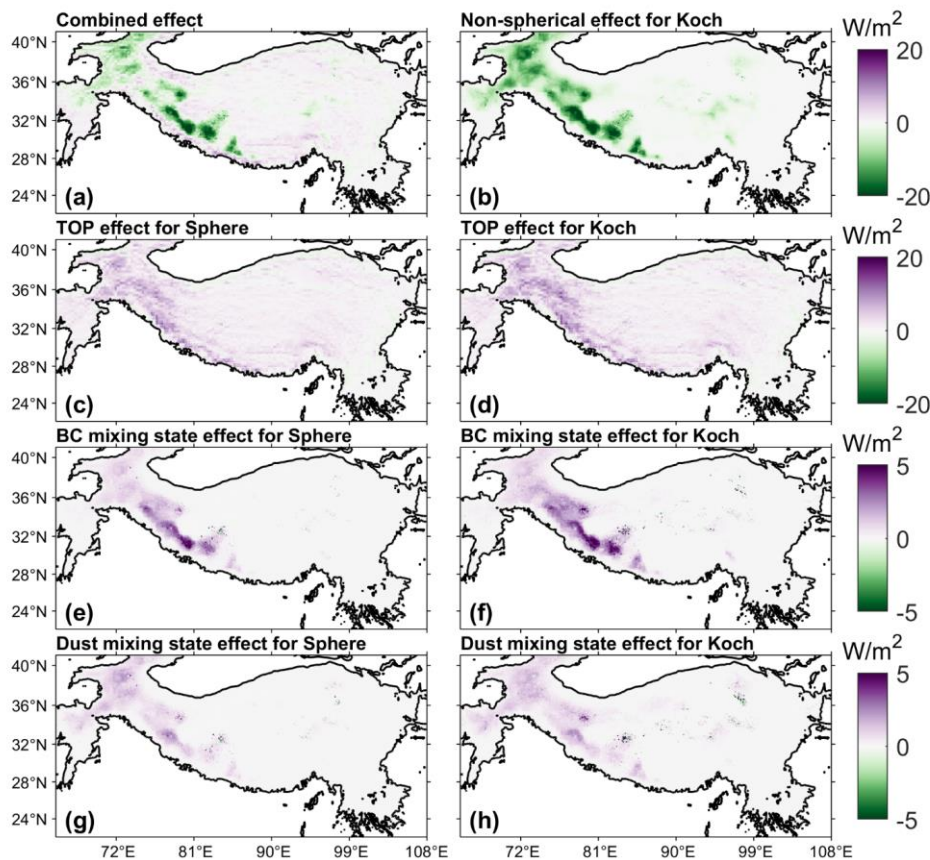
Figure 13: Spatial distributions of the change of net solar radiation ( R_{net}^s ) contributed by individual influencing factors and their combined effects in spring, which are derived based on Table 2. The corresponding results in winter are shown in Figure S13.
