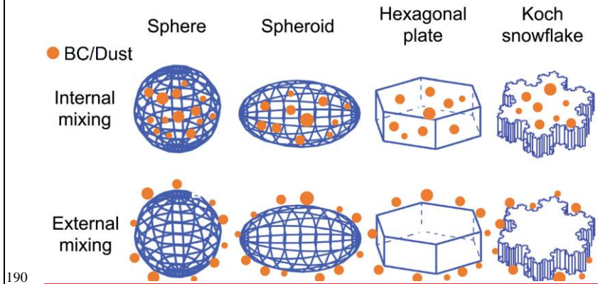
190 Figure 1: Schematics of four typical snow grain shapes: sphere, spheroid, hexagonal plate and Koch snowflake, and two different mixing states of BC-snow or dust-snow: internal and external. This figure is adapted from (He et al., 2019).
