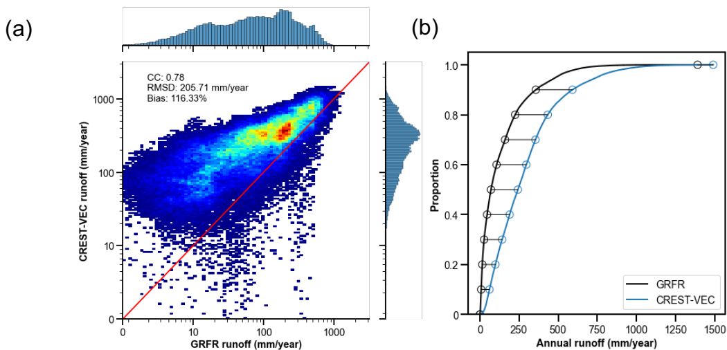
Supplementary Figure 1. (a) density plot of CREST-VEC simulated annual surface runoff against GRFR (Global Reach-level Flood Reanalysis) in the Great Plains; (b) cumulative density function (CDF) of CREST-VEC and GRFR simulated annual runoff.
