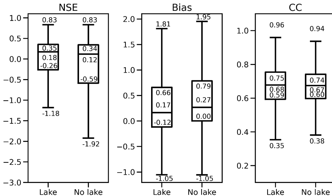
Figure 5. Boxplot of model performance (NSE, Bias, and CC) comparing results with lake routing and without it. The numbers for each box represent first quartile minus 1.5 times interquartile range, first quartile, median, third quartile, and third quartile plus 1.5 times interquartile range.
