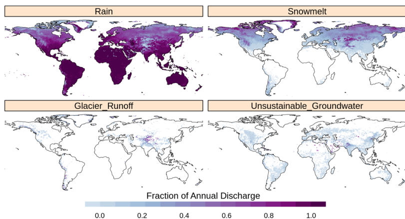
Figure 7. The fraction of annual average discharge composed of the four different primary source water components used in the primary source tracking method.
