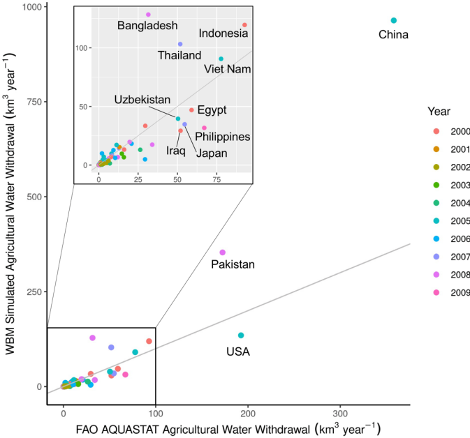
Figure 6. WBM-simulated irrigation water withdrawals compared to FAO AQUASTAT-reported values, by country. The 1:1 line is shown in grey. Countries with FAO-reported agricultural water withdrawals < 100 km³ year⁻¹ are shown in the inset. Countries with FAO-reported agricultural water withdrawals > 50 km³ year⁻¹ are labeled.
