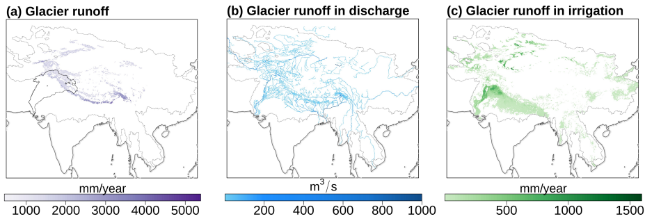
985 Figure 9. Tracking glacier runoff (a) downstream through rivers (b) and irrigation water use (c) in High Mountain Asia, a region where glacier meltwater is an important resource. While glacier water originates in the mountains, its' use in agriculture is extensive due to reuse through the river network and shallow groundwater stores, and retention in and distribution from large reservoirs. The boundary of all High Mountain Asia basins with glaciers at their headwaters is shown in grey. Panel (a) also shows the Indus basin boundaries for reference in comparing with Figure 10. 990
