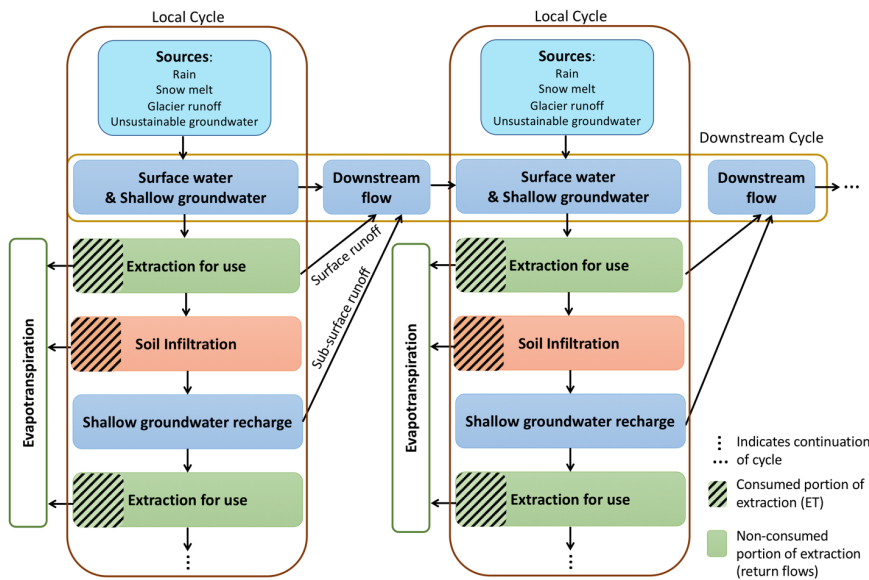
Figure 2: Primary source component tracking schematic. All surface and shallow groundwater is composed of the four primary sources: rain, snow melt, glacier runoff, and unsustainable groundwater. When surface and/or shallow groundwater is extracted for use, this initiates both a local cycle and a downstream cycle of water use and re-use. In the example shown here, water is extracted and applied to soils (irrigation). A portion of the extracted water and a portion of the soil water becomes evapotranspiration (the consumed portion, shown with hashes). Some of the water applied to soils percolates to the shallow groundwater pool. Water from the shallow groundwater pool can be extracted again, continuing the local water re-use cycle. Water extracted for use, and water from the shallow groundwater pool, generate runoff that moves downstream. This initiates a downstream cycle in which this water can be re-extracted for use from the surface water system. Downstream cycles intersect with local cycles, as water from the four primary sources are input in every locality. Figure modified from Grogan et al. (2017).
