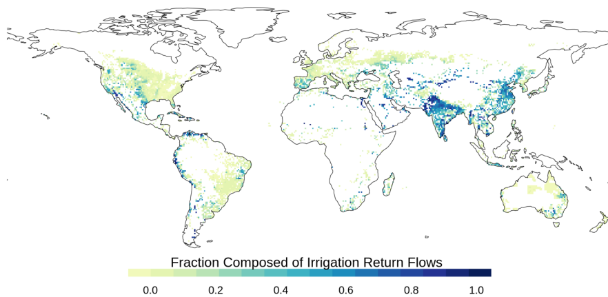
Figure 11. Fraction of average annual discharge composed of irrigation return flow water, simulated by the return flow tracking function. The large fraction of irrigation return flows in northern India and Pakistan results from this region being one of the most intensively irrigated regions in the world, combined with very low (~30%) classical irrigation efficiency (Zaveri et al., 2016; Grogan et al., 2017). This combination means that large volumes of water are extracted for irrigation, and nearly two-thirds of that water returns to the system.
