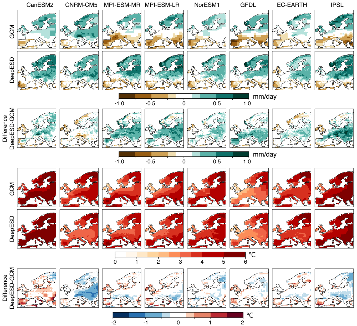
Figure 5. The climate change signals (2071-2100 with respect to 1975-2005) of the eight CMIP5 climate models considered and the equivalent DeepESD downscaled fields for precipitation (rows 1-2) and temperature (rows 4-5). Rows 3 and 6 show the difference between the DeepESD downscaled and raw climate change signals for the different GCMs
