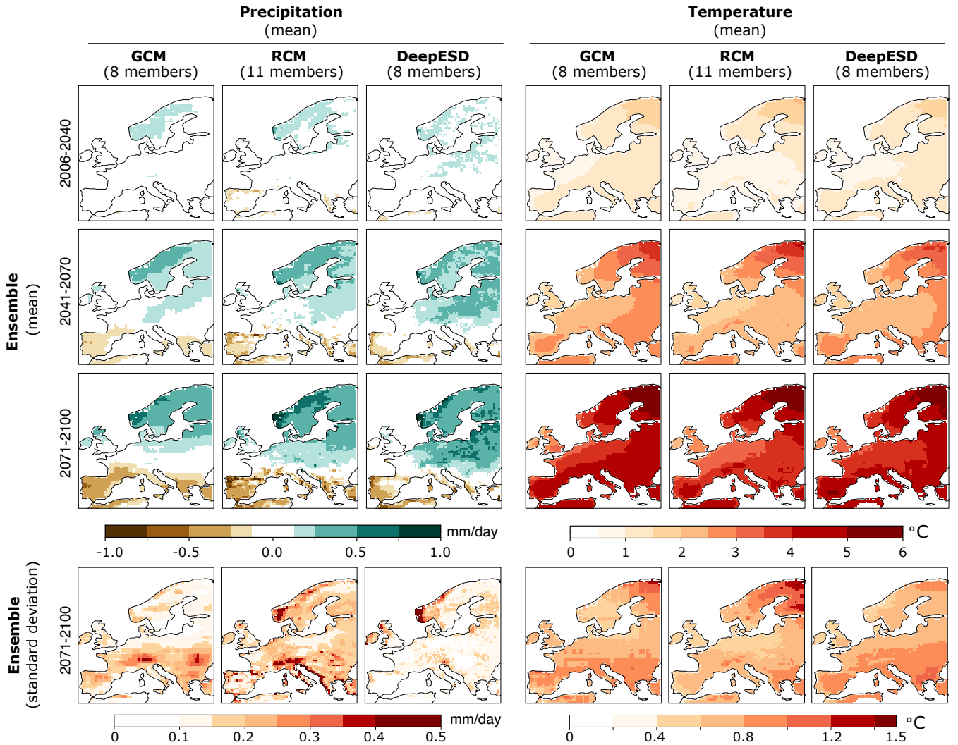
Figure 4. Climate change signal for annual mean precipitation (left) and temperature (right) for near- (2006-2040), mid- (2041-2070) and far-future (2071-2100) periods, in rows, relative to 1975-2005 as projected by the GCM, RCM and DeepESD ensembles (in columns). The last row shows the uncertainty of the far-future signal, as measured by the standard deviation of the results across models.
