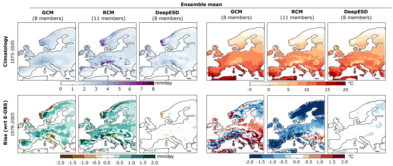
Figure 2. Annual daily precipitation (left block) and temperature (right) for the historical period 1975-2005, as obtained from the ensembles of GCMs, RCMs and DeepESD GCM-downscaled results (left, middle and right columns, respectively). The first row shows the ensemble mean climatological values and the second row displays the corresponding biases with respect to E-OBS v20.
