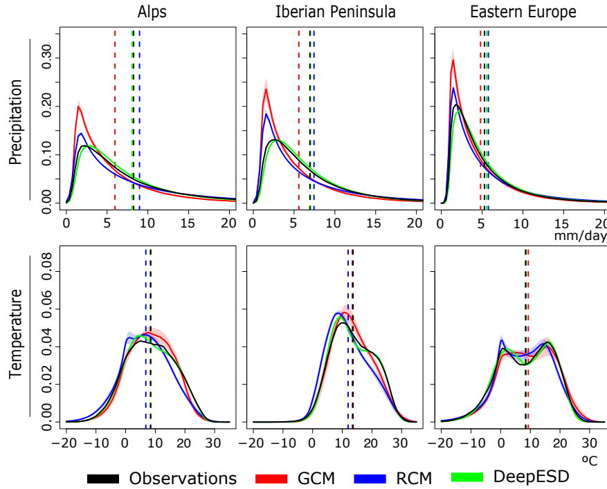
Figure 3. Probability Density Functions (PDFs) of the GCM (red), RCM (blue) and DeepESD (green) ensembles of precipitation and temperature over the historical period 1979-2005, plus E-OBS (black) for the Alps, the Iberian Peninsula and Eastern Europe as defined in the PRUDENCE regions (Christensen and Christensen, 2007). The solid line represents the ensemble mean and the shadow encompass two standard deviations. The dashed line indicates the distributional mean of each PDF.
