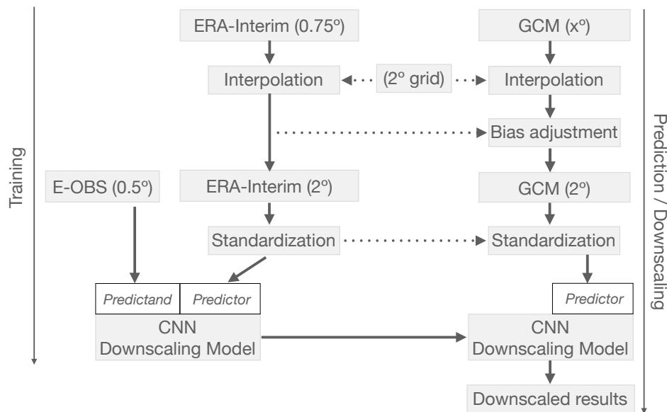
Figure 1. Workflow of pre-processing steps applied to reanalysis and GCM data in this work.
