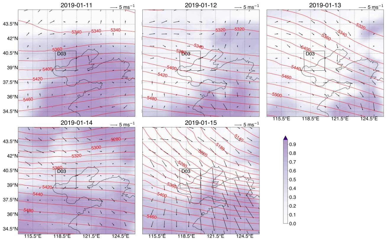
660 Figure 2: The daily averaged geopotential height (contour lines, units: gpm) at 500 hPa, total cloud fraction (shading) and surface winds at 10 meters (vectors, units: m/s) from ERA5 during 11 to 15 January 2019, the box indicates the D03 domain in Figure 1.
