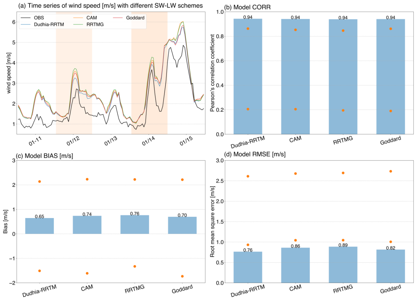
Figure 7: Same as Figure 3, but for the radiation schemes.
