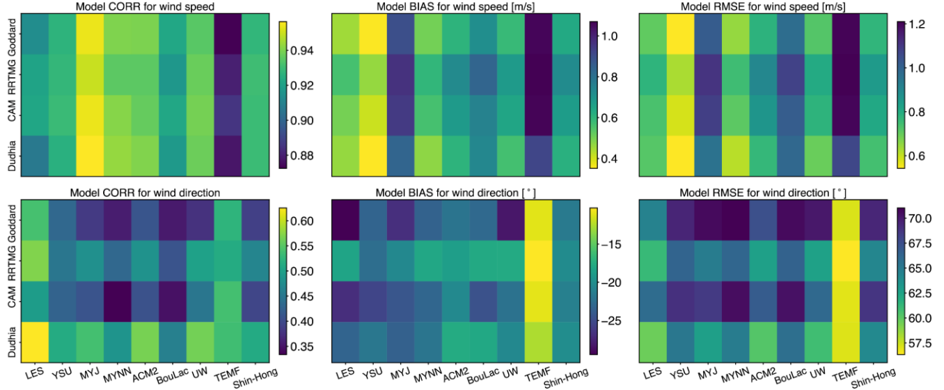
Figure 9: Statistic scores (CORR, BIAS and RMSE) for wind speed and direction for different combinations of PBL and SW-LW radiation schemes. (The MP schemes used in (a) and (b) are MYDM7 and P3, respectively. Dudhia represents Dudhia-RRTM SW-LW schemes in all the subplots.
