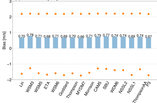
(c) Model BIAS [m/s]
