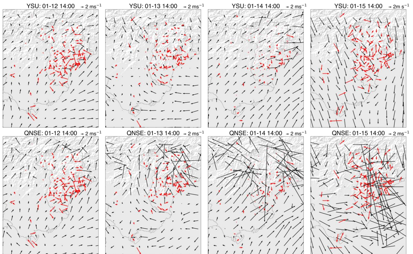
810 Figure 13: Spatial distribution of simulated (black vector) and observed (red vector) winds at 14:00 (in local time) during the study period from simulations with the YSU and QNSE schemes, the shading indicates the elevation, and the height of the wind is 10 meters.
