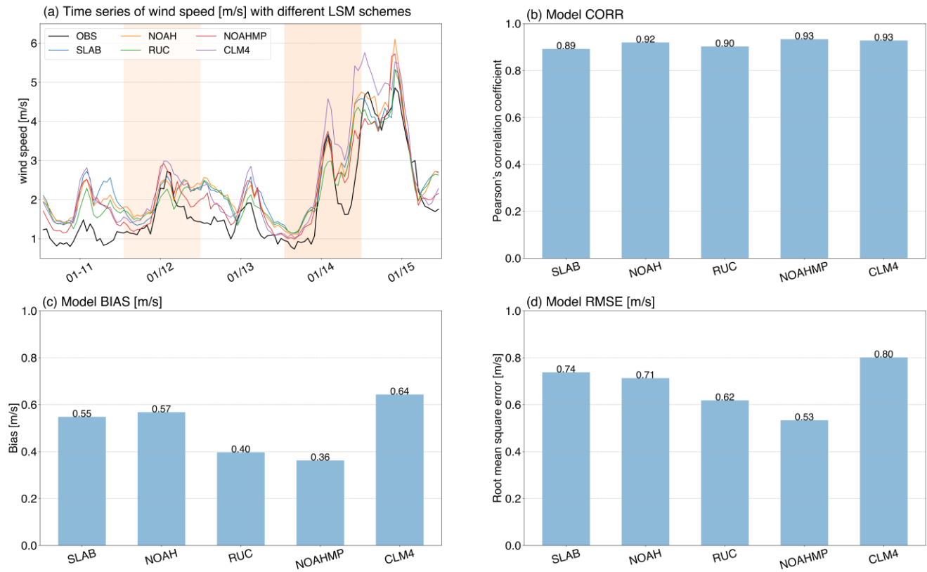
Figure 156: Same as Figure 3, but for simulations with different land surface schemes, the PBL, MP and SW-LW schemes used are the same as the simulation with best Taylor skill score (WDM6 in Figure 10).
