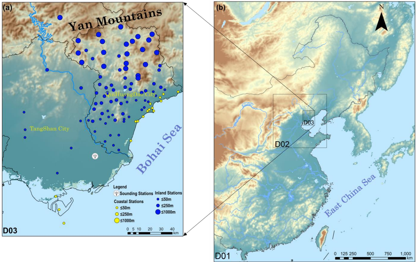
Figure 1: Map showing the (a) study area and (b) WRF nested domains (D01–D03). Solid yellow and blue circles and triangles in (a) represent coastal (16 stations in total) and inland stations (89 stations in total), the size of circles represents the station elevations , and white circlegreen triangle represent the sounding station.
