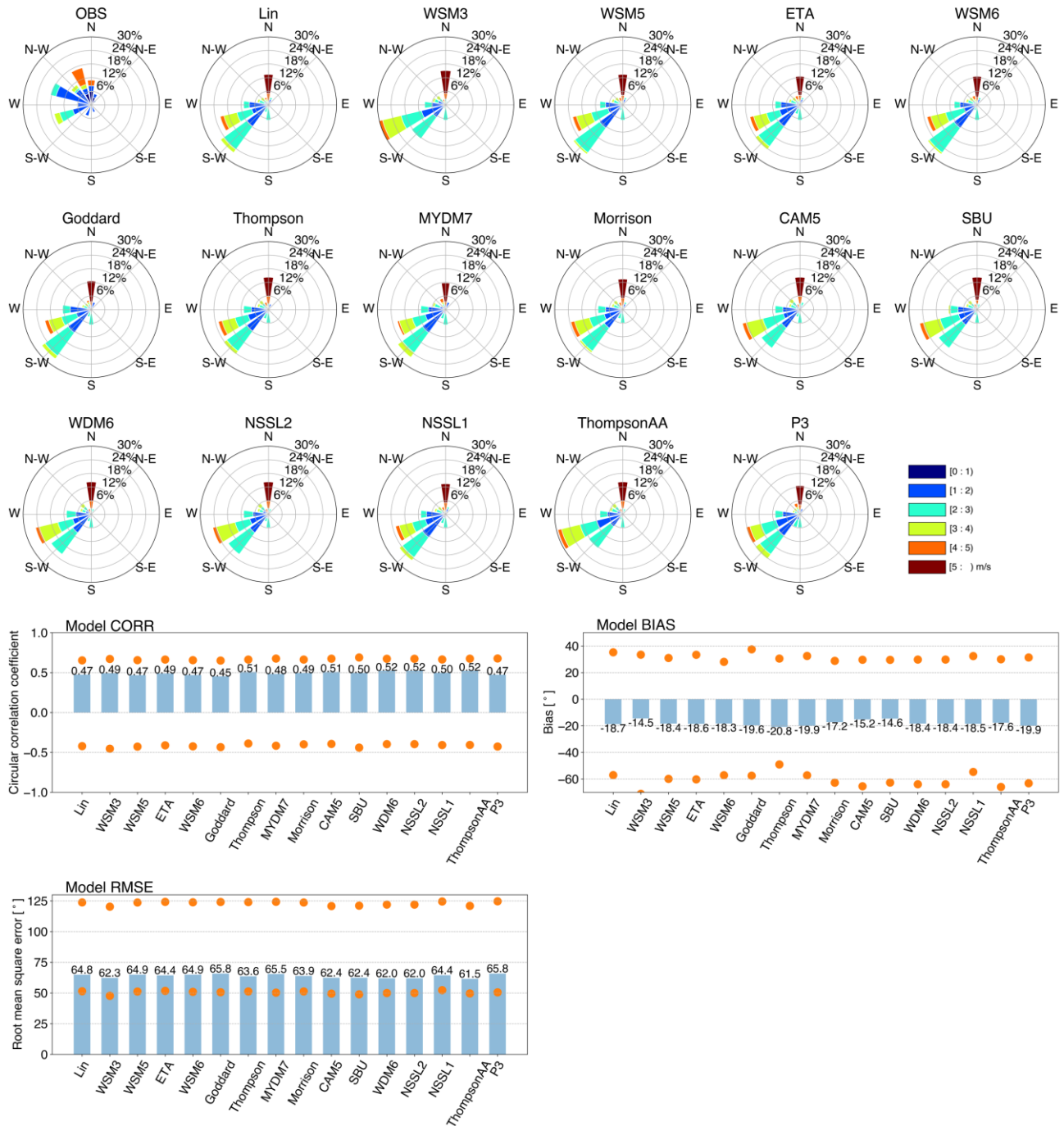
Figure 6: Same as Figure 4, but for the MP schemes.
