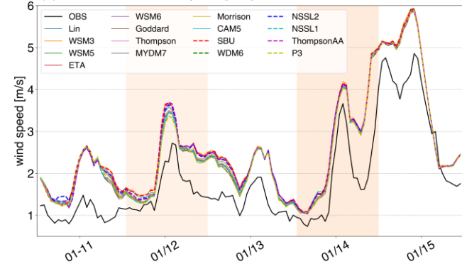
(a) Time series of wind speed [m/s] with different MP schemes
