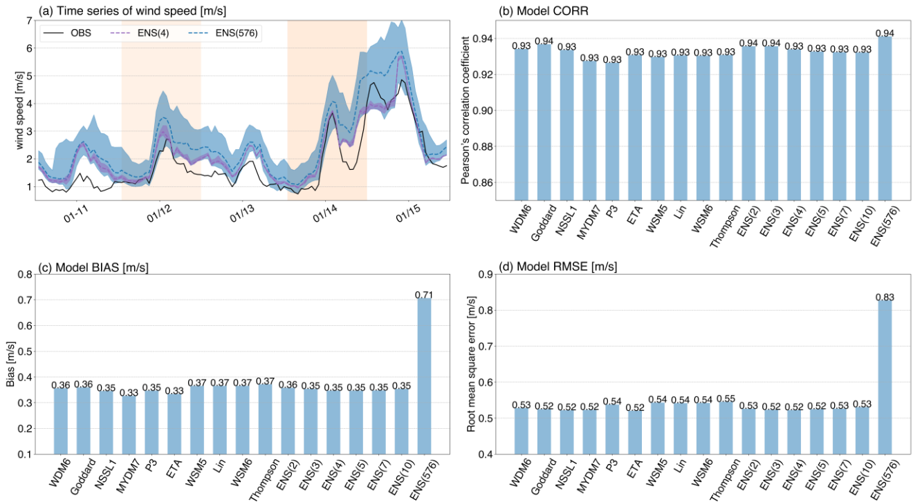
Figure 10: (a) Time series of wind speed (m/s) from observation and different ensembles, shading shows the spread, and the corresponding (b) CORR, (c) BIAS and (d) RMSE scores for the best 10 simulations along with different ensembles, are shown in b-d. The shading in a shows the spread for ENS(4) and ENS(576). As the best 10 simulations use the same PBL (YSU) and SW-LW (Dudhia-RRTM) schemes, only the MP schemes are labeled in the figure.
