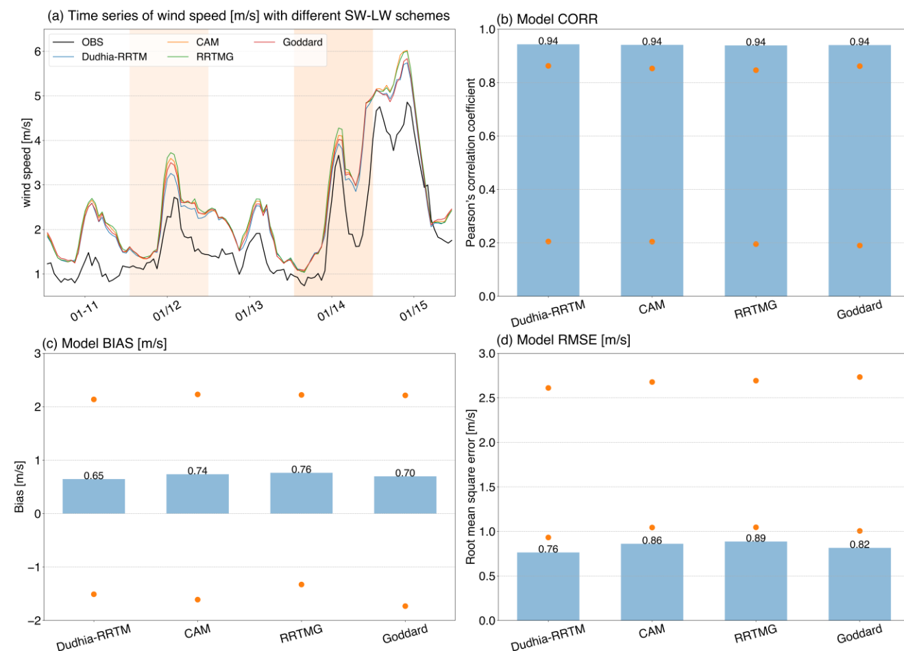
780 Figure 7: Same as Figure 3, but for the radiation schemes.
