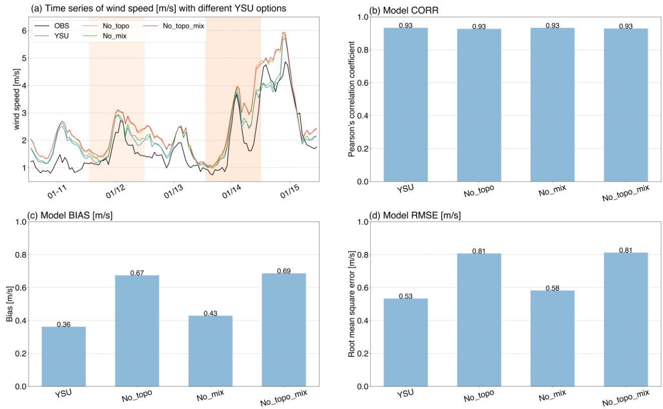
Figure 17 Same as Figure 3, but for simulations with different YSU options.
