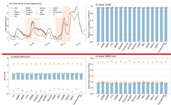
(a) Time series of wind speed [m/s] with different MP schemes
