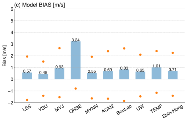
760 Figure 3: (a) Time series of observed and simulated wind speeds (m/s) and the corresponding statistics of (b) CORR, (c) BIAS and (d) RMSE for the PBL schemes. In a, the frequency of wind speed is hourly, and the tick marks in x-axis indicate 12:00 in local time of that day, For each PBL scheme, the average is calculated over the 105 stations and then over all the simulations with that scheme; the dots in b, c and d represent the range across the stations, fo-
