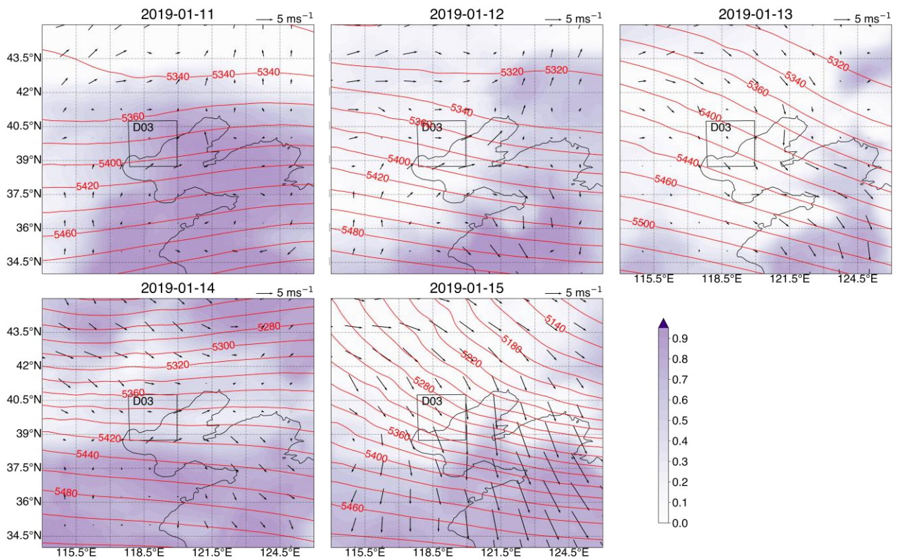
Figure 2: The daily averaged geopotential height (contour lines, units: gpm) at 500 hPa, total cloud fraction (shading) and surface winds at 10 meters (vectors, units: m/s) from ERA5 and cloud fraction (shading, units: %) at 925 hPa during 11 to 15 January 2019, the box indicates the D03 domain in Figure 1.
