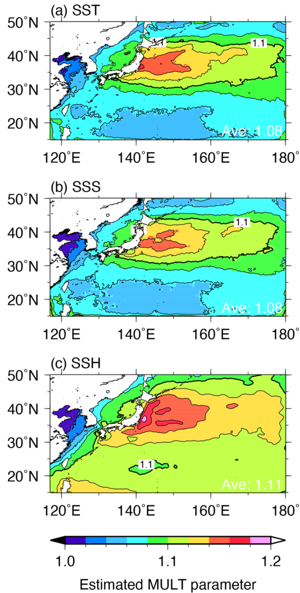
Figure 11: Estimated MULT parameters [Eq. (13)] averaged over 2016 for (a) SST, (b) SSS, and (c) SSH fields using the outputs from the RTPP09+IAU experiment. Right bottom values indicate spatiotemporally averaged estimated MULT parameters. Thin (Thick) counter intervals are 0.02 (0.1).
