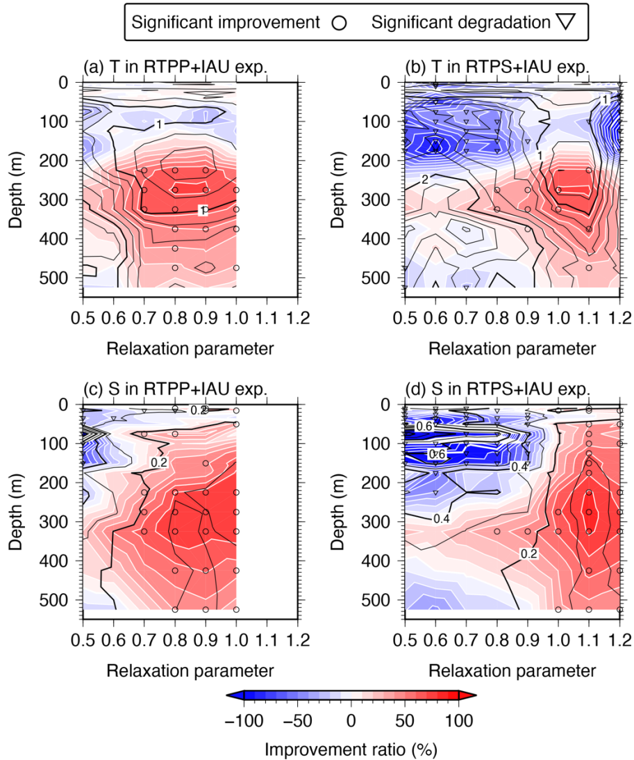
715 Figure 10: Temperature analysis RMSDs (black contours) and IRs (color shading and white contours) between the KEO buoy and (a) RTPP+IAU and (b) RTPS+IAU experiments averaged over 2016. (c) and (d) as in (a) and (b) but for salinity. Open circles and triangles indicate significant improvement and degradation relative to the NO INFL experiment at a 99% confidence level, respectively. Thin (thick) black contour intervals are 0.2 (1.0) °C in (a) and (b), and 0.1 (0.2) in (c) and (d); thin (thick) white contour intervals are 10% (100%).
