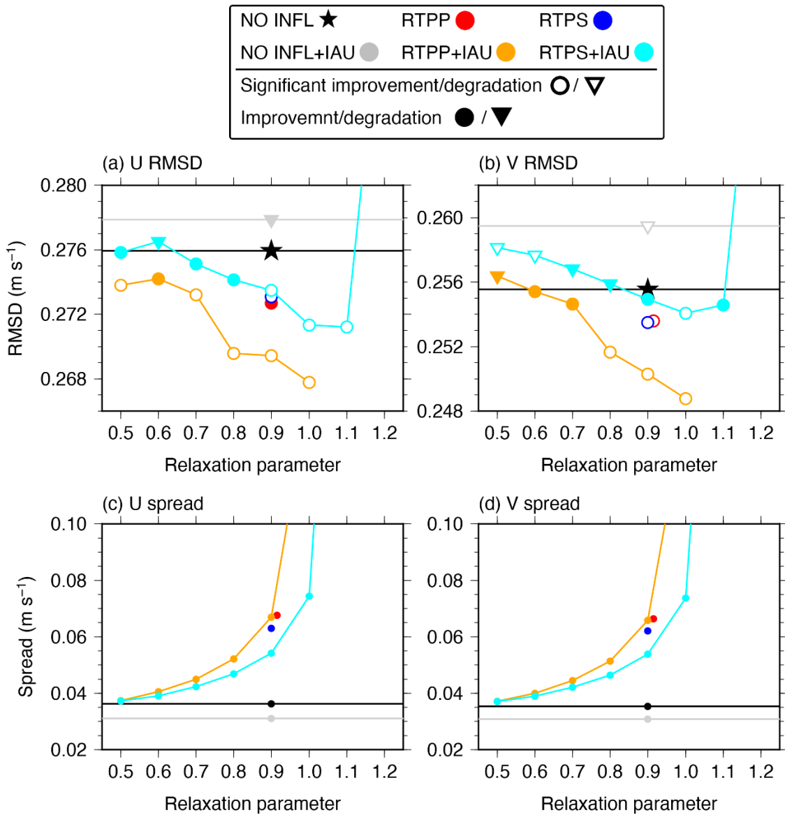
685 Figure 4: As in Fig. 1 but for the analysis RMSDs of the surface (a) zonal and (b) meridional velocity relative to the drifter buoys, and the ensemble spreads of the surface (c) zonal and (d) meridional velocity. The RMSDs of surface zonal and meridional velocity in the RTPS12+IAU experiment are 0.293 and 0.277 \text{m s}^{-1} , respectively (not shown). The RMSD in (b) and ensemble spreads in (c) and (d) in the RTPP09 experiment are slightly offset for visualization.
