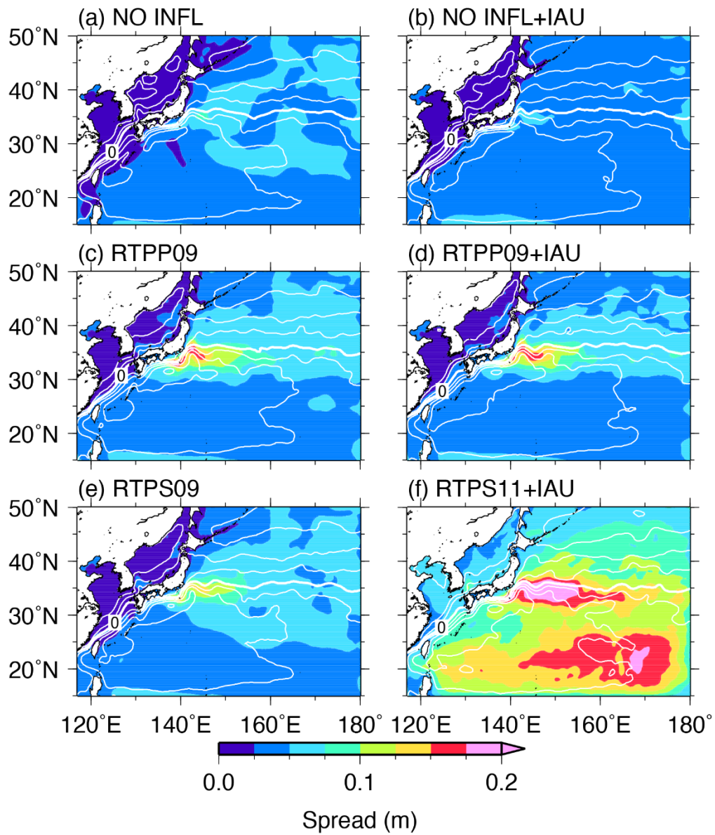
Figure 6: As in Fig. 3 but for the SSHA ensemble spreads.
