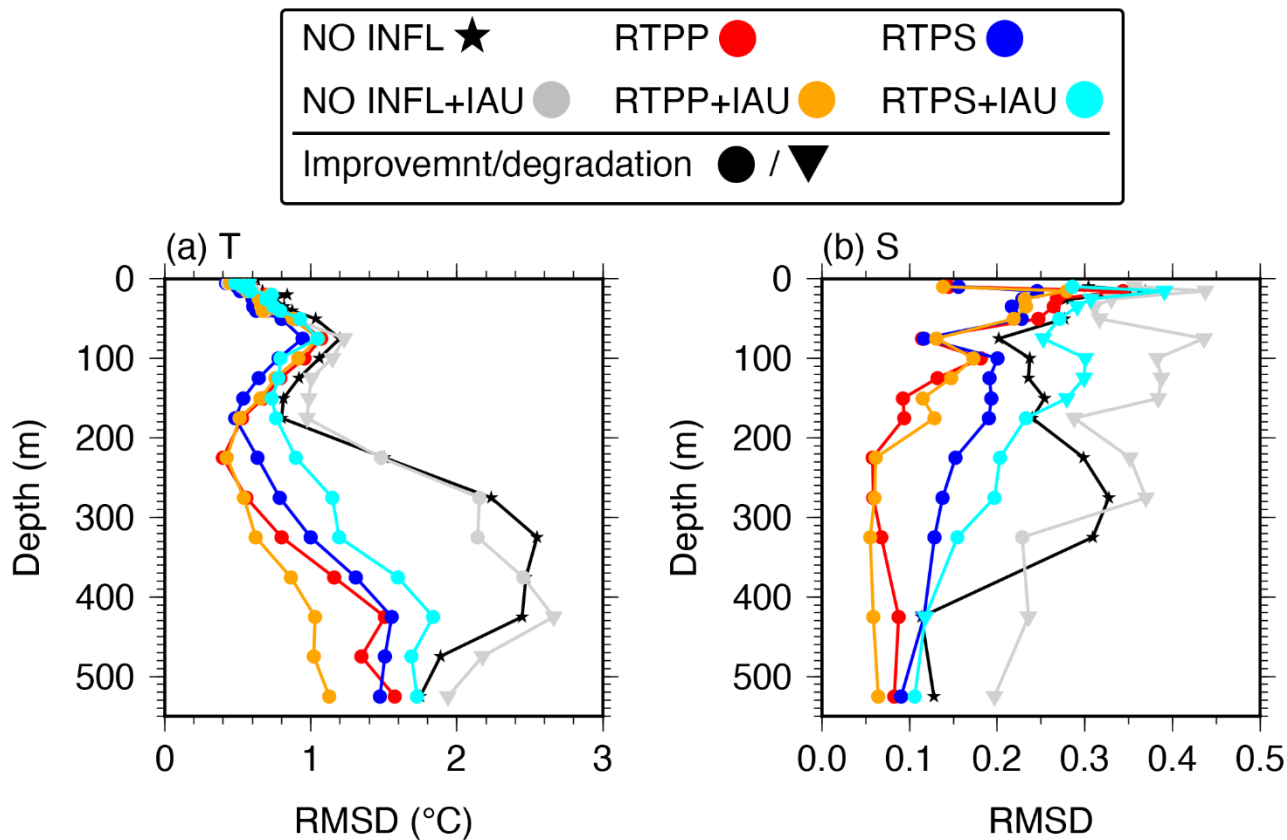
710 Figure 9: As in Fig. 8 but for the forecast RMSDs of the 11-day ensemble forecast experiments. Here, we note that the results of the RTPS09+IAU experiment are shown here, whereas the analysis RMSDs of the RTPS11+IAU experiment are shown in Fig. 8, and thus the relaxation parameters are different in the RTPS+IAU experiments.
