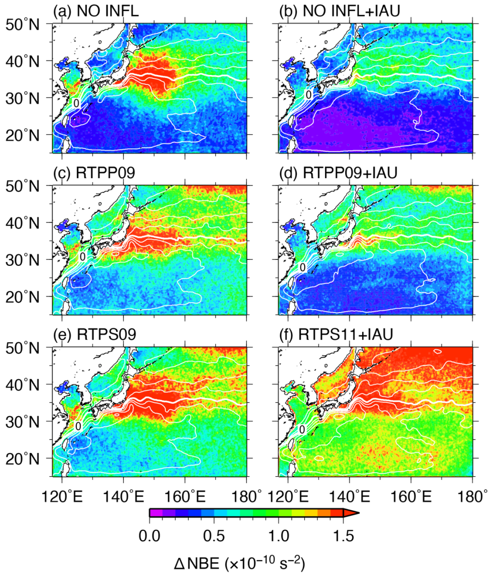
675 Figure 2: \Delta NBE (colors) and SSH (white contours) averaged over 2016 in the (a) NO INFL, (b) NO INFL+IAU, (c) RTPP09, (d) RTPP09+IAU, (e) RTPS09, (f) RTPS11+IAU experiments. Thin (thick) contour intervals are 0.2 m (1.0 m).
