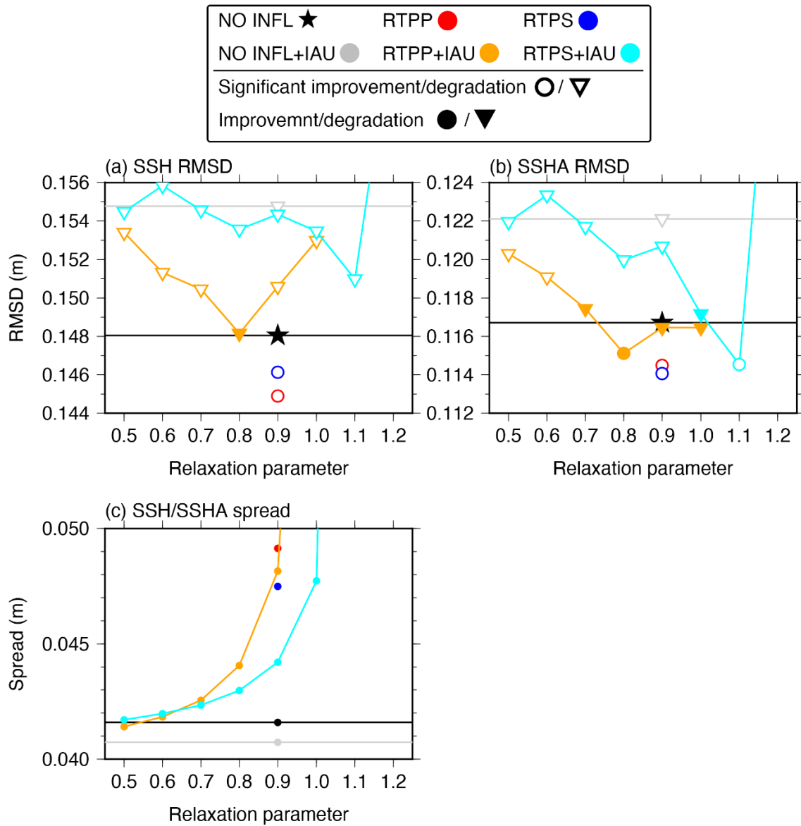
680 Figure 3: As in Fig. 1 but for the analysis RMSDs of (a) SSH and (b) SSHA relative to the AVISO dataset. (c) Spatiotemporally averaged ensemble spreads of SSH and SSHA over the whole domain for 2016 in observational space (circles). The RMSDs of SSH and SSHA in the RTPS12+IAU experiment are 0.164 and 0.137 m, respectively (not shown).
