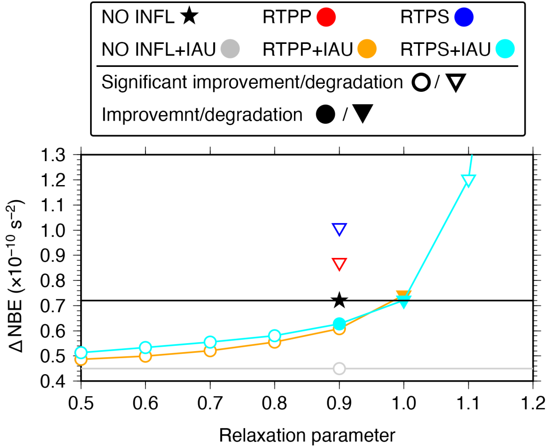
Figure 1: Spatiotemporally averaged \Delta NBE over the whole domain for 2016 in the NO INFL (black star), RTPP (red), 665 RTPS (blue), NO INFL+IAU (gray), RTPP+IAU (orange), and RTPS+IAU (cyan) experiments as a function of the relaxation parameters. Open circles and triangles indicate significant improvement and degradation relative to the NO INFL experiment at a 99% confidence level, respectively, and closed circles and triangles denote improvement and degradation of NO INFL experiment with no significant differences. The RTPS12+IAU, MULT+IAU, and MULT experiments show significant degradation with the averaged \Delta NBE of 2.94 , 2.11 , and 5.22 \times 10^{-10} \text{ s}^{-2} , 670 respectively (not shown). The RTPP+IAU experiments for the relaxation parameters of \alpha_{RTPP} \geq 1.1 are not shown because numerical instability developed.
