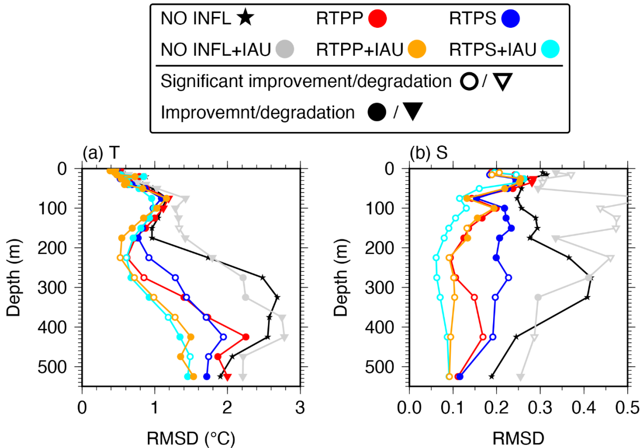
705 Figure 8: Analysis RMSDs of (a) temperature and (b) salinity relative to the KEO buoy averaged over 2016 in the NO INFL (black star), RTPP09 (red), RTPS09 (blue), NO INFL+IAU (gray), RTPP09+IAU (orange), RTPS11+IAU (cyan) experiments. Open circles and triangles denote significant improvement and degradation relative to the NO INFL experiment at a 99% confidence level, respectively. Closed circles and triangles indicate improvement and degradation with no significant differences, respectively.
