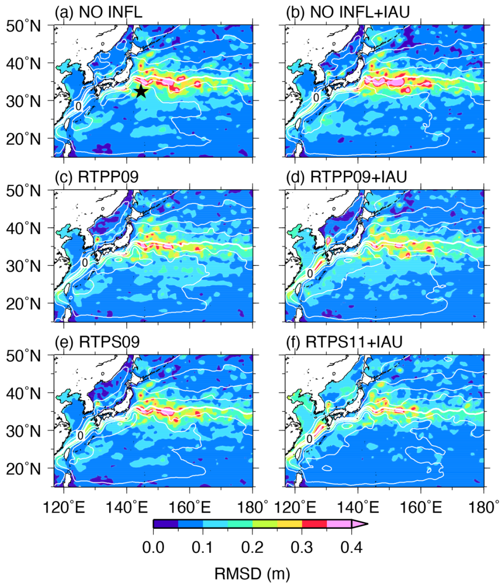
Figure 5: As in Fig. 3 but for the analysis RMSDs relative to the SSHA from the AVISO dataset (color). Black star in 690 (a) indicates the KEO buoy location (144.6°E, 32.3°N).
