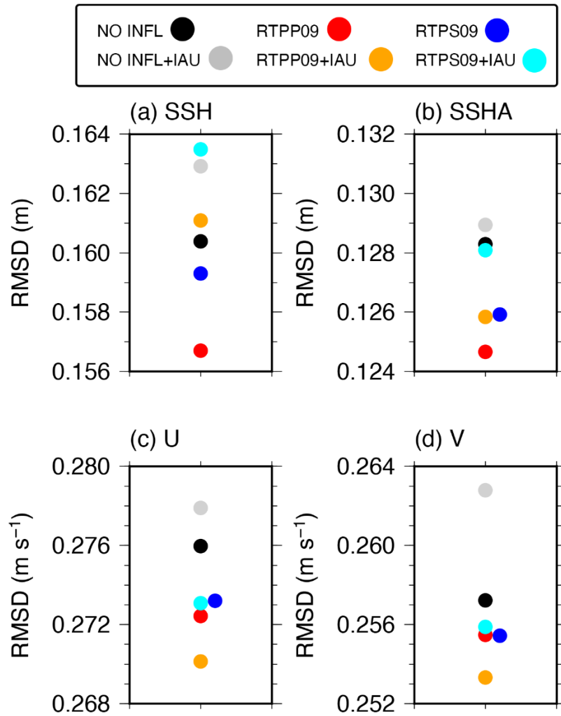
Fig. 7 Spatiotemporally averaged RMSDs of 11-day ensemble forecast in the NO INFL (black), RТПP09 (red), RТПS09 (blue), NO INFL+IAU (gray), RТПP09+IAU (orange), and RТПS09+IAU (cyan) experiments relative to surface (a) SSH and (b) SSHA from the AVISO and (c) zonal and (d) meridional velocities from the drifter buoys.
