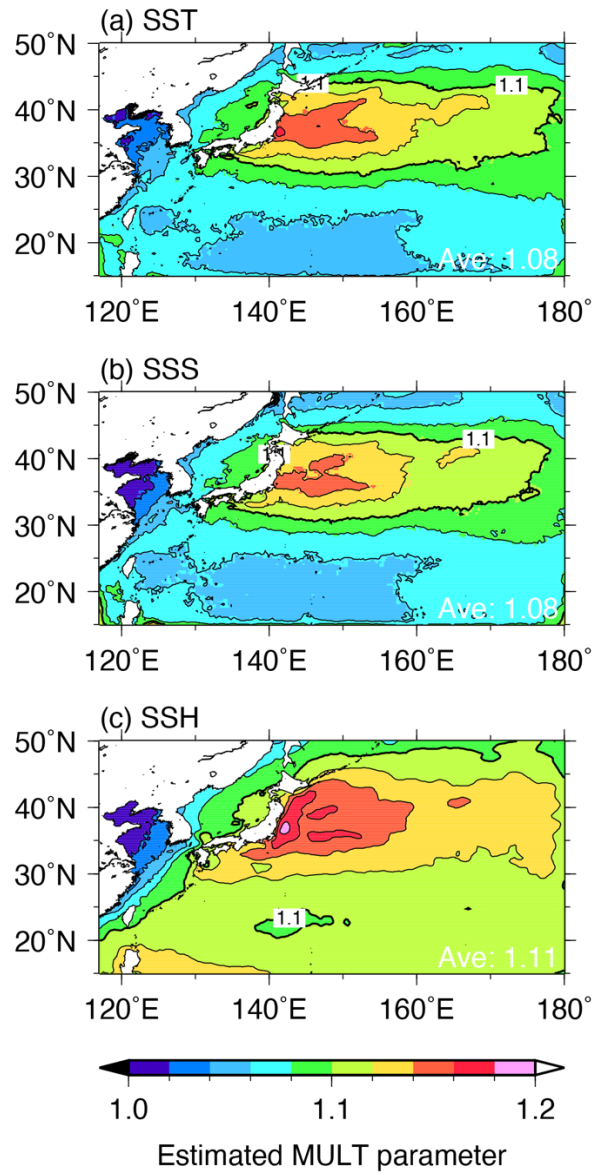
720 Figure 11: Estimated MULT parameters [Eq. (13)] averaged over 2016 for (a) SST, (b) SSS, and (c) SSH fields using the outputs from the RTPP09+IAU experiment. Right bottom values indicate spatiotemporally averaged estimated MULT parameters. Thin (Thick) counter intervals are 0.02 (0.1).
