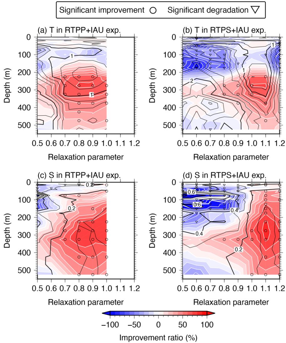
Figure 10: Temperature analysis RMSDs (black contours) and IRs (color shading and white contours) between the KEO buoy and (a) RTPP+IAU and (b) RTPS+IAU experiments averaged over 2016. (c) and (d) as in (a) and (b) but for salinity. Open circles and triangles indicate significant improvement and degradation relative to the NO INFL experiment at a 99% confidence level, respectively. Thin (thick) black contour intervals are 0.2 °C (1.0 °C) in (a) and (b), and 0.1 (0.2) in (c) and (d); thin (thick) white contour intervals are 10% (100%).
