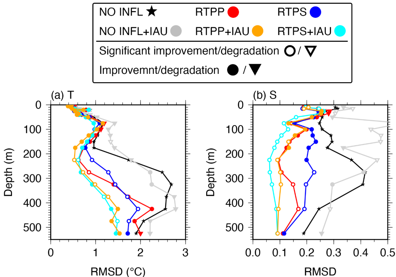
Figure 8: Analysis RMSDs of (a) temperature and (b) salinity relative to the KEO buoy averaged over 2016 in the NO INFL (black star), RTPP09 (red), RTPS09 (blue), NO INFL+IAU (gray), RTPP09+IAU (orange), RTPS11+IAU (cyan) experiments. Open circles and triangles denote significant improvement and degradation relative to the NO INFL experiment at a 99% confidence level, respectively. Closed circles and triangles indicate improvement and degradation with no significant differences, respectively.
