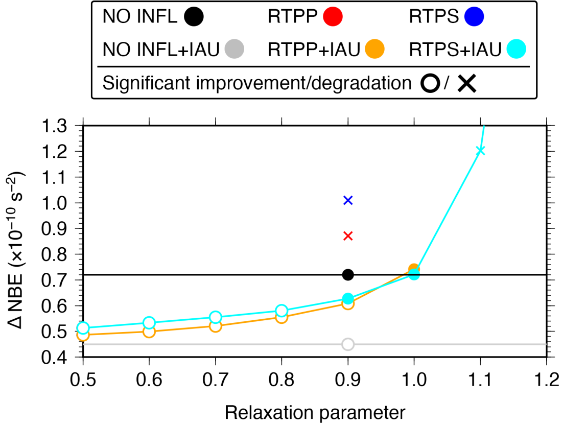
Figure 1: Spatiotemporally averaged \Delta NBE over the whole domain for 2016 in the NO INFL (black), RTPP (red), RTPS (blue), NO INFL+IAU (gray), RTPP+IAU (orange), and RTPS+IAU (cyan) experiments as a function of the relaxation parameters. Open circles and crosses indicate significant improvement and degradation relative to the NO INFL experiment at a 99% confidence level, respectively, and closed circles denote no significant differences. The RTPS12+IAU, MULT+IAU, and MULT experiments show significant degradation with average \Delta NBE of 2.94 , 2.11 , and 5.22 \times 10^{-10} \text{ s}^{-2} , respectively (not shown). The RTPP+IAU experiments for the relaxation parameters of \alpha_{RTPP} \geq 1.1 are not shown because numerical instability developed.
