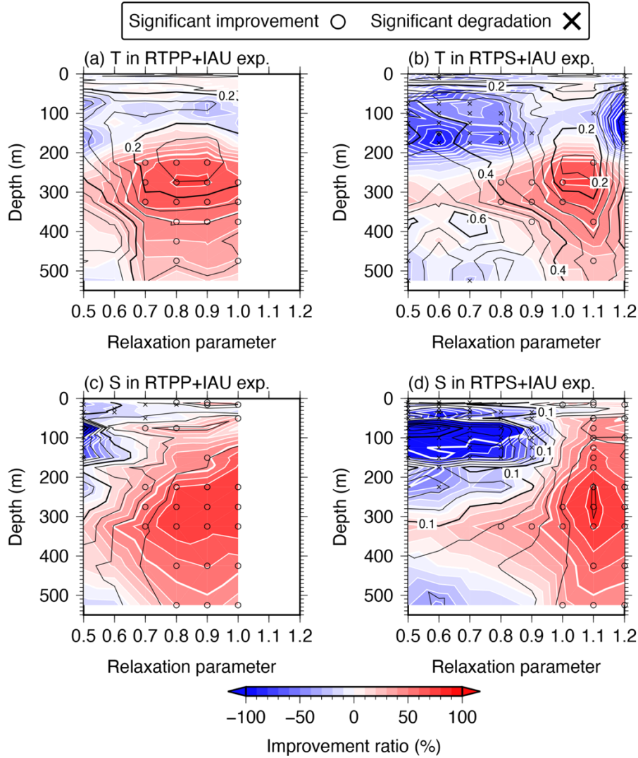
Figure 8: Temperature RMSDs (black contours) and IRs (color shading and white contours) between the KEO buoy and (a) RTTP+IAU and (b) RTPS+IAU experiments averaged over 2016. (c) and (d) as in (a) and (b) but for salinity. Open circles and crosses indicate significant improvement and degradation relative to the NO INFL experiment at a 99% confidence level, respectively. Thin (thick) black contour intervals are 0.05 °C (0.2 °C) in (a) and (b), and 0.02 (0.1) in (c) and (d); thin (thick) white contour intervals are 10% (50%).
