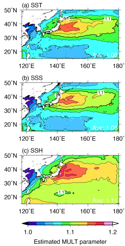
745 Figure 11: Estimated MULT parameters [Eq. (13)] averaged over 2016 for (a) SST, (b) SSS, and (c) SSH fields using the outputs from the RTPP09+IAU experiment. Right bottom values indicate spatiotemporally averaged estimated MULT parameters. Thin (Thick) counter intervals are 0.02 (0.1).
