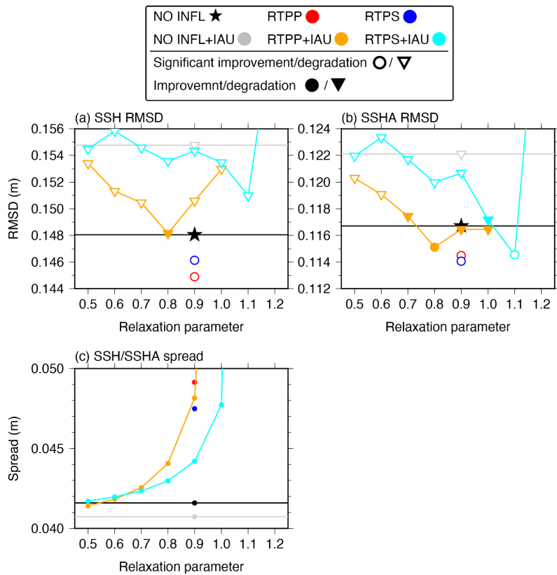
Figure 3: As in Fig. 1 but for the analysis RMSDs of (a) SSH and (b) SSHA relative to the AVISO dataset. (c) Spatiotemporally averaged ensemble spreads of SSH and SSHA over the whole domain for 2016 in observational space (circles). The RMSDs of SSH and SSHA in the RTPS12+IAU experiment are 0.164 and 0.137 m, respectively (not shown).
