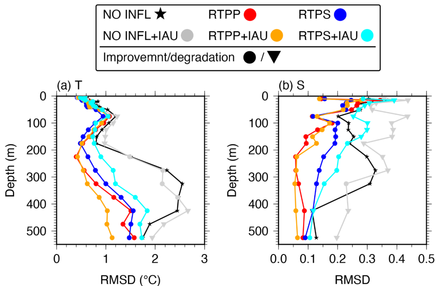
Fig. 9 Same as Fig. 8, but for the RMSDs of the 11-day ensemble forecast experiments. Here, we note that the results of the RTPS09+IAU experiment are shown here, whereas the analysis RMSDs of the RTPS11+IAU experiment are shown in Fig.8, and thus the relaxation parameters are different in the RTPS+IAU experiments.
