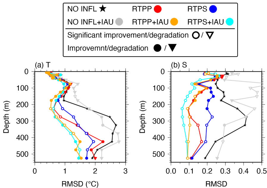
Figure 8: Analysis RMSDs of (a) temperature and (b) salinity relative to the KEO buoy averaged over 2016 in the NO INFL (black star), RTTP09 (red), RTPS09 (blue), NO INFL+IAU (gray), RTTP09+IAU (orange), RTPS11+IAU (cyan) experiments. Open circles and triangles denote significant improvement and degradation relative to the NO INFL experiment at a 99% confidence level, respectively. Closed circles and triangles indicate improvement and degradation with no significant differences, respectively.
