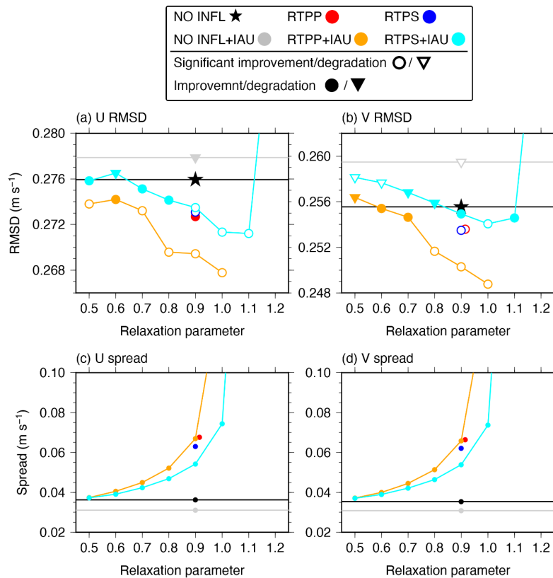
Figure 4: As in Fig. 1 but for the analysis RMSDs of the surface (a) zonal and (b) meridional velocity relative to the drifter buoys, and the ensemble spreads of the surface (c) zonal and (d) meridional velocity. The RMSDs of surface zonal and meridional velocity in the RTPS12+IAU experiment are 0.293 and 0.277 m s -1 , respectively (not shown). 710 The RMSD in (b) and ensemble spreads in (c) and (d) in the RTPP09 experiment are slightly offset for visualization.
