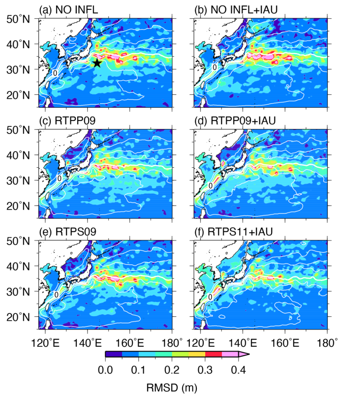
Figure 5: As in Fig. 3, but for the analysis RMSDs relative to the SSHA from the AVISO dataset (color). Black star in (a) indicates the KEO buoy location [144.6°E, 32.3°N].
