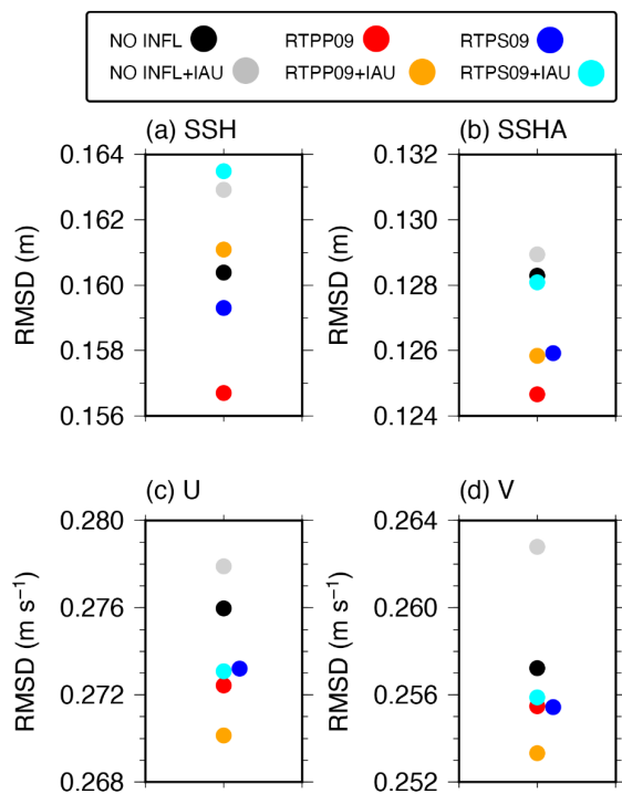
720 Fig. 7 Spatiotemporally averaged RMSDs of 11-day ensemble forecast in the NO INFL (black), RTPP09 (red), RTPS09 (blue), NO INFL+IAU (gray), RTPP09+IAU (orange), and RTPS09+IAU (cyan) experiments relative to surface (a) SSH and (b) SSHA from the AVISO and (c) zonal and (d) meridional velocities from the drifter buoys. The RMSDs in the RTPS09 in (b), (c), and (d) are slightly offset for visualization.
