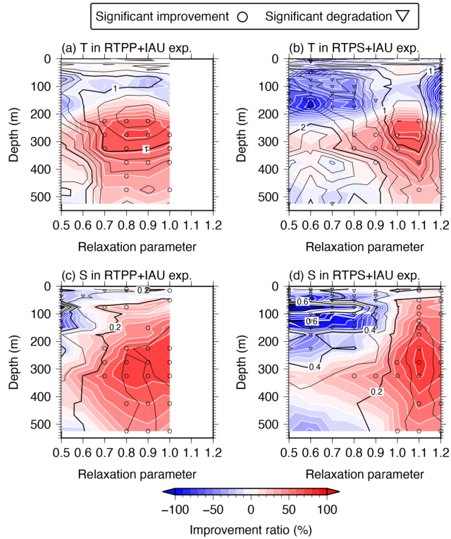
Figure 10: Temperature analysis RMSDs (black contours) and IRs (color shading and white contours) between the KEO buoy and (a) RTTPP+IAU and (b) RTPS+IAU experiments averaged over 2016. (c) and (d) as in (a) and (b) but for salinity. Open circles and triangles indicate significant improvement and degradation relative to the NO INFL experiment at a 99% confidence level, respectively. Thin (thick) black contour intervals are 0.2 °C (1.0 °C) in (a) and (b), and 0.1 (0.2) in (c) and (d); thin (thick) white contour intervals are 10% (100%).
