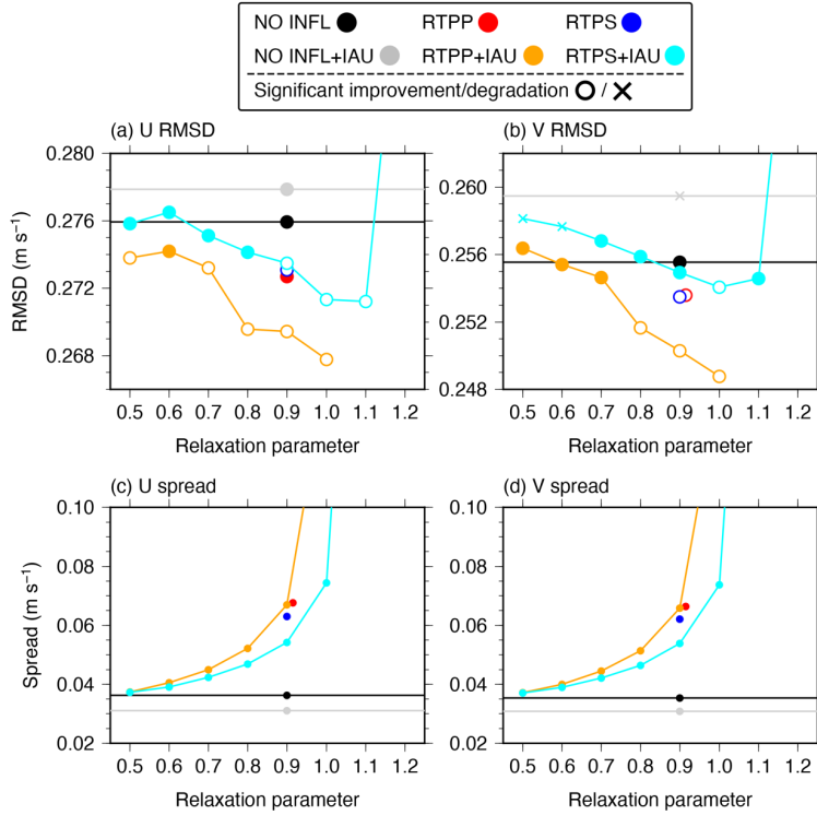
Figure 4: As in Fig. 1 but for the RMSDs of the surface (a) zonal and (b) meridional velocity relative to the drifter 650 buoys, and the ensemble spreads of the surface (c) zonal and (d) meridional velocity. The RMSDs of surface zonal and meridional velocity in the RTPS12+IAU experiment are 0.293 and 0.277 m s -1 , respectively (not shown). The RMSD in (b) and ensemble spreads in (c) and (d) in the RTPP09 experiment are slightly offset for visualization.
