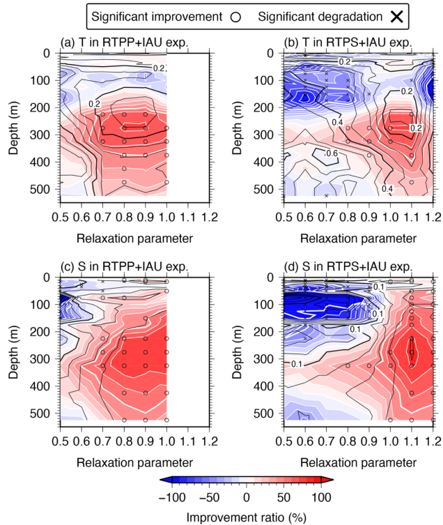
Figure 8: Temperature RMSDs (black contours) and IRs (color shading and white contours) between the KEO buoy and (a) RTPP+IAU and (b) RTPS+IAU experiments averaged over 2016. (c) and (d) as in (a) and (b) but for salinity. Open circles and crosses indicate significant improvement and degradation relative to the NO INFL experiment at a 99% confidence level, respectively. Thin (thick) black contour intervals are 0.05 °C (0.2 °C) in (a) and (b), and 0.02 (0.1) in (c) and (d); thin (thick) white contour intervals are 10% (50%).
