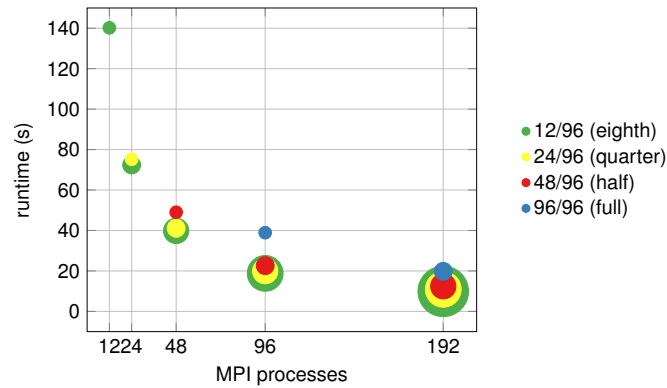
Figure 7. Performance of CUAS-MPI on full (96/96), half (48/96), quarter (24/96), eighth (12/96) populated nodes of Lichtenberg HPC system without file output. The center of the circle shows the number of spawned MPI processes (x-axis) and the runtime (y-axis). For each color the smallest circle indicates the usage of one compute node, the next size up indicates two nodes, the third four nodes, then 8 and lastly 16 nodes.
