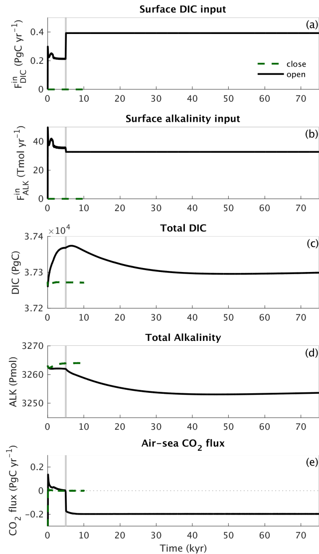
Figure 2. Open versus closed carbon cycle spinup for pre-industrial conditions. The figure shows surface input of (a) DIC and (b) alkalinity, the evolution of (c) DIC and (d) alkalinity inventories in the ocean and (e) the air-sea \text{CO}_2 flux. The grey vertical lines indicate the switch between first and second spinup phase, as described in the text.
