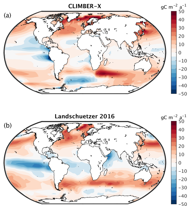
Figure 7. 1985-2010 average air–sea CO 2 flux in (a) CLIMBER-X compared to (b) observations from Landschützer et al. (2016).
