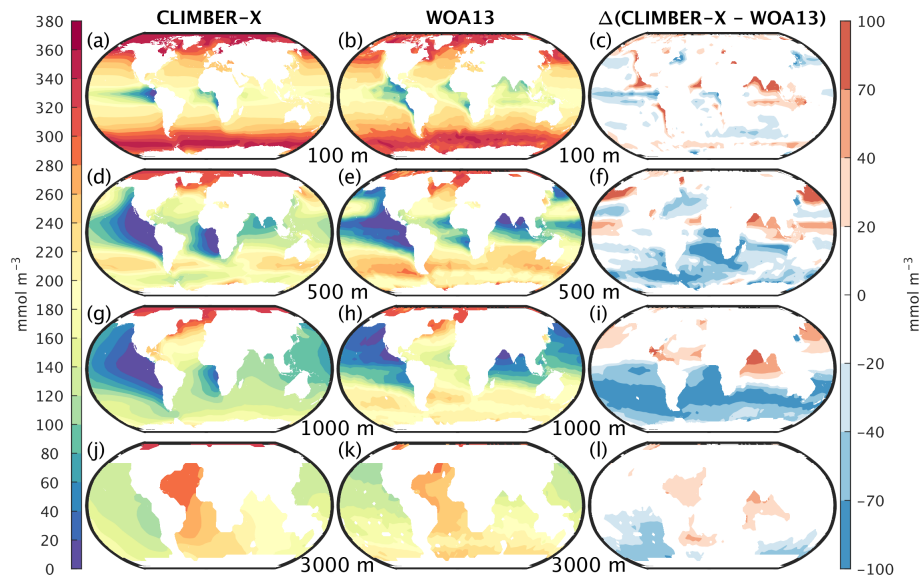
Figure 19. Oxygen concentration in CLIMBER-X, 1981-2010 average, (left column) and WOA13 (Garcia et al., 2013a) (middle column) at different ocean depths: from top to bottom, 100 m, 500 m, 1000 m and 3000 m. The model bias is shown in the right column.
