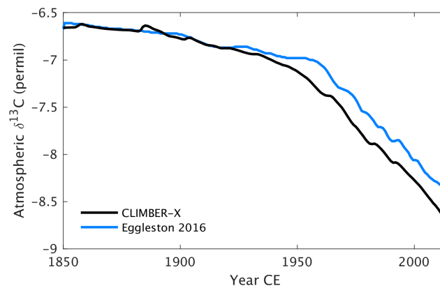
Figure 31. Historical \delta^{13}C of atmospheric CO 2 in CLIMBER-X compared with observations (Eggleston et al., 2016).
