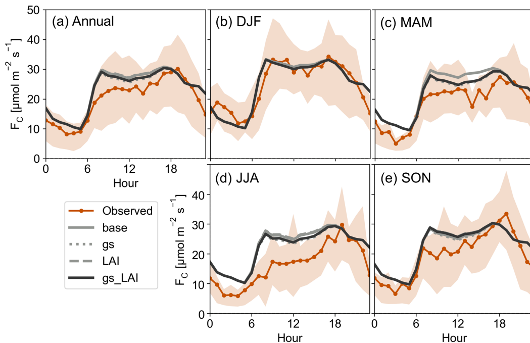
Figure 6. Annual and seasonal average diurnal cycles of observed and modelled \text{CO}_2 flux ( F_C ) for the four model cases (case base , gs , LAI , and gs_LAI ) in the year 2016. The shaded area denotes the interquartile range.
