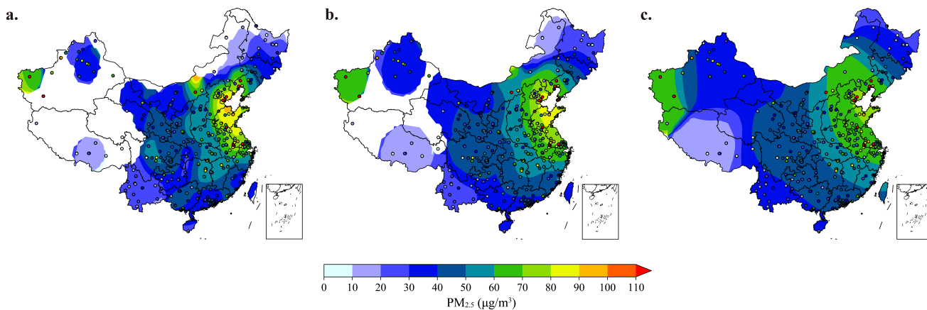
Figure 5. Snapshots of the distribution of the \text{PM}_{2.5} concentration forecasts and observations at at 2019/10/30 16:00:00 (UTC). Panel a, b, and c represent Cressman interpolation of the RFSML (6 h in advance) predictions with a scaling radius of 3^\circ , 5^\circ , and 10^\circ . The colored circles imply the independent observations from 376 ground stations which are not used as source of interpolation.
