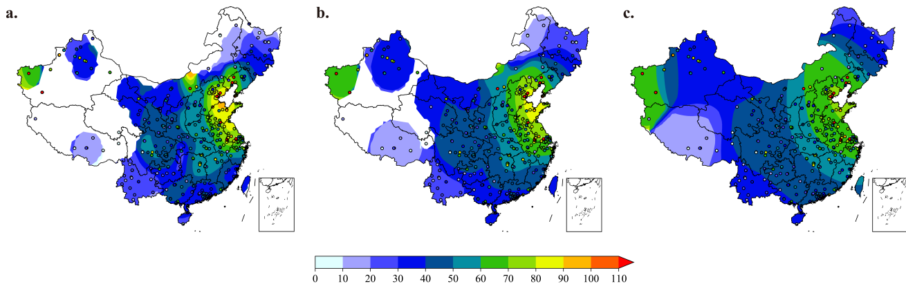
Figure 5. Snapshots of the distribution of the \text{PM}_{2.5} concentration forecasts and observations at at 2019/10/30 16:00:00 (UTC). Panel a, b, and c represent Cressman interpolation of the RFSML (6 h in advance) predictions with a scaling radius of 3^\circ , 5^\circ , and 10^\circ . The colored circles imply the independent observations from 376 ground stations which are not used as source of interpolation.
