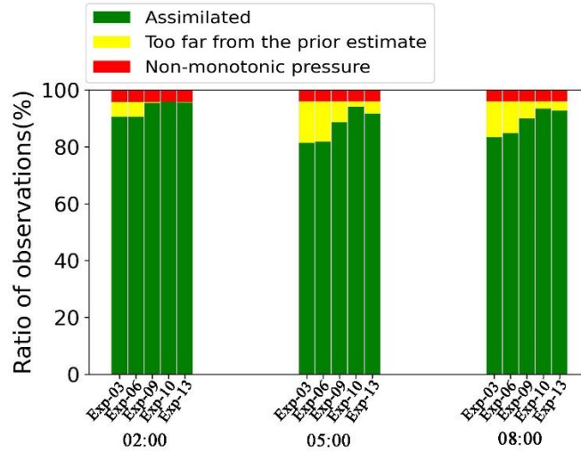
525 Figure 12. The time evolution of the ratio of observations that are assimilated or rejected by the WRF-DART system for different experiment designs with different outlier threshold values and observation errors.
