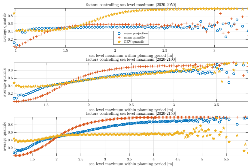
Figure 7. Same as Fig. 6, but with zero probability given to the low confidence versions of SSP2-2.6 and SSP5-8.5.
