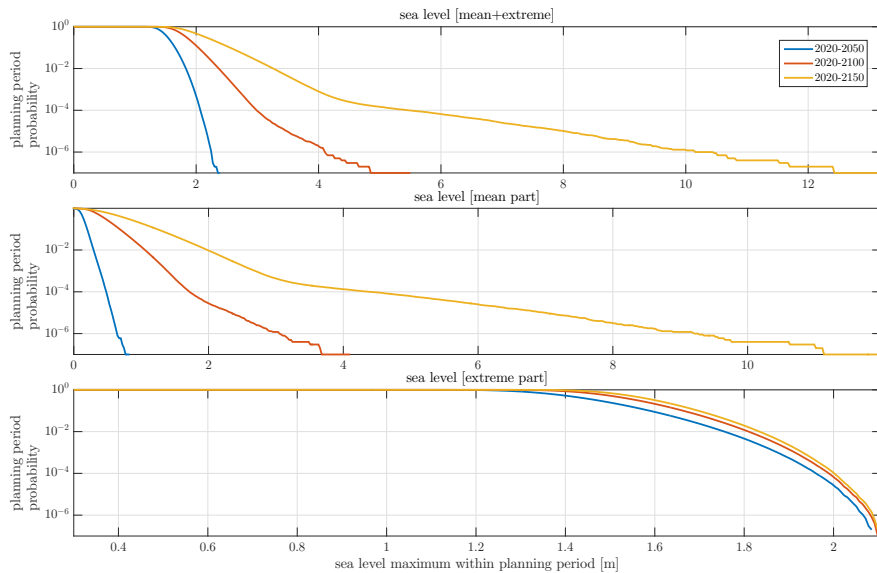
Figure 5. Same as Fig. 3, but with all extremes drawn from the same GEV distribution. That is, all simulated planning periods have their extremes drawn from a GEV distribution that uses the maximum likelihood parameter estimates inferred from the tide gauge data.
