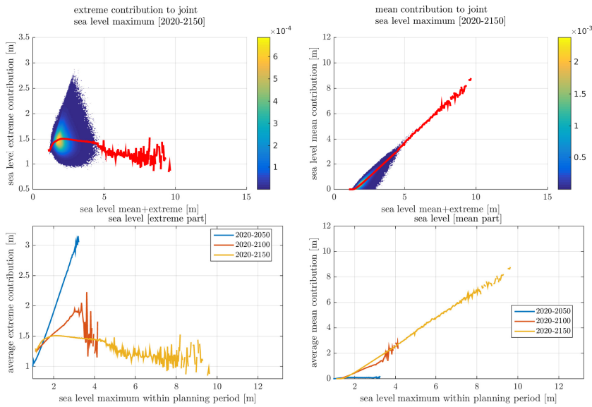
Figure 8. Mean sea level and extreme sea level contributions to joint sea level maximum. Upper panels show relative density [unitless] of the extreme and mean sea level contributions to the joint sea levels. The lower panels show average extreme and mean sea level contributions for different lengths of the planning period. Similarly, the red lines in the upper panels show the average extreme and mean sea level contributions for the 2020-2150 planning period.
