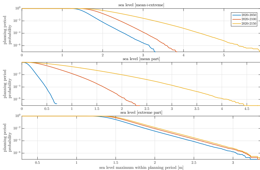
Figure 4. Same as Fig. 3, but with zero probability given to the low confidence versions of SSP2-2.6 and SSP5-8.5.
