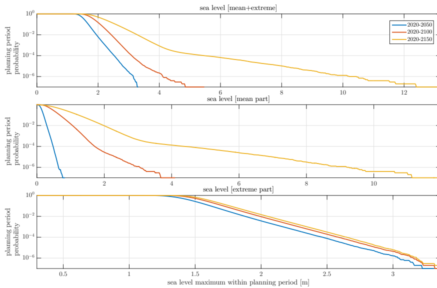
Figure 3. Planing period probability of sea level maximum for three different lengths of the planning period. The top panel shows the joint sea level maximum, the middle the maximum mean sea level and the lower panel the maximum extreme sea level. The figure is derived using the mean sea level projection probabilities given in Tab. 1.
