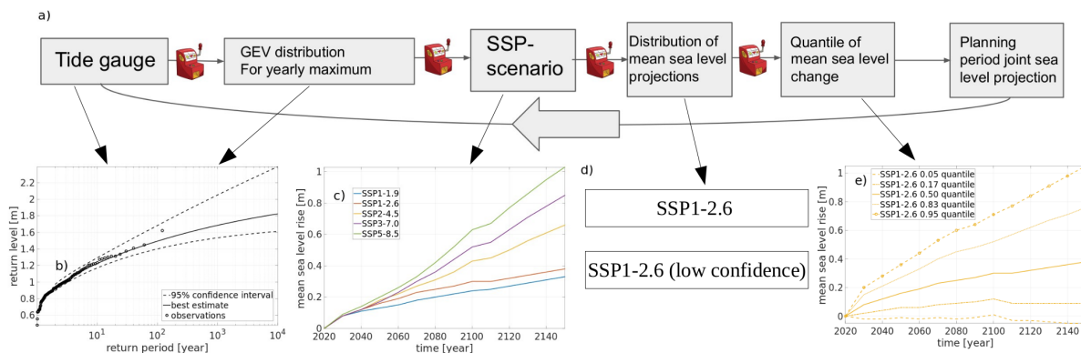
Figure 1. Schematic view of the sea level simulator with insets showing some of the data the simulator depends on. a) shows schematically how a planning period is simulated by going through a chain of modules from left to right. The large arrow below indicates that this cycle is repeated many time (i.e. that many planning periods are simulated). The one armed bandits signify that a stochastic process is involved in going from one module to the next. b) shows the GEV fit and the observed annual maxima, c) shows mean sea level projections for different SSPs, d) indicates that some SSPs have multiple mean sea level projections and e) shows some quantiles of the mean sea level projection for SSP1-2.6.
