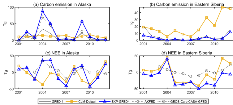
630 Figure 5. Simulated carbon fluxes of CLM-Default and EXP-GFED4 such as carbon emission (a,b), and (c,d) in Alaska (a,c) and Eastern Siberia (b,d) from 2001 to 2012. GFED carbon emission (a,b) and AKFED carbon emission (a) are added to evaluate the performance of carbon emission in CLM-Default and EXP-GFED4 runs. Also, NEE of GEOS-Carb CASA-GFED was added to evaluate the performance of NEE in CLM-Default and EXP-GFED4 runs (c, d).-
