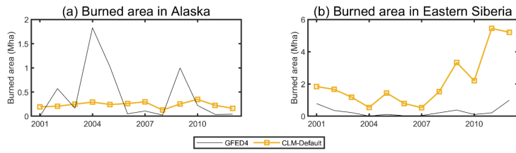
Figure 3. Burned area based on GFED4 and simulated burned area of CLM-Default over (a) Alaska (b) and Eastern Siberia from 2001 to 2012.
