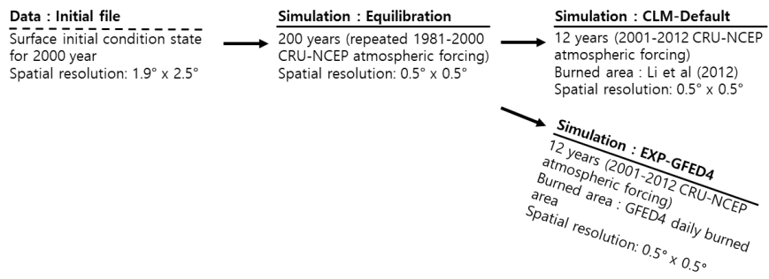
Figure 2. Flow diagram for CLM-Default and EXP-GFED4.
