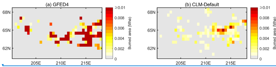
Figure 4. Spatial distribution of burned area of (a) GFED4 (b) and CLM-Default in 2004 over Alaska.
