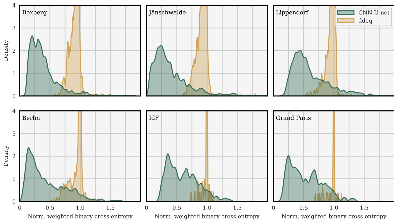
Figure 8. Kernel densities of the histograms of the nwbee-NWBCE scores of the U-net and ddeq segmentation techniques over all images of the various geographical domains.
