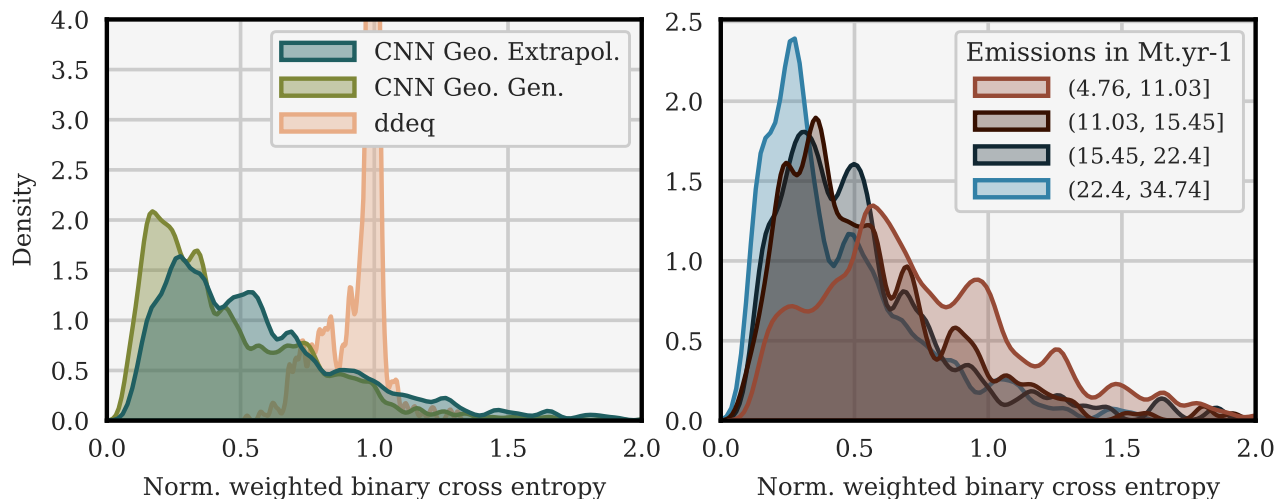
Figure 13. Histograms of the nwbee-NWBCE image scores over all test images of Berlin. Plumes/segmentations are classified depending on the method used (left). In the geographical extrapolation case, the CNN segmentation outputs are classified in four equivalent clusters according to the corresponding emissions (right).
